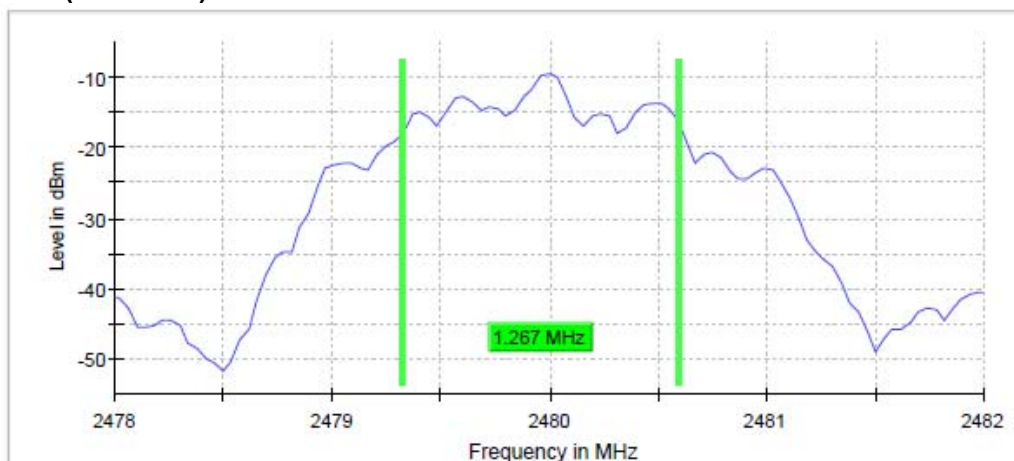
Channel 39 (2480MHz)
