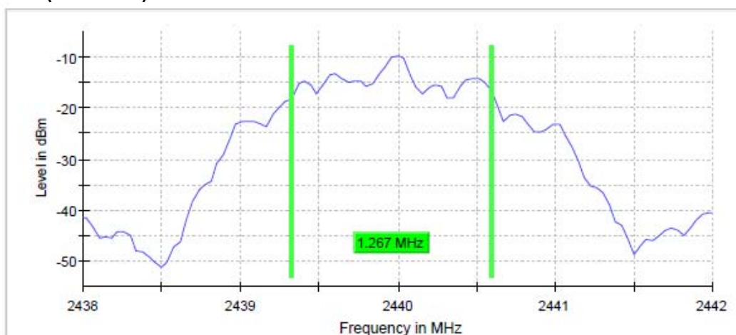
Channel 19 (2440MHz)
