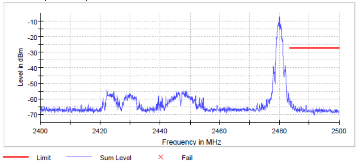
Channel 39 (2480MHz)
