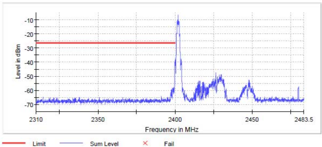
Channel 0 (2402MHz)
