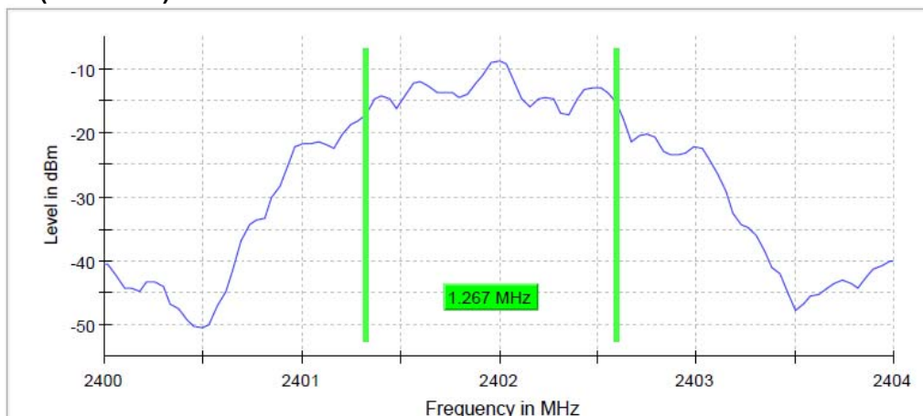
Channel 0 (2402MHz)
