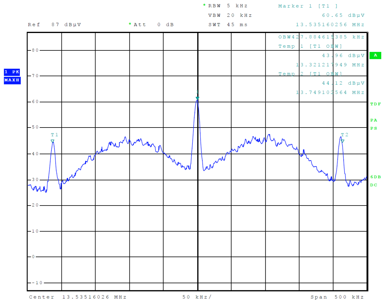
Figure 5 Plot of NFC 99 percent Occupied Bandwidth
