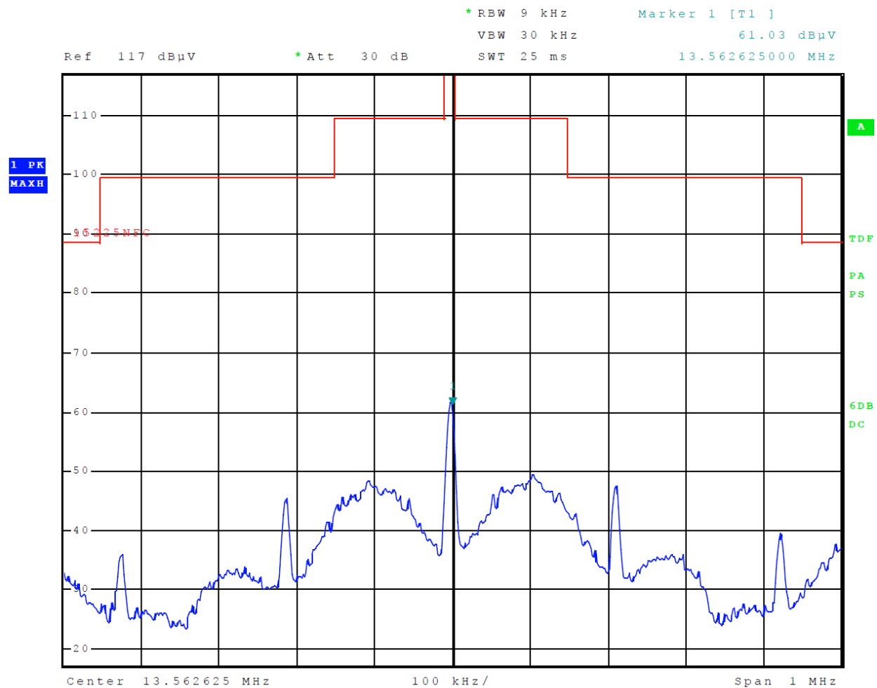
Figure 4 Plot of NFC Operation in Authorized Frequency Band
