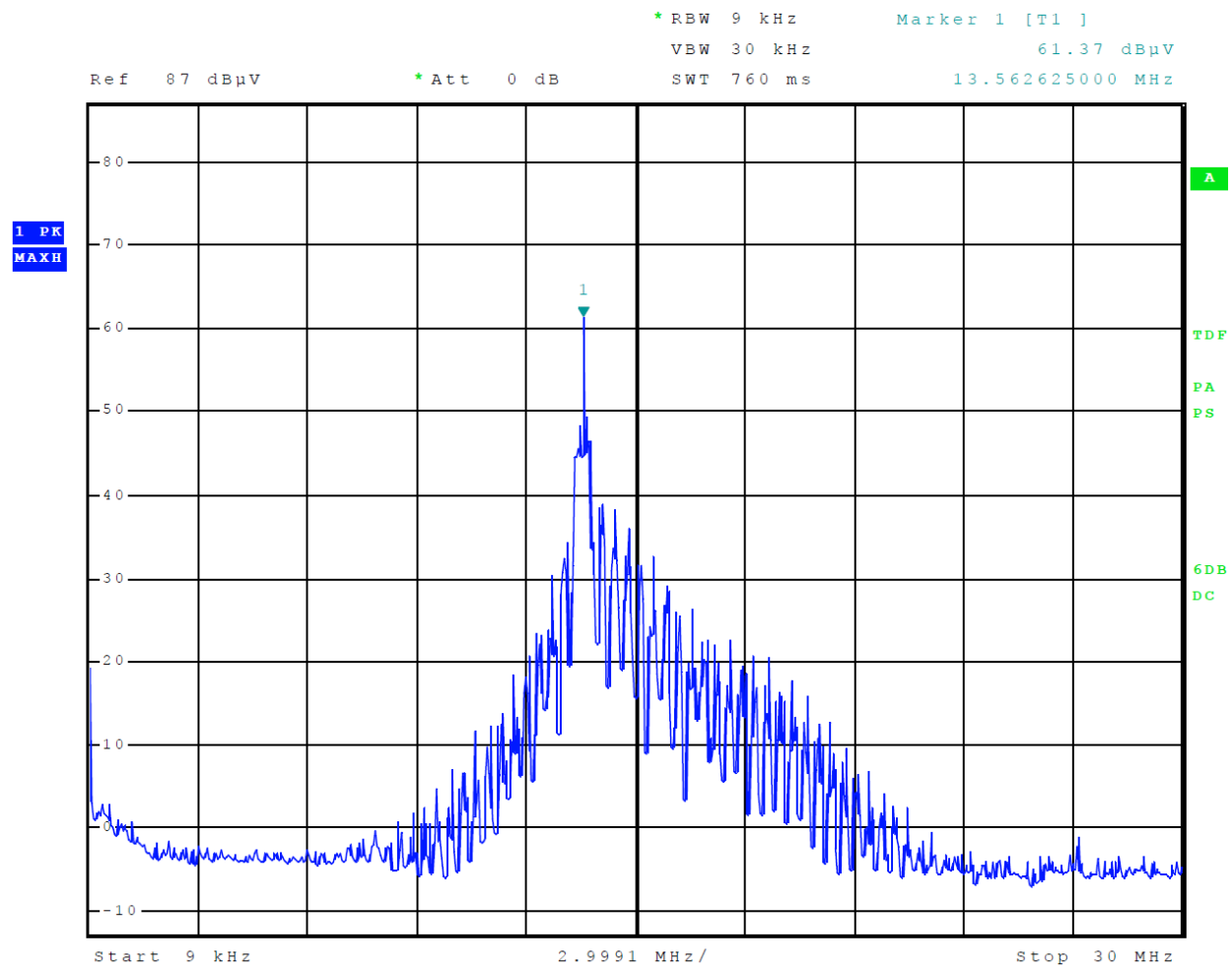
Figure 3 Plot of NFC Operation Across Frequency Spectrum
