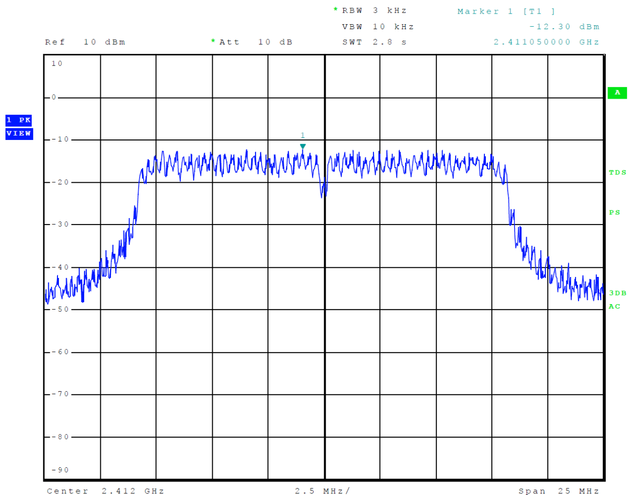
Figure 30 Mode 4 802.11g Plot of Transmitter Power Spectral Density
