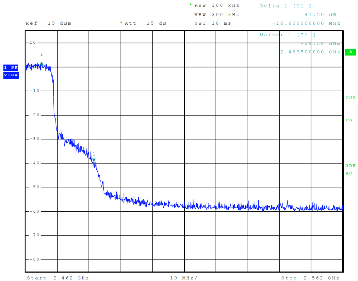
Figure 16 Mode 5 802.11n Plot of Transmitter Emissions High Band Edge
