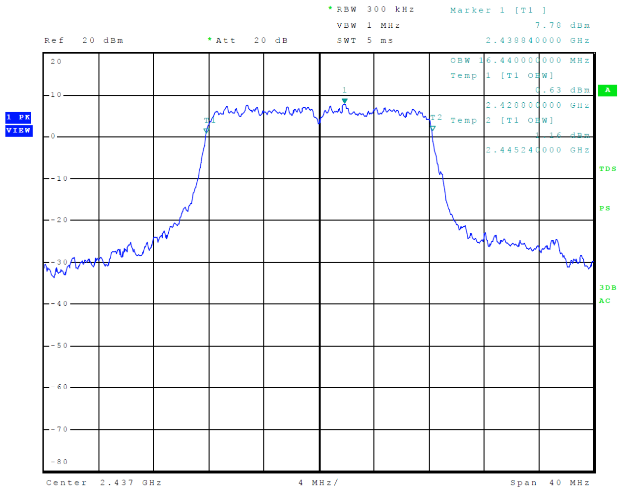
Figure 23 Mode 4 802.11g Plot of 99% Occupied Bandwidth
