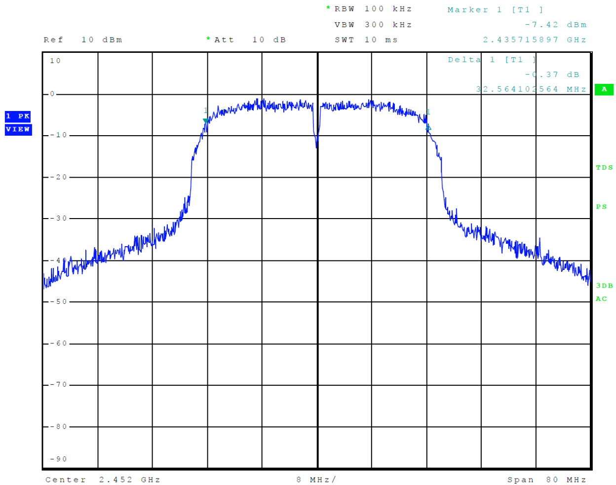
Figure 26 Mode 6 802.11n40 Plot of 6-dB Occupied Bandwidth
