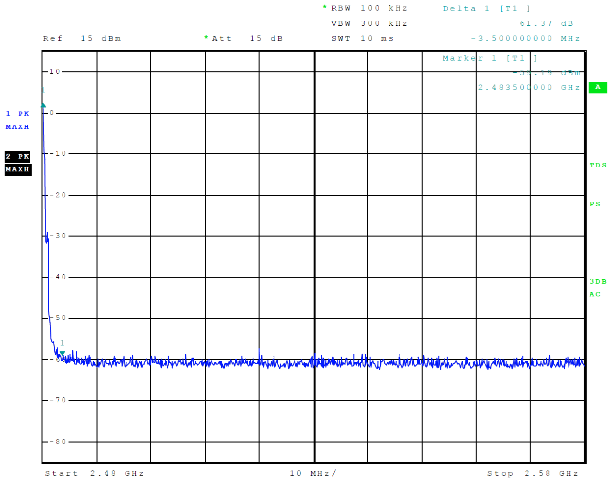
Figure 13 Mode 2 BT BLE Plot of Transmitter Emissions High Band Edge
