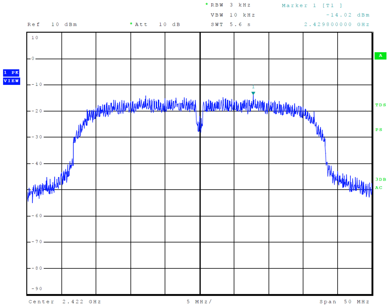
Figure 32 Mode 6 802.11n40 Plot of Transmitter Power Spectral Density
