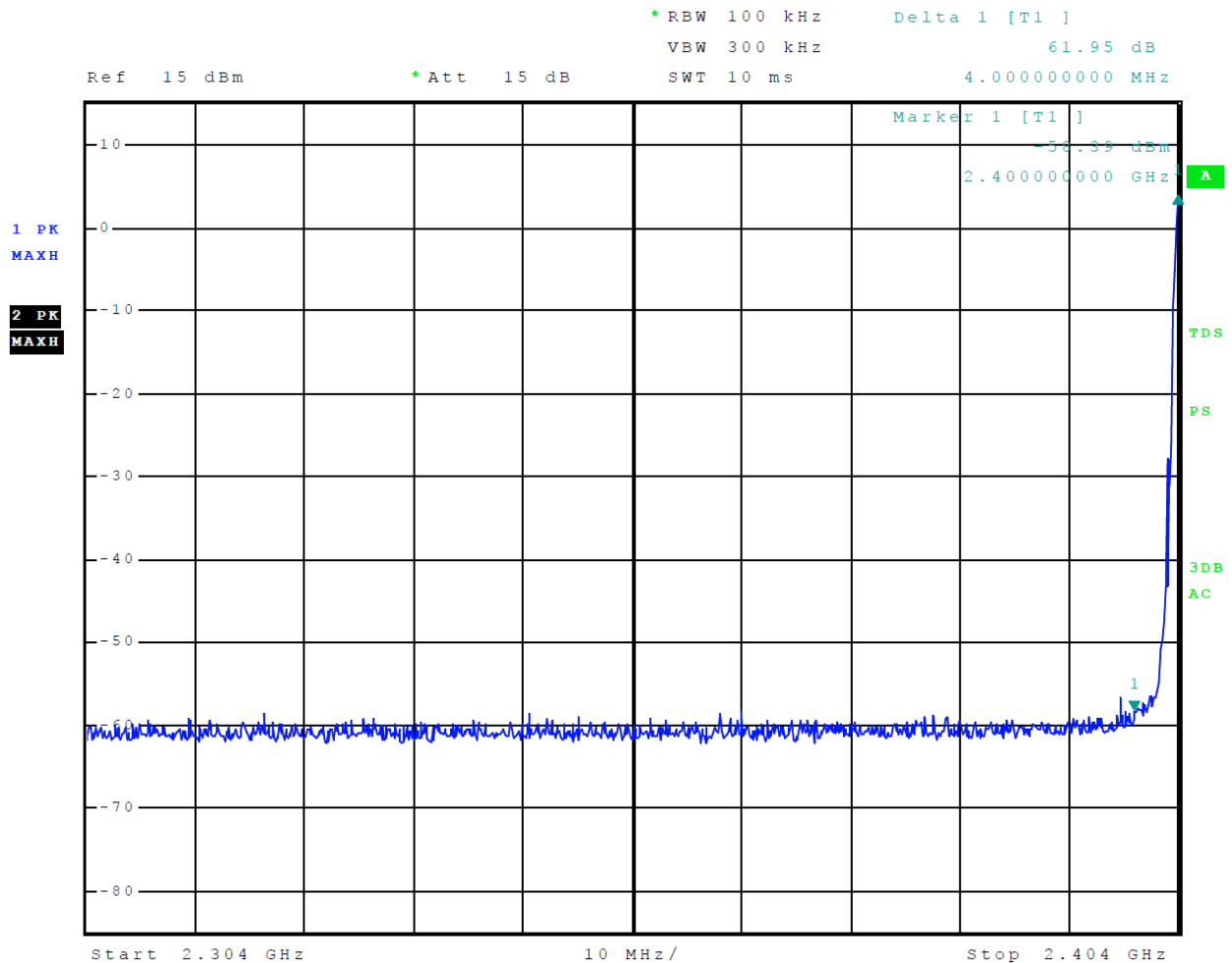
Figure 8 Mode 2 BT BLE Plot of Transmitter Emissions Low Band Edge
