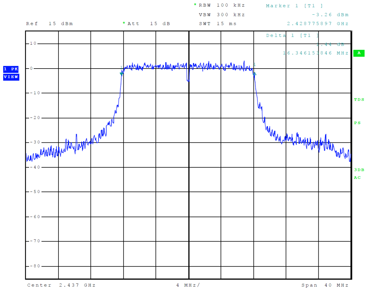
Figure 22 Mode 4 802.11g Plot of 6-dB Occupied Bandwidth
