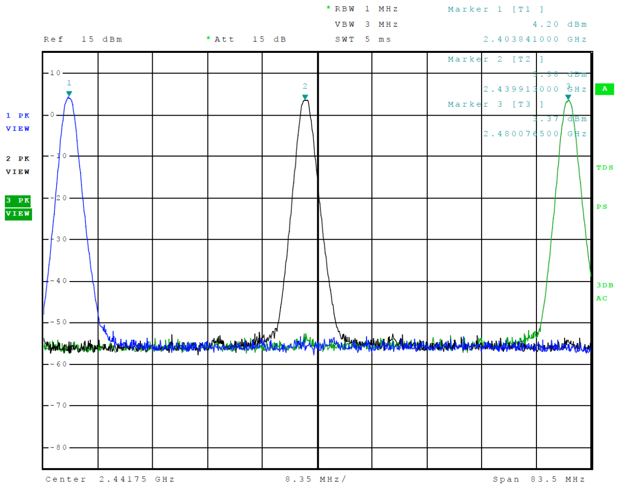
Figure 3 Mode 2 BT BLE Plot of Transmitter Emissions Operation in 2404-2480 MHz
