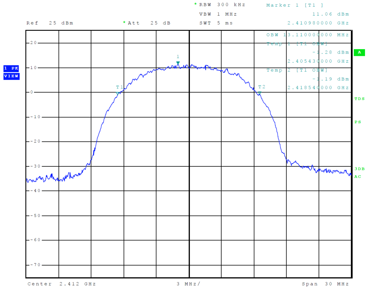
Figure 21 Mode 3 802.11b Plot of 99% Occupied Bandwidth
