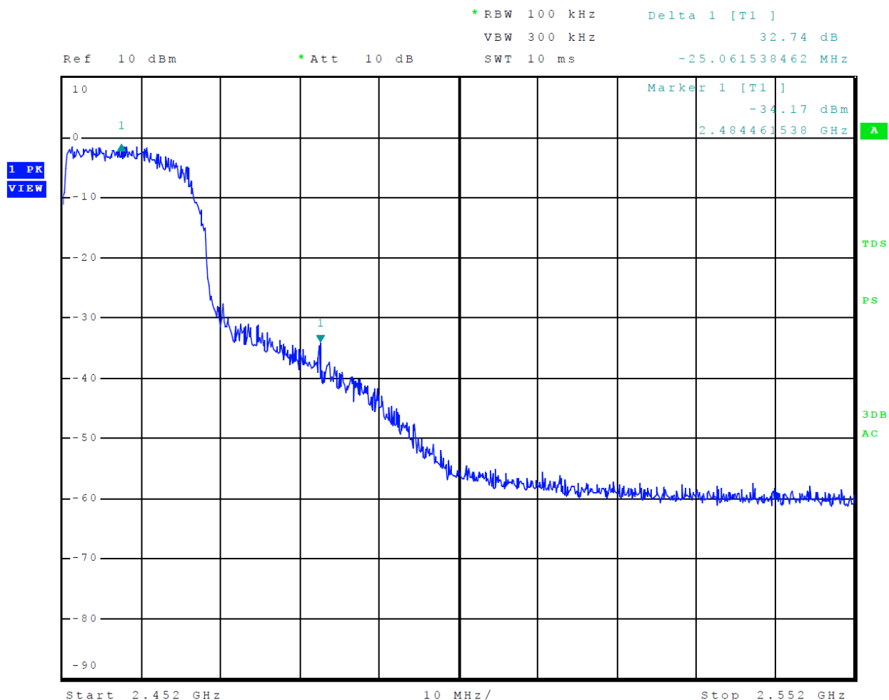
Figure 17 Mode 6 802.11n40 Plot of Transmitter Emissions High Band Edge
