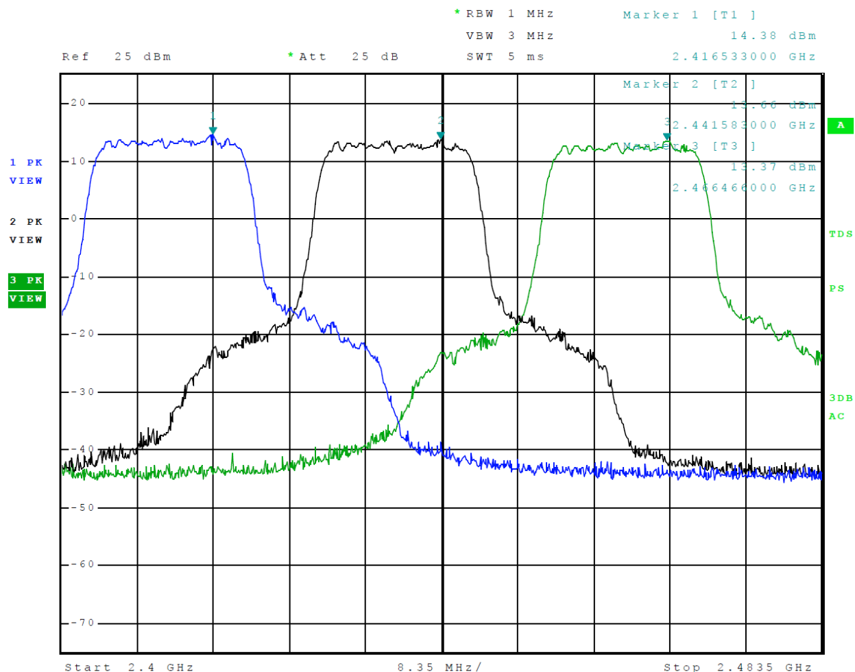
Figure 6 Mode 5 802.11n Plot of Transmitter Operation in 2412-2462 MHz
