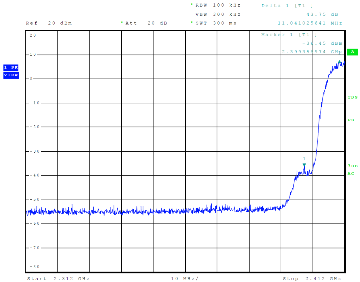
Figure 9 Mode 3 802.11b Plot of Transmitter Emissions Low Band Edge
