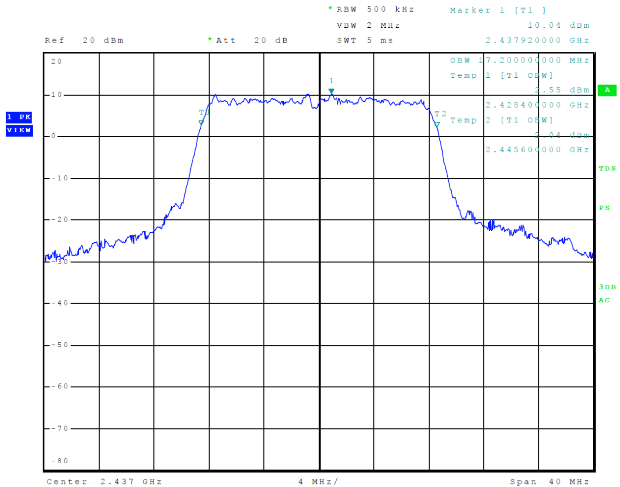
Figure 25 Mode 5 802.11n Plot of 99% Occupied Bandwidth
