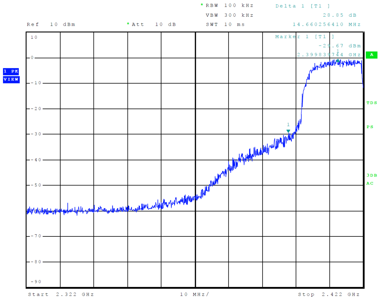
Figure 12 Mode 6 802.11n40 Plot of Transmitter Emissions Low Band Edge
