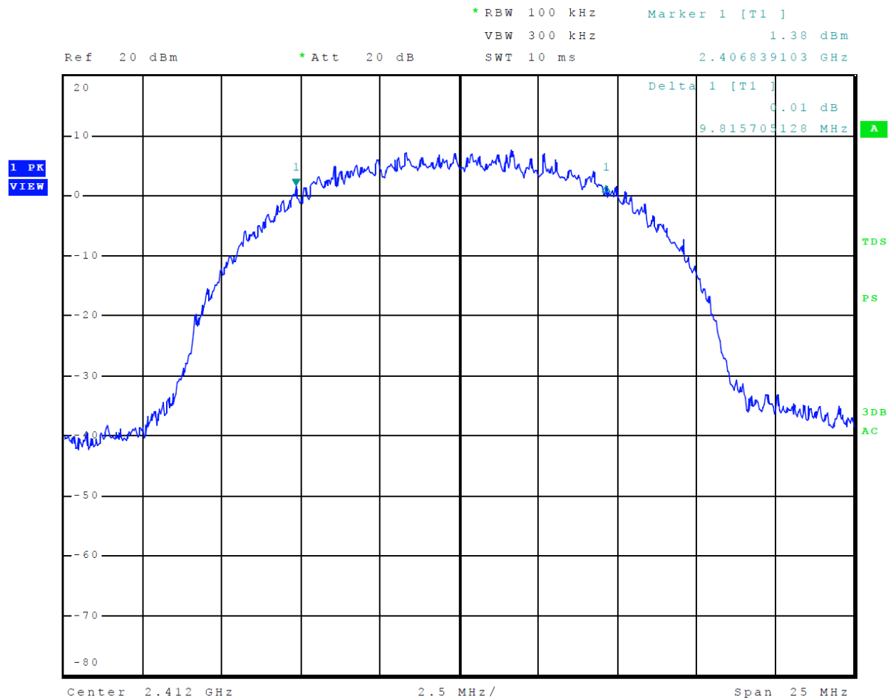
Figure 20 Mode 3 802.11b Plot of 6-dB Occupied Bandwidth
