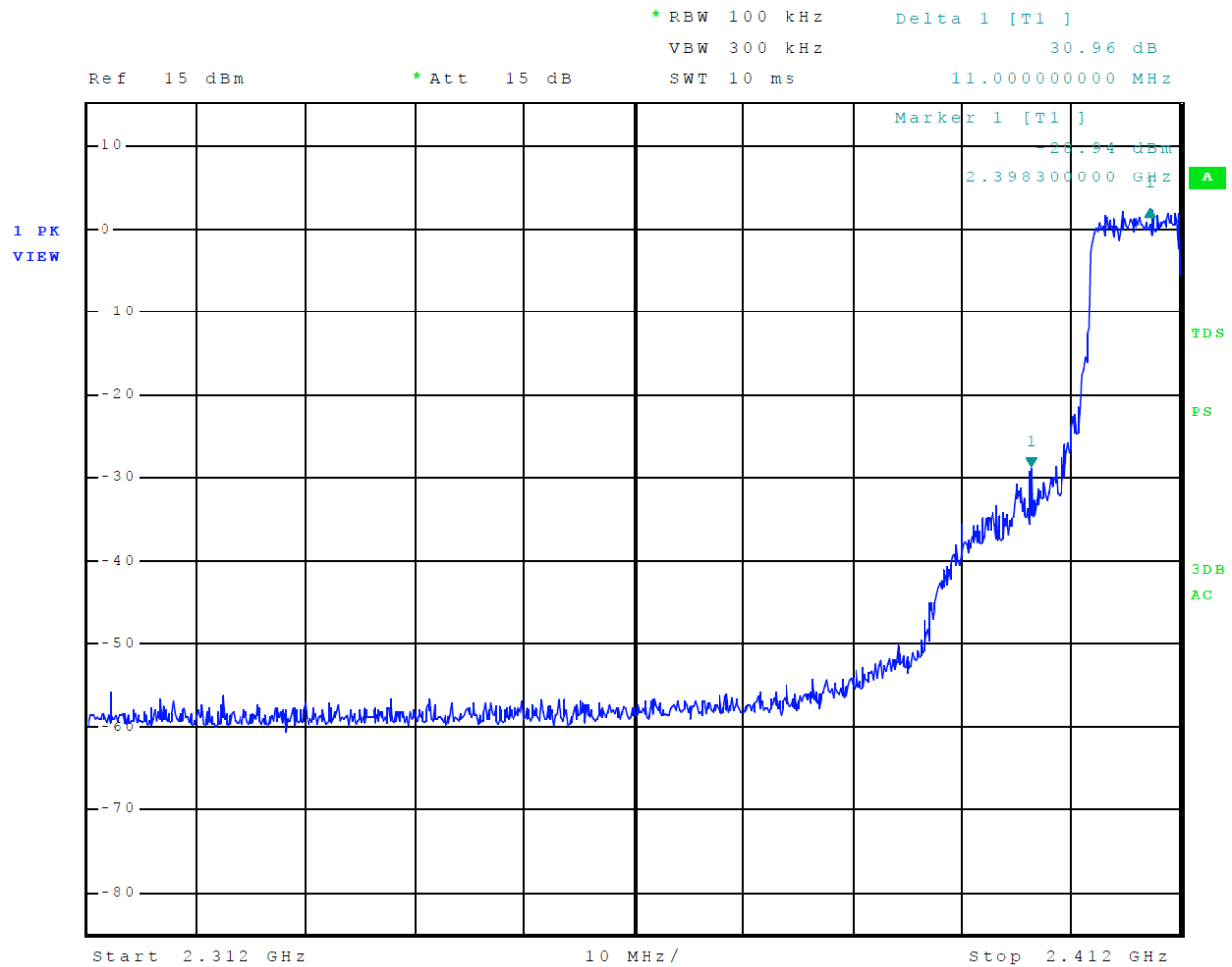
Figure 10 Mode 4 802.11g Plot of Transmitter Emissions Low Band Edge
