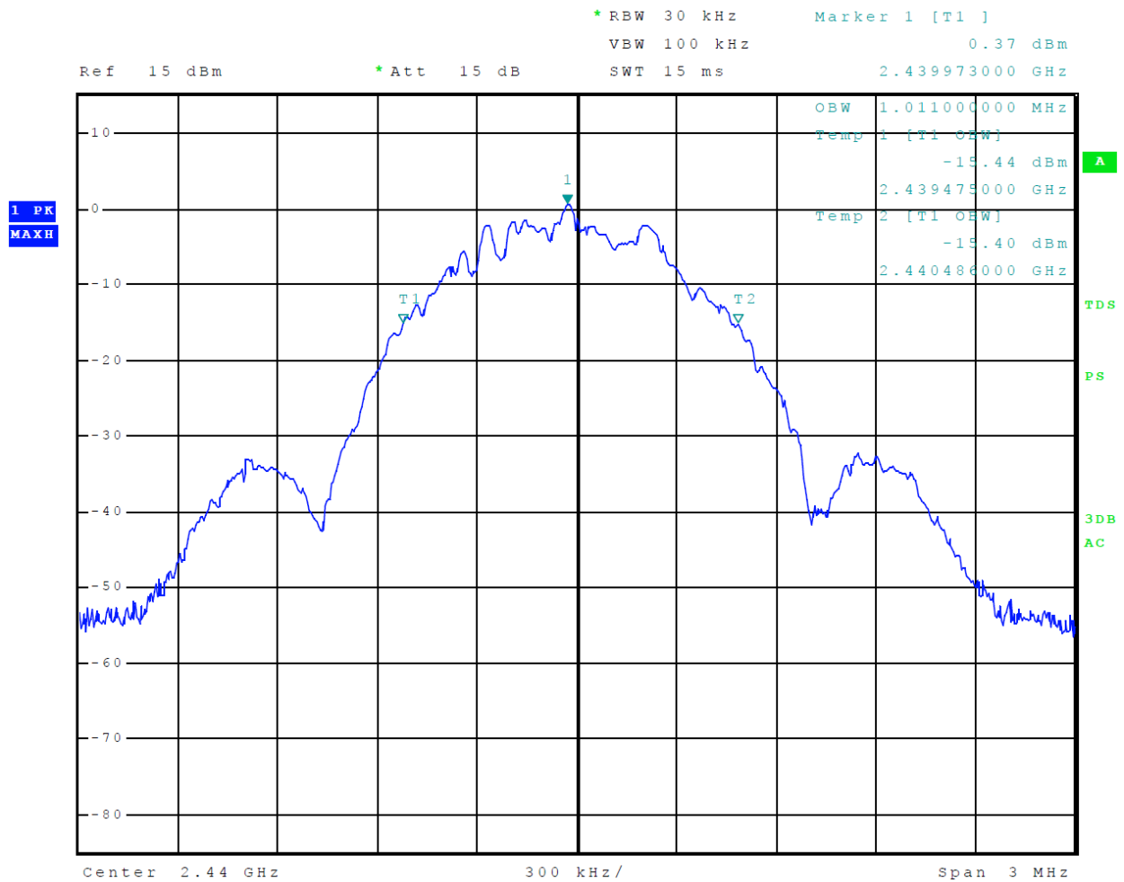
Figure 19 Mode 2 BT BLE Plot of 99% Occupied Bandwidth
