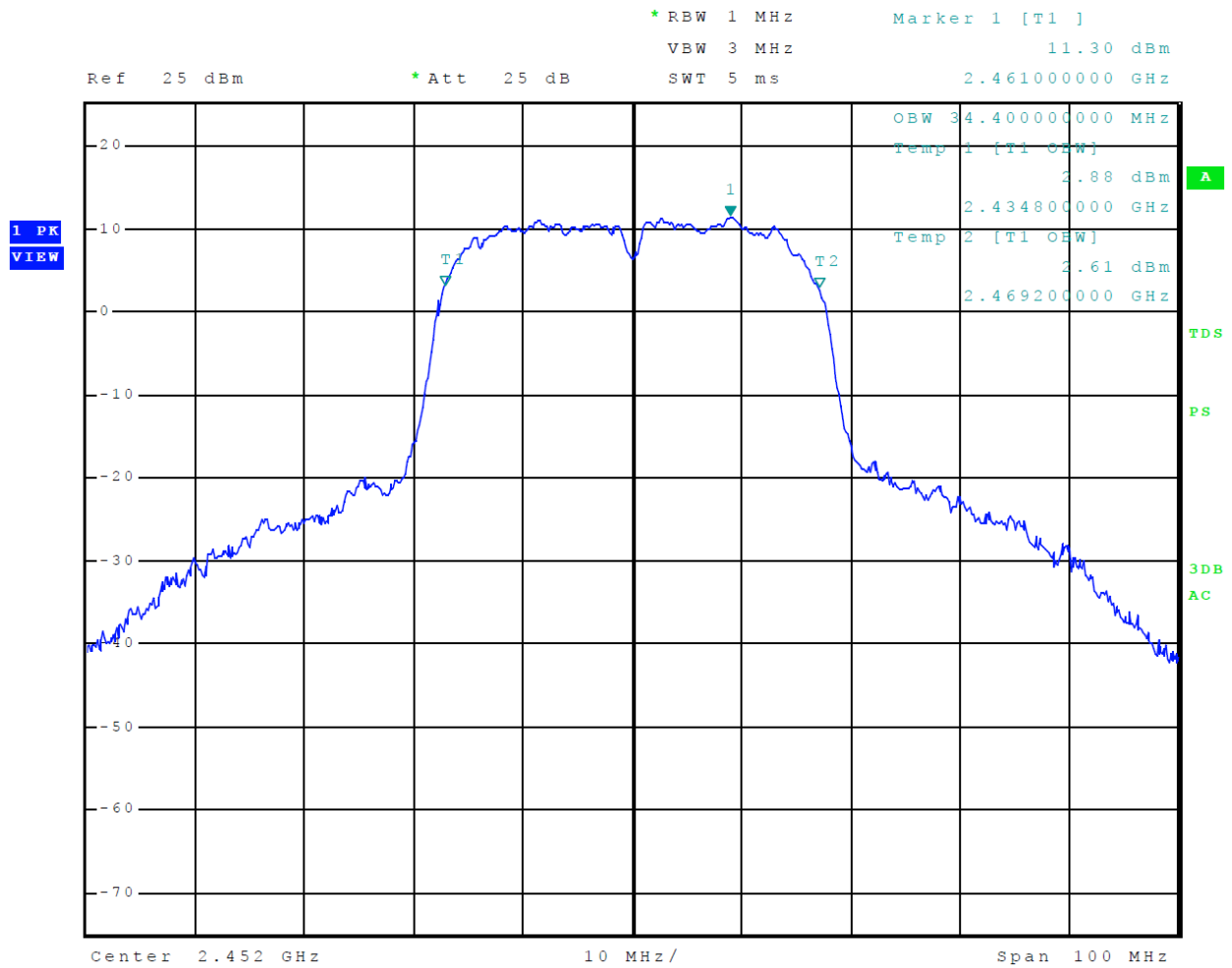
Figure 27 Mode 6 802.11n40 Plot of 99% Occupied Bandwidth
