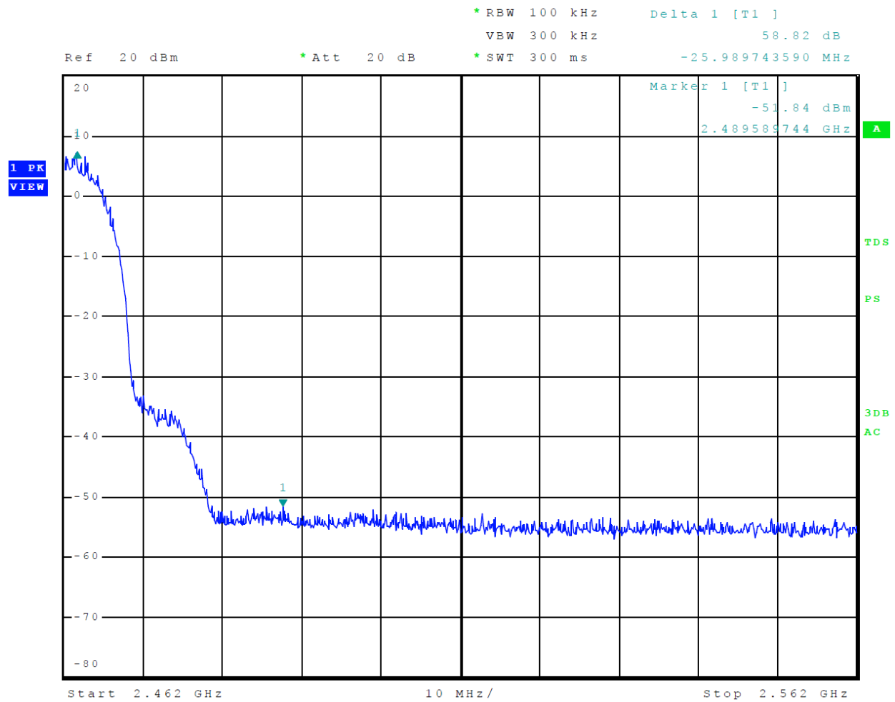
Figure 14 Mode 3 802.11b Plot of Transmitter Emissions High Band Edge
