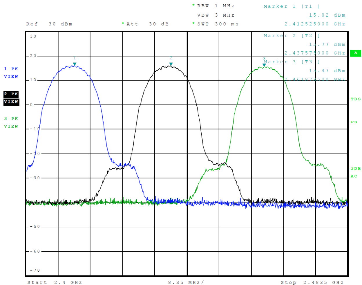
Figure 4 Mode 3 802.11b Plot of Transmitter Operation in 2412-2462 MHz
