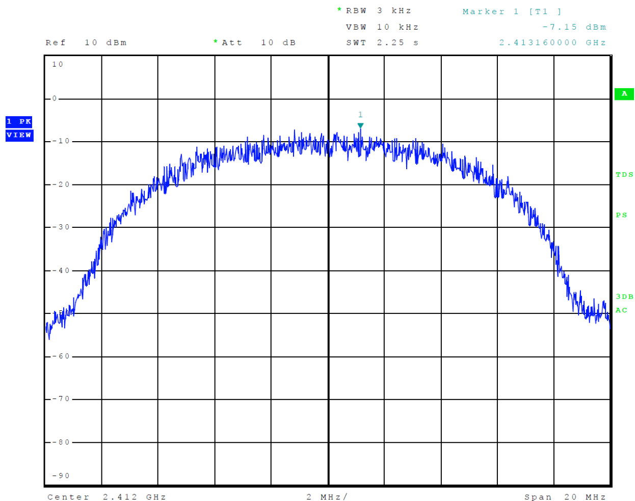
Figure 29 Mode 3 802.11b Plot of Transmitter Power Spectral Density
