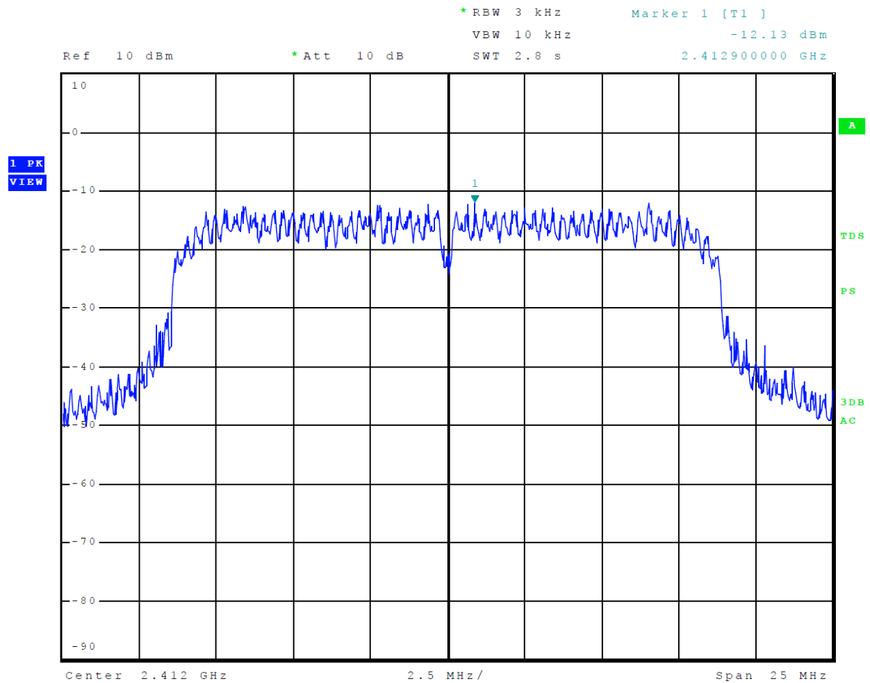
Figure 31 Mode 5 802.11n Plot of Transmitter Power Spectral Density
