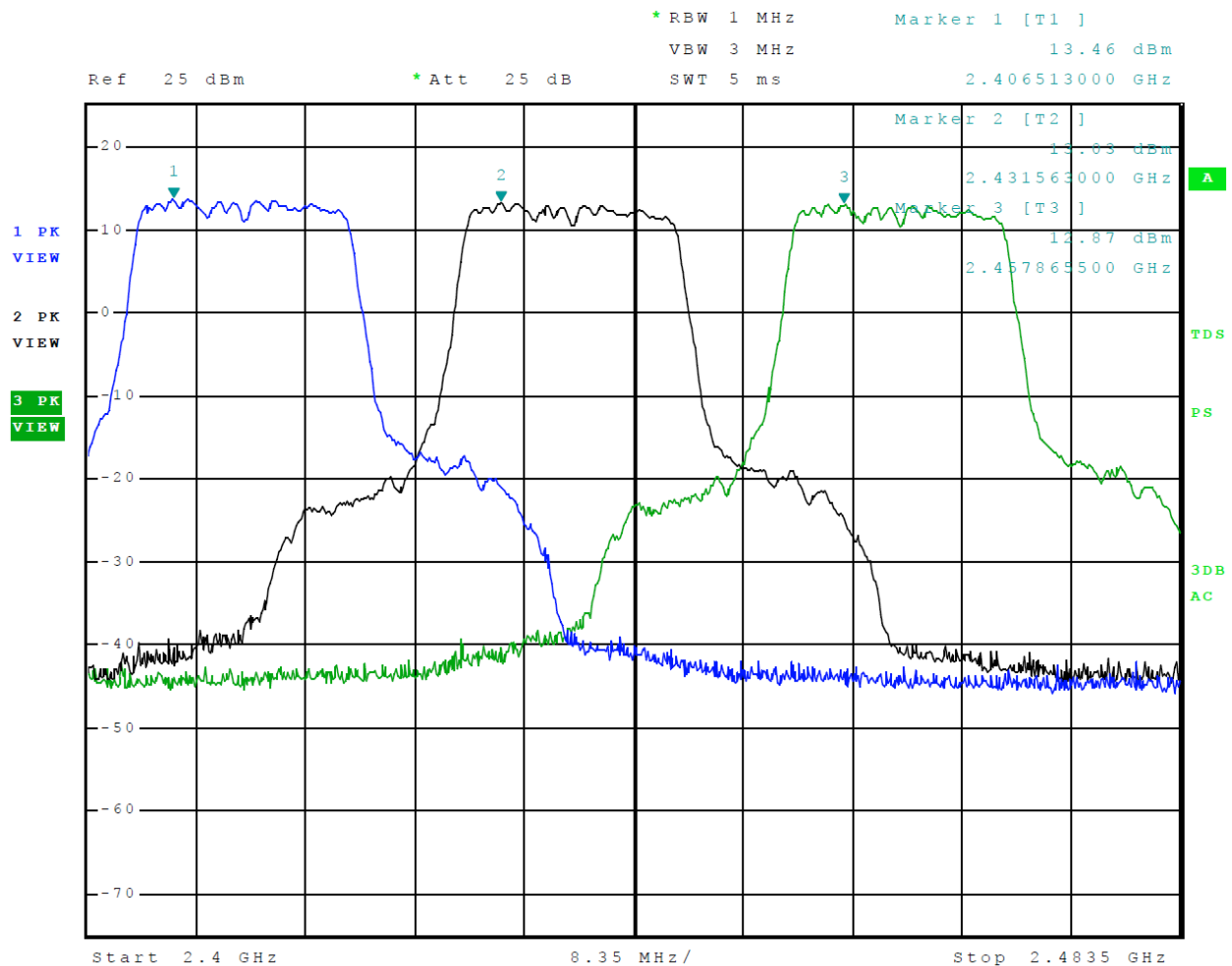
Figure 5 Mode 4 802.11g Plot of Transmitter Operation in 2412-2462 MHz
