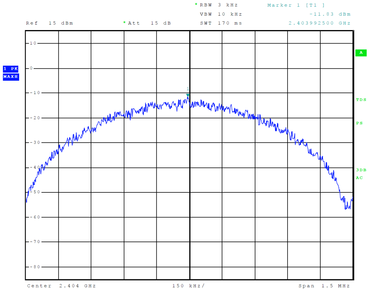
Figure 28 Mode 2 BT BLE Plot of Transmitter Power Spectral Density
