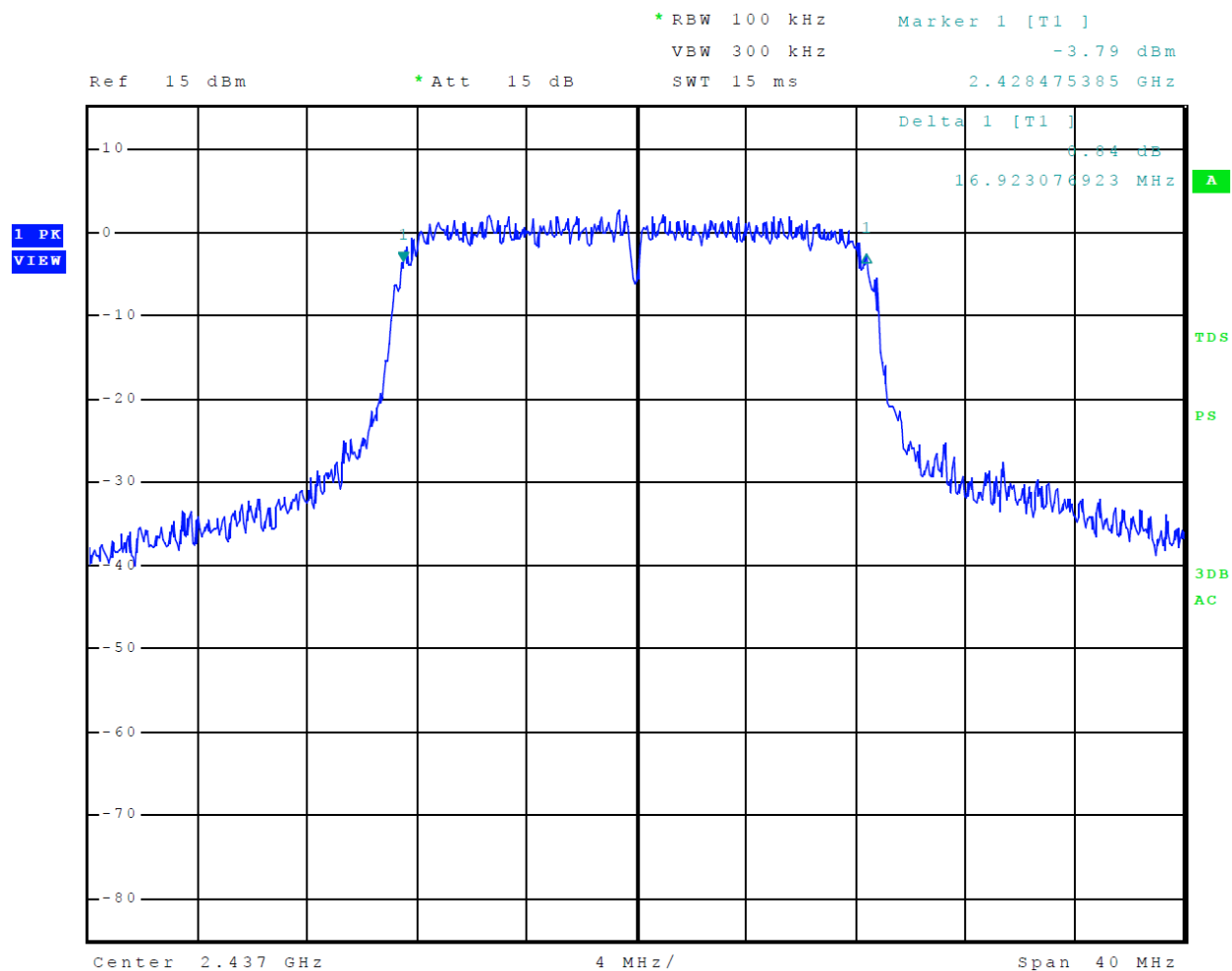
Figure 24 Mode 5 802.11n Plot of 6-dB Occupied Bandwidth
