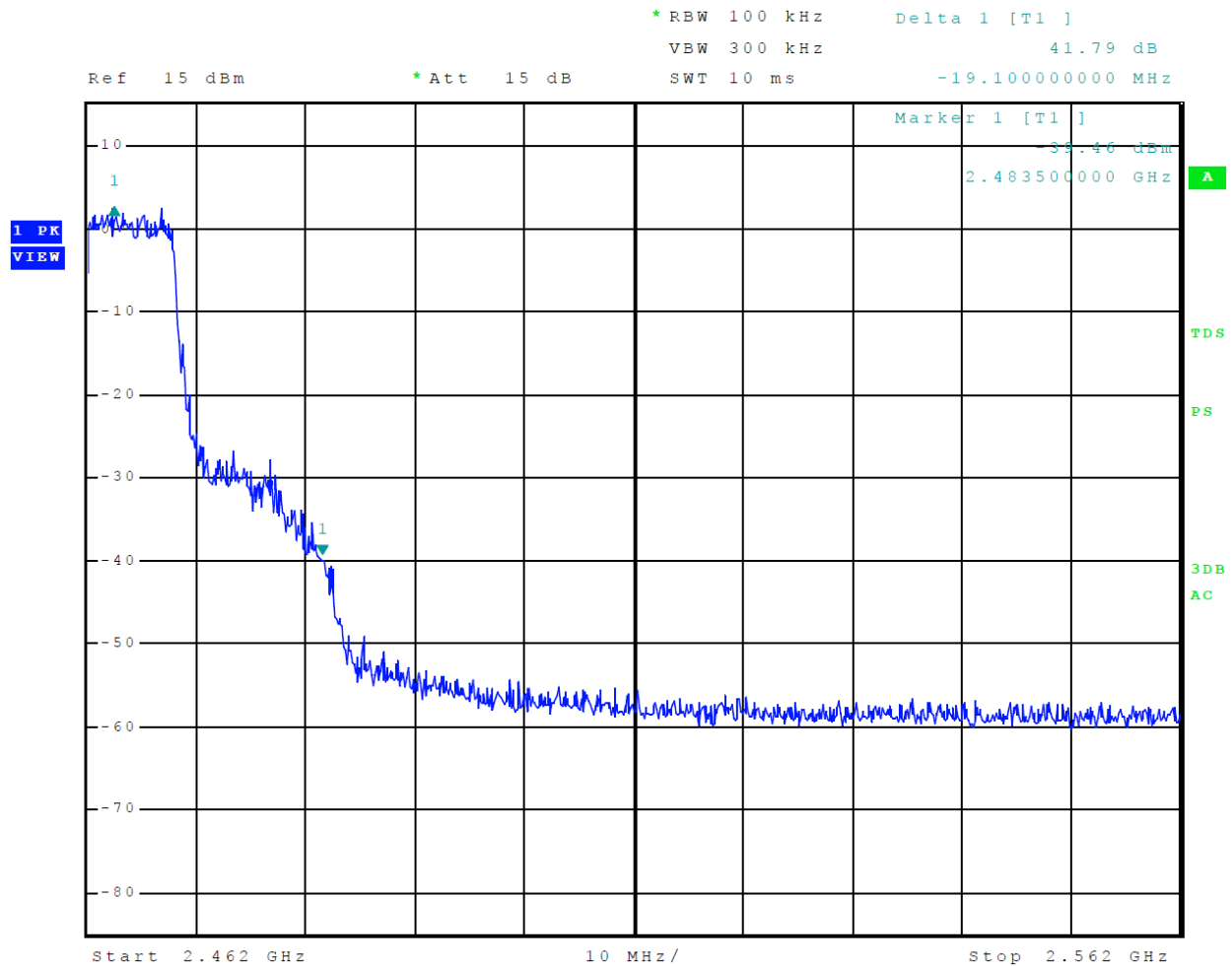
Figure 15 Mode 4 802.11g Plot of Transmitter Emissions High Band Edge
