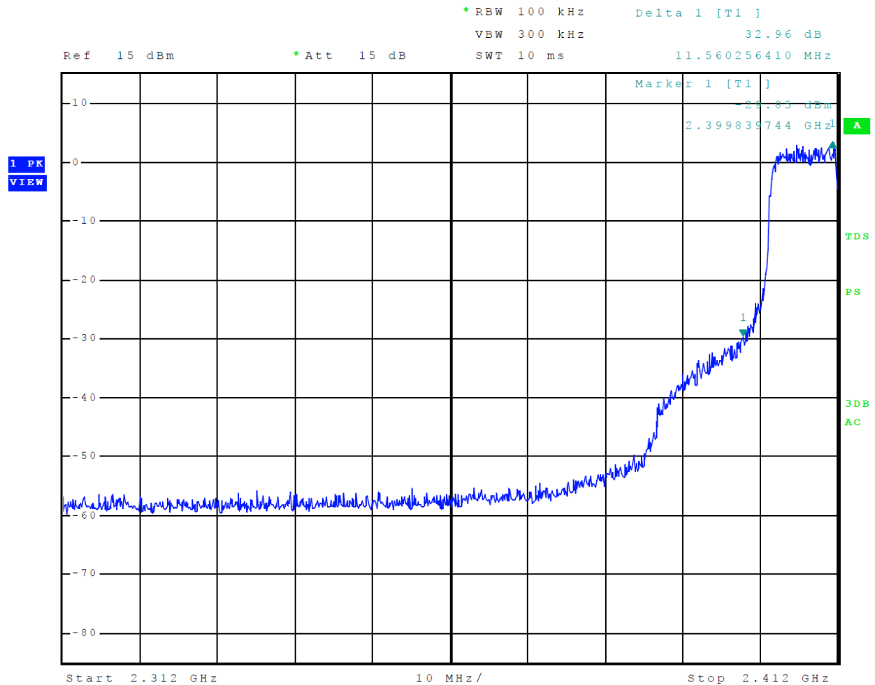
Figure 11 Mode 5 802.11n Plot of Transmitter Emissions Low Band Edge
