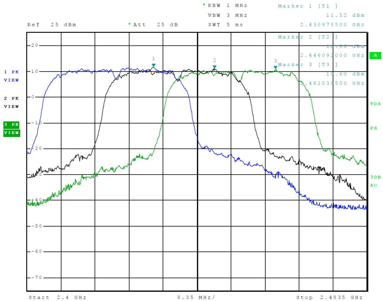
Figure 7 Mode 6 802.11n40 Plot of Transmitter Operation in 2412-2462 MHz
