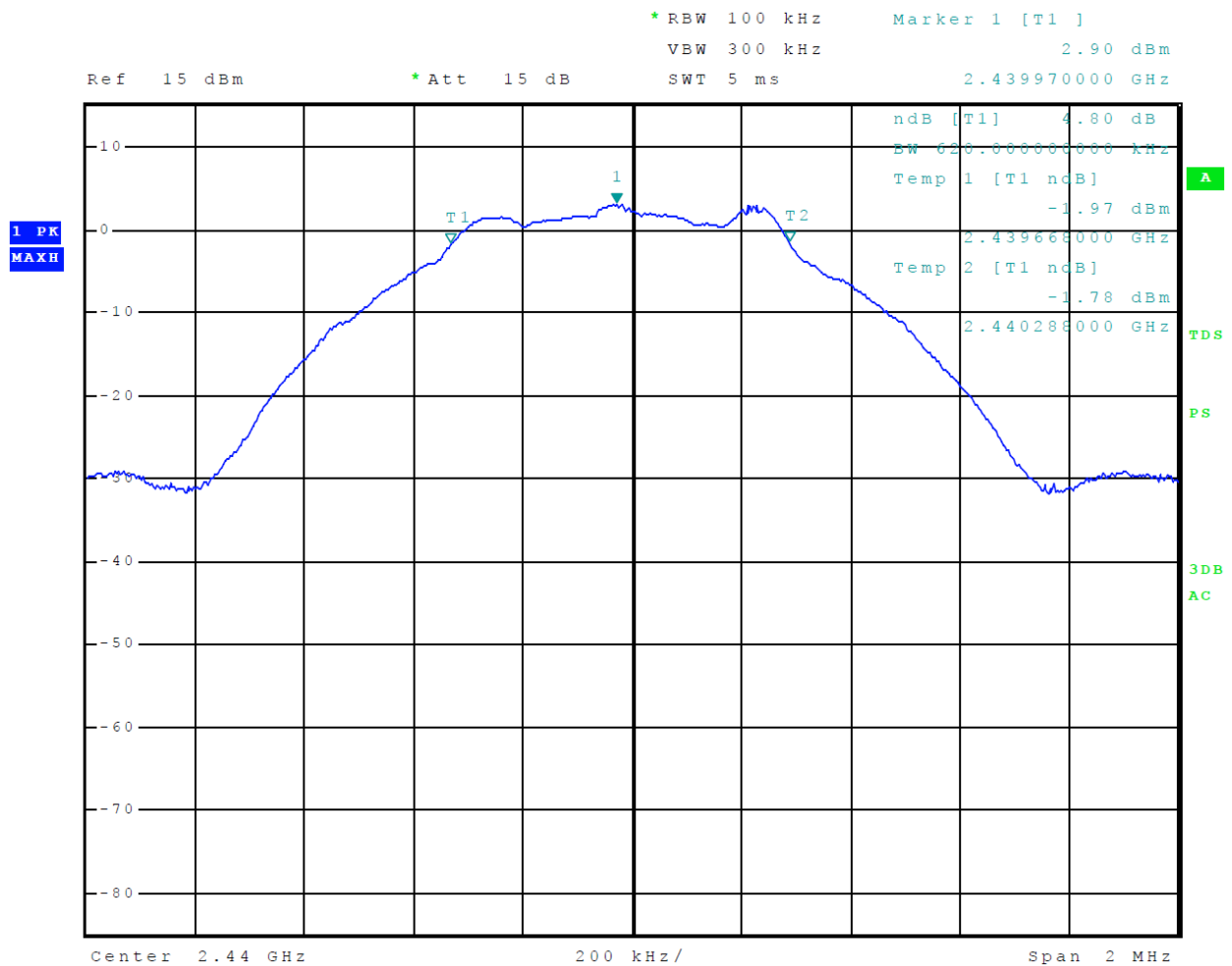
Figure 18 Mode 2 BT BLE Plot of 6-dB Occupied Bandwidth
