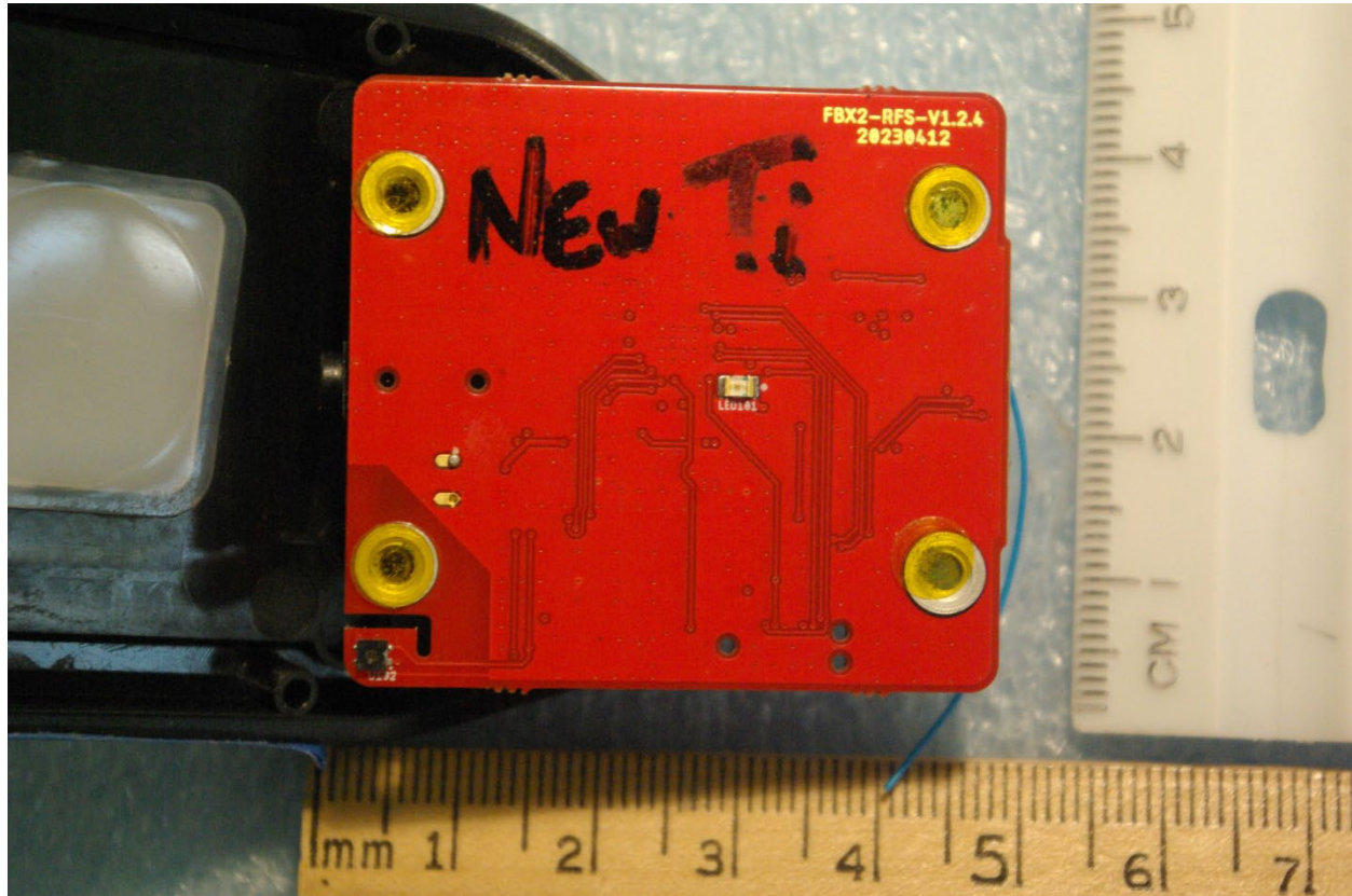
Back Side PCB
