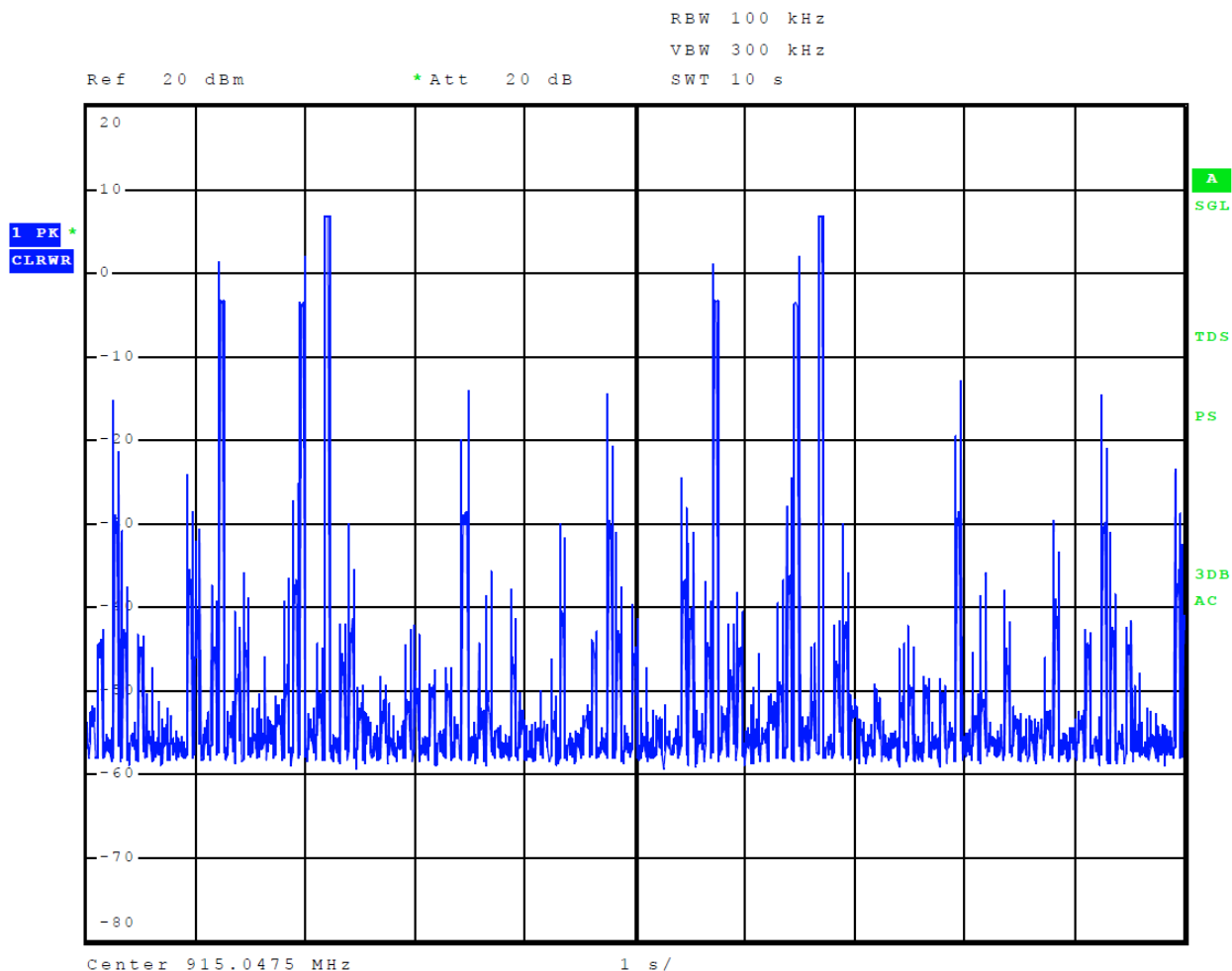
Figure 7 Plot of Number of Times on Channel over 10 Second Period
