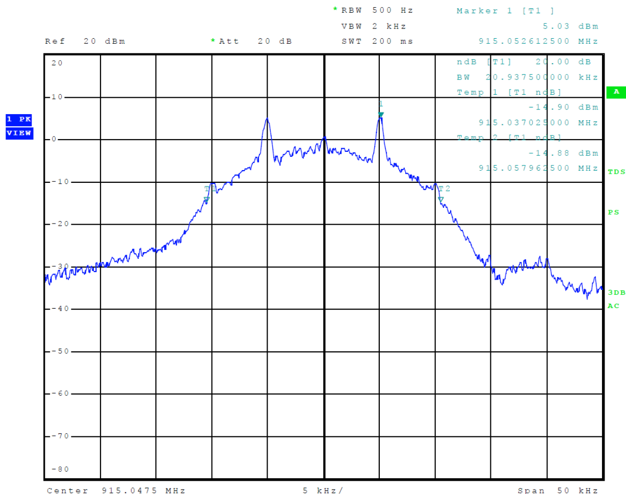
Figure 2 Plot of Transmitter Emissions 20-dB Occupied Bandwidth
