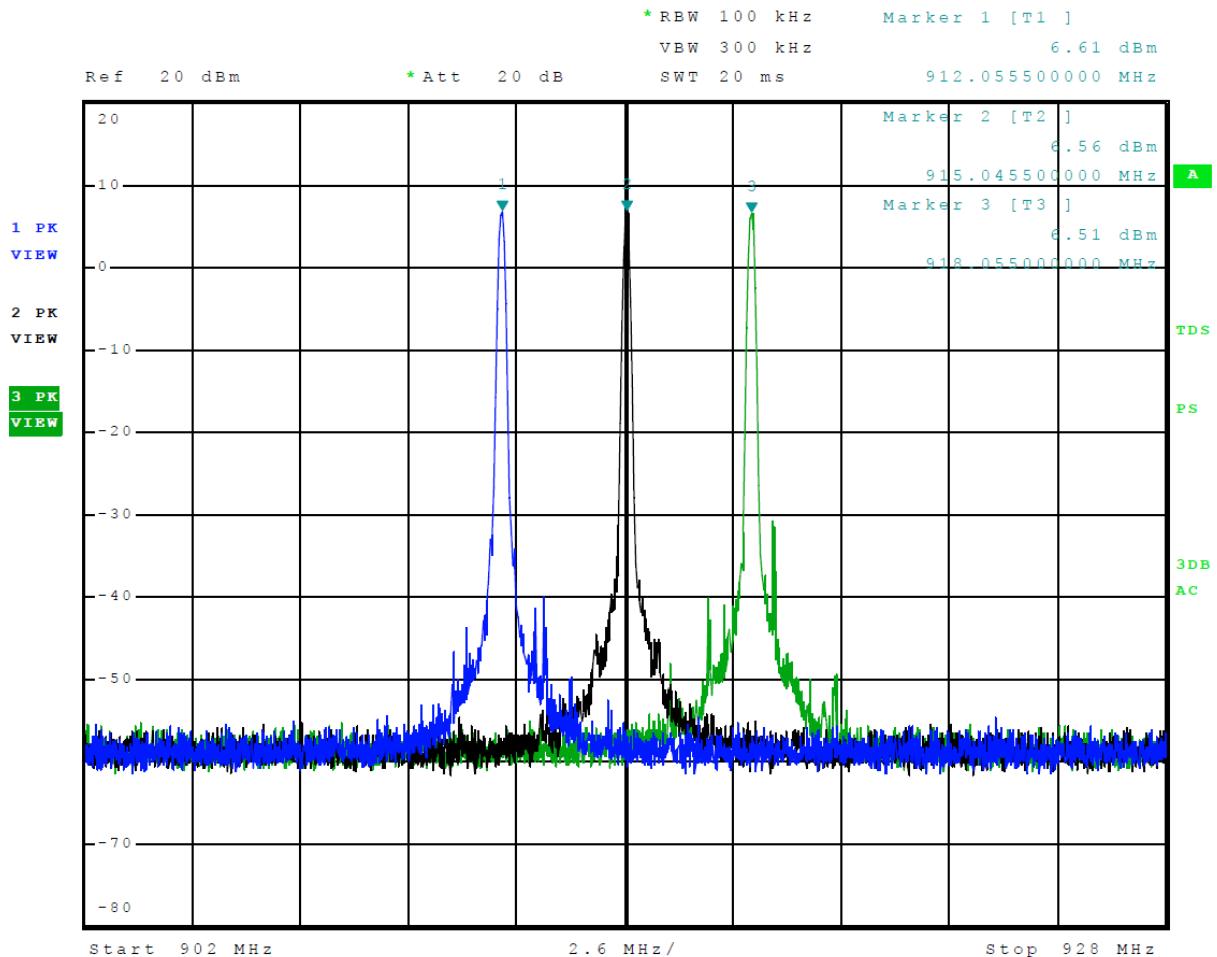
Figure 1 Plot of Transmitter Emissions Operation in 902-928 MHz
