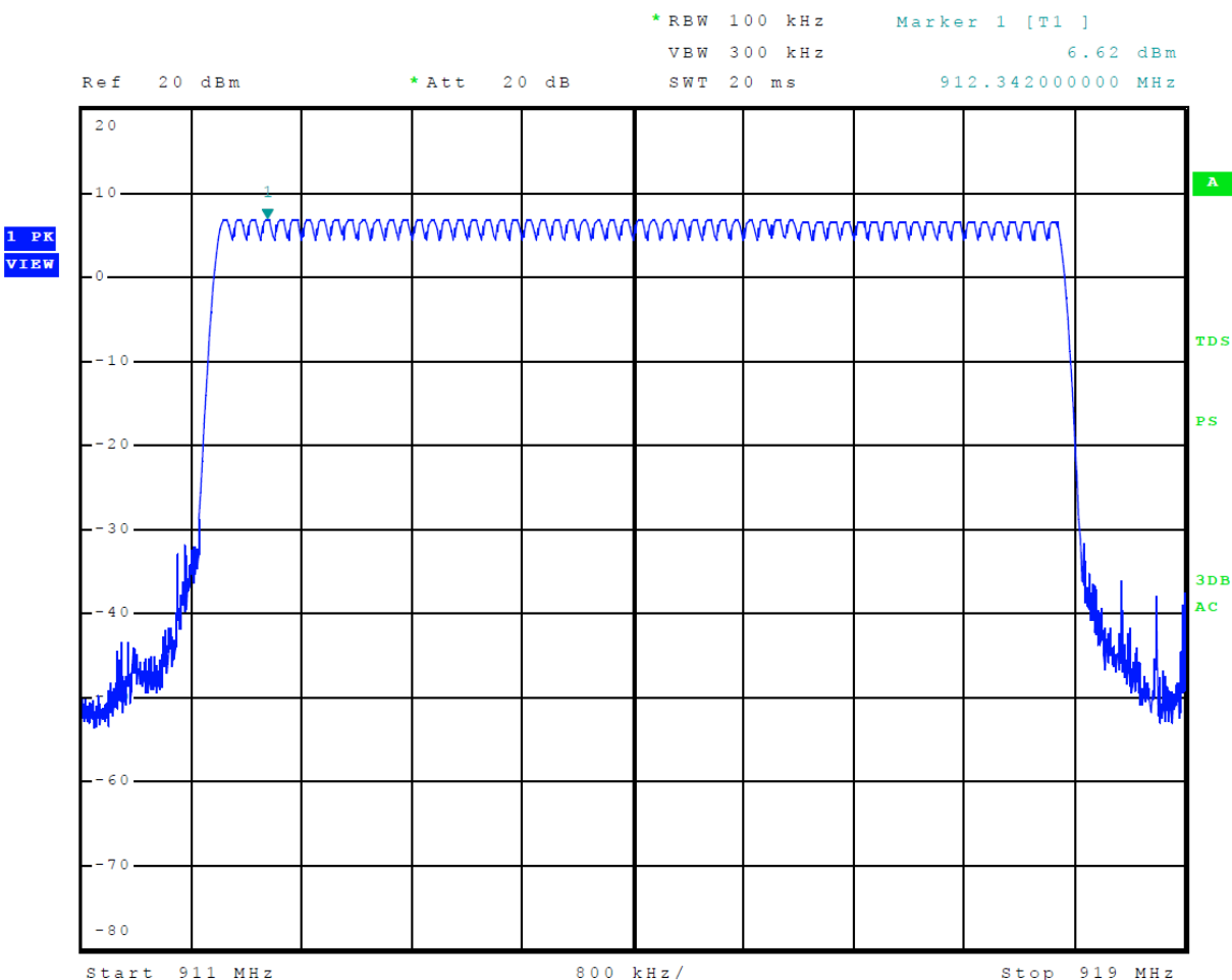
Figure 4 Plot of Number of Hopping Channels
