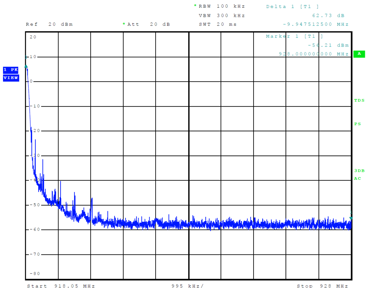
Figure 9 Plot of Transmitter Emissions High Band Edge
