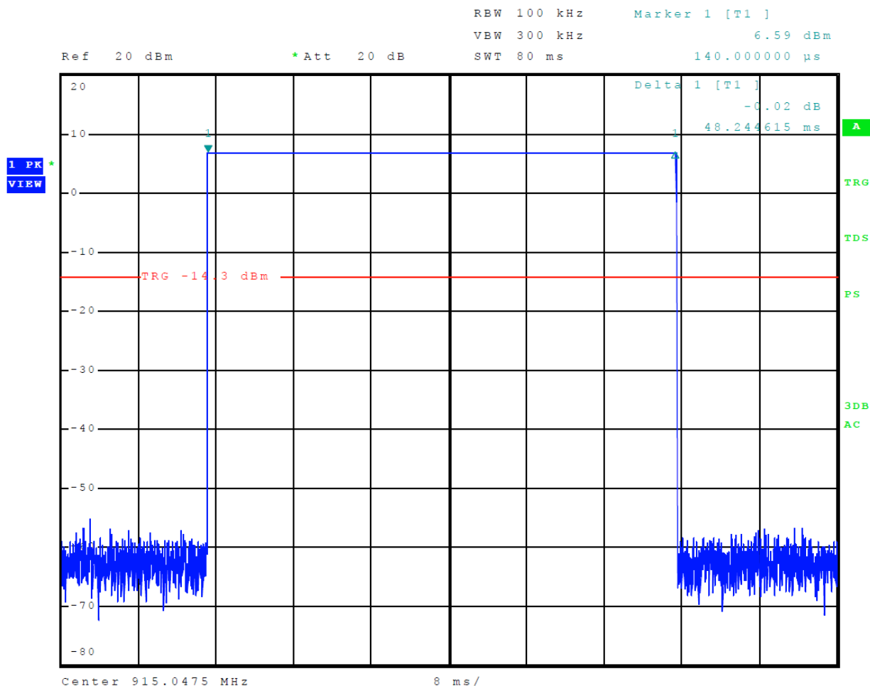
Figure 6 Plot of Dwell time On Channel
