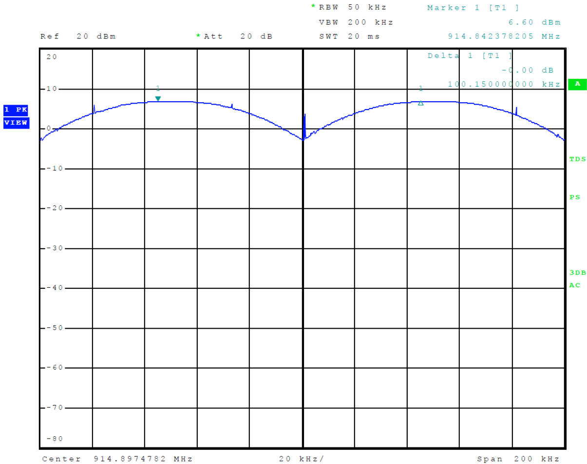
Figure 5 Plot of Channel Separation
