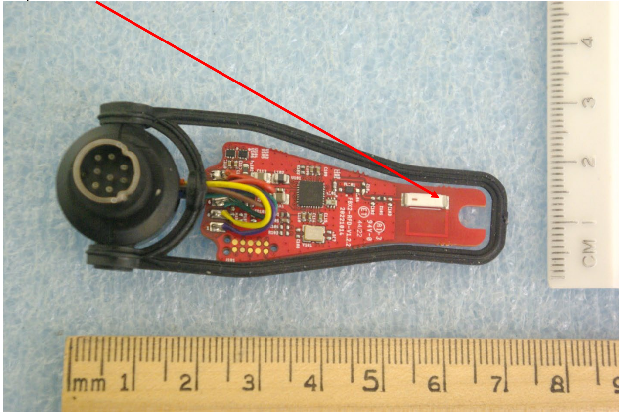
Chip Antenna
