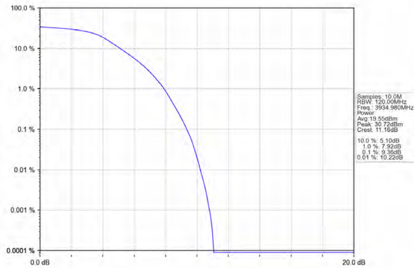
n77a_30kHz_SISO_NTNV_90MHz_DFT-s-OFDM_QPSK_3934.98MHz_Outer_Full_Ant1
