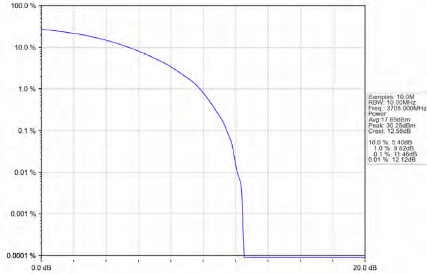
n77a_30kHz_SISO_NTNV_10MHz_CP-OFDM_16_QAM_3705MHz_Outer_Full_Ant1
