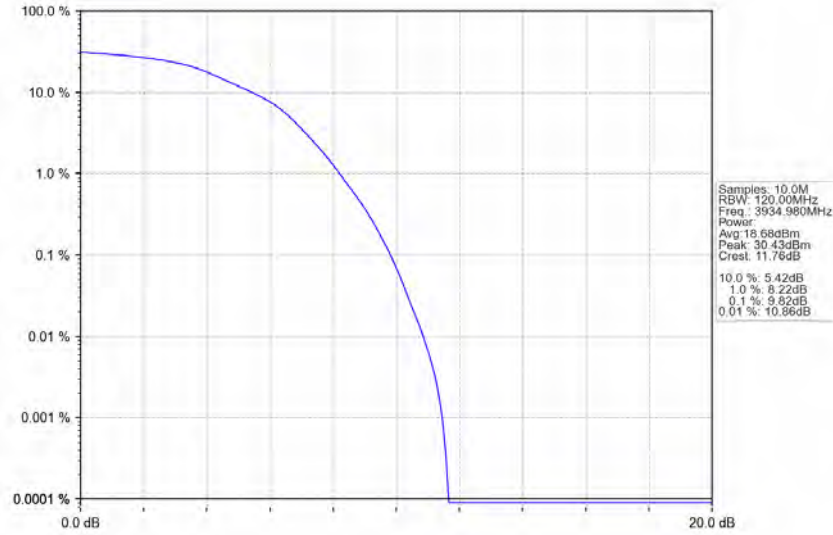
n77a_30kHz_SISO_NTNV_90MHz_DFT-s-OFDM 16 QAM 3934.98MHz_Outer_Full_Ant1
