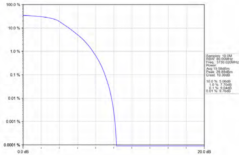
n77a_30kHz_SISO_NTNV_60MHz_DFT-s-OFDM QPSK_3730.02MHz_Outer_Full_Ant1
