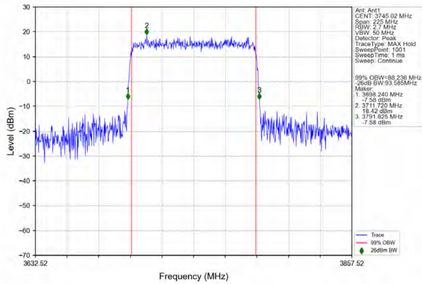
n77a_30kHz_SISO_NTNV_90MHz_CP-OFDM_QPSK_3745.02MHz_Outer_Full_Ant1
