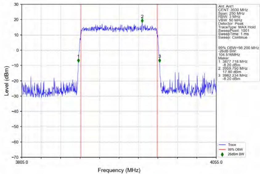
n77a_30kHz_SISO_NTNV_100MHz_CP-OFDM_64_QAM_3930MHz_Outer_Full_Ant1
