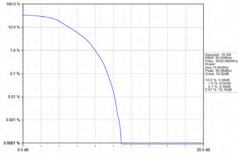
n77a_30kHz_SISO_NTNV_80MHz_DFT-s-OFDM_QPSK_3939.99MHz_Outer_Full_Ant1
