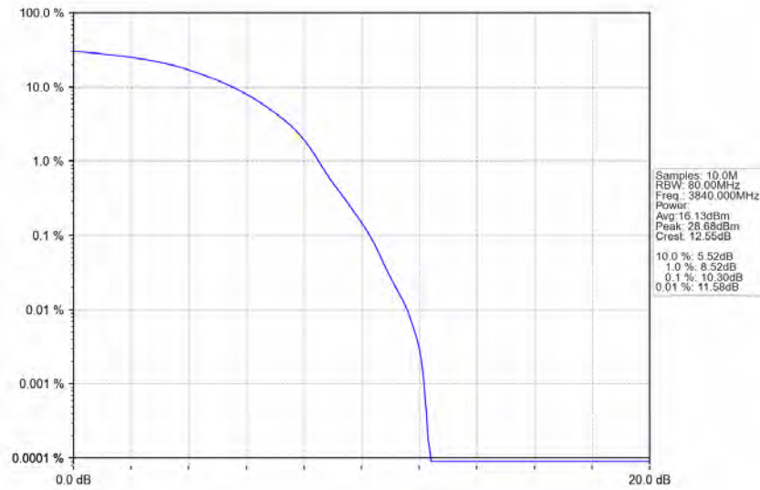
n77a_30kHz_SISO_NTNV_50MHz_DFT-s-OFDM_256_QAM_3840MHz_Outer_Full_Ant1
