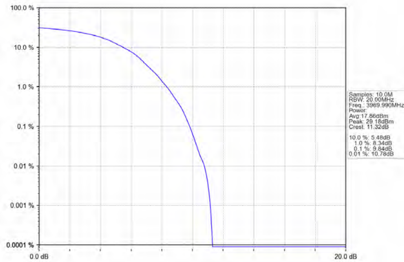
n77a_30kHz_SISO_NTNV_20MHz_DFT-s-OFDM_64_QAM_3969.99MHz_Outer_Full_Ant1
