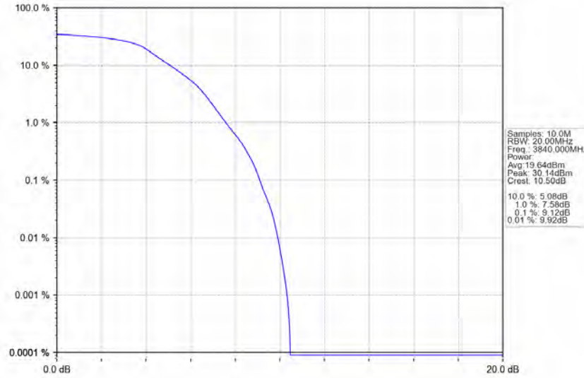
n77a_30kHz_SISO_NTNV_20MHz_DFT-s-OFDM_QPSK_3840MHz_Outer_Full_Ant1
