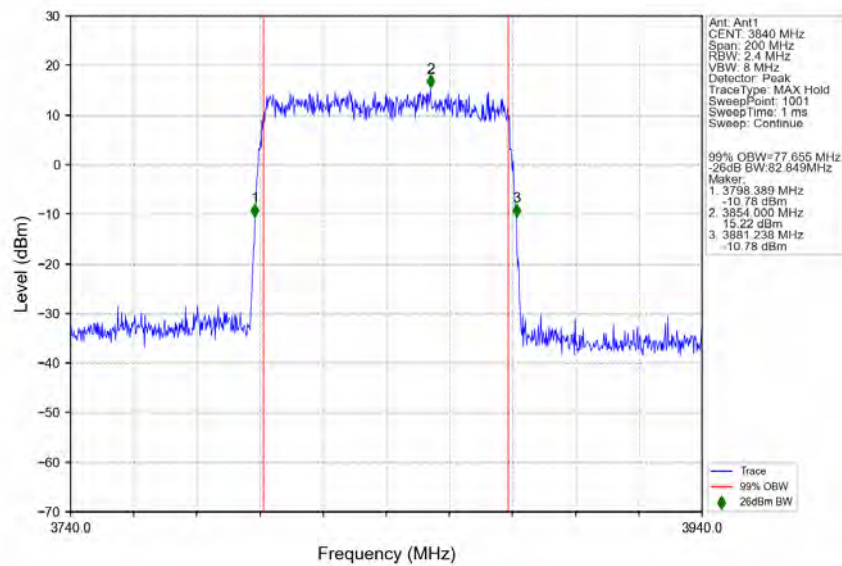
n77a_30kHz_SISO_NTNV_80MHz_DFT-s-OFDM_256_QAM_3840MHz_Outer_Full_Ant1
