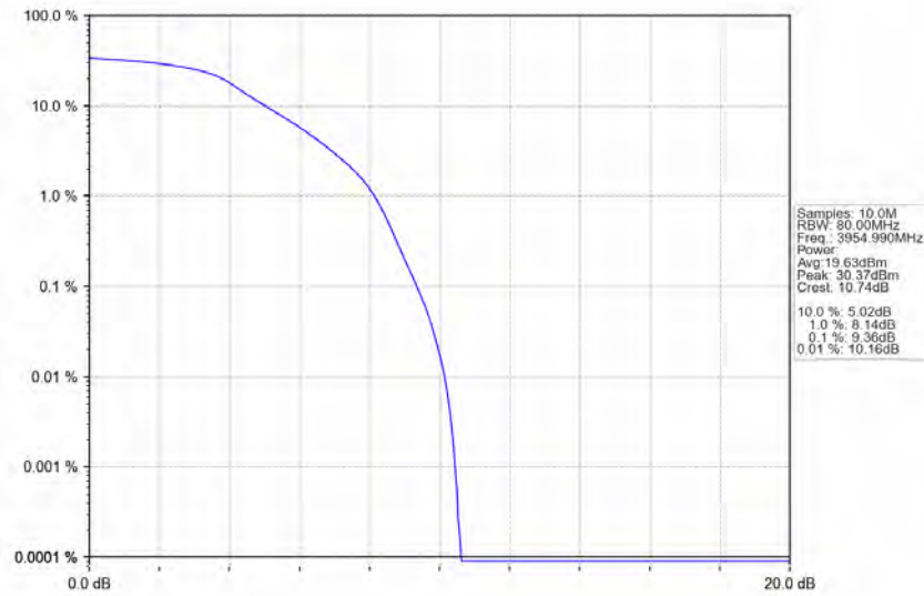
n77a_30kHz_SISO_NTNV_50MHz_DFT-s-OFDM_QPSK_3954.99MHz_Outer_Full_Ant1
