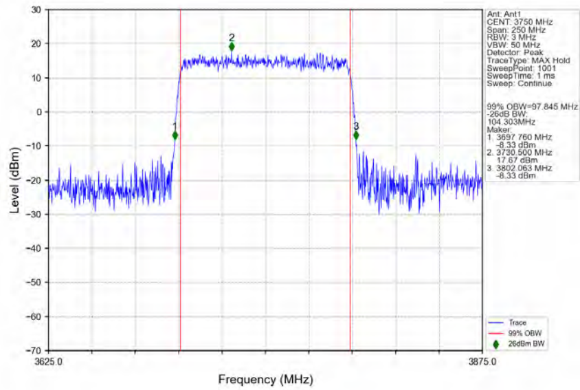
n77a_30kHz_SISO_NTNV_100MHz_CP-OFDM 64 QAM_3750MHz_Outer_Full_Ant1
