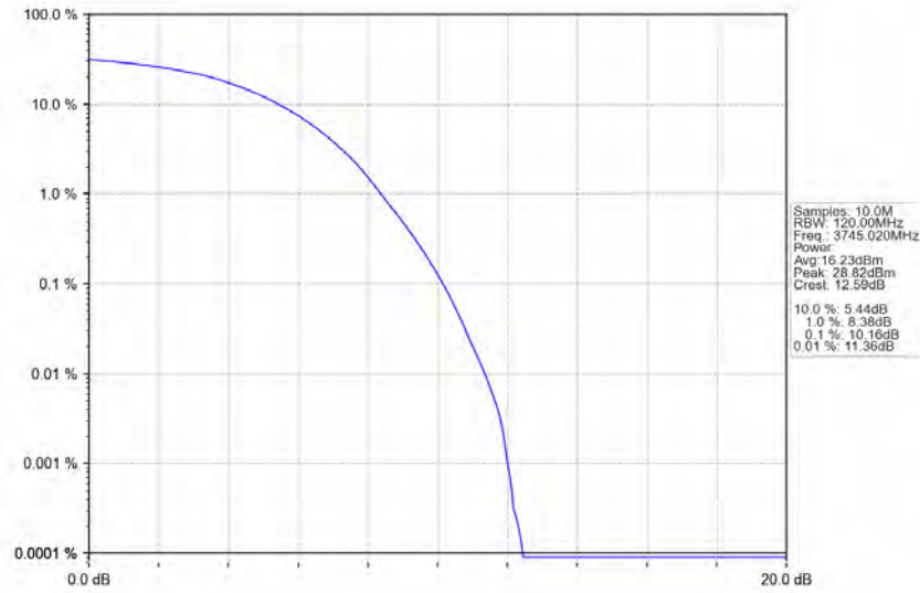
n77a_30kHz_SISO_NTNV_90MHz_DFT-s-OFDM_256_QAM_3745.02MHz_Outer_Full_Ant1
