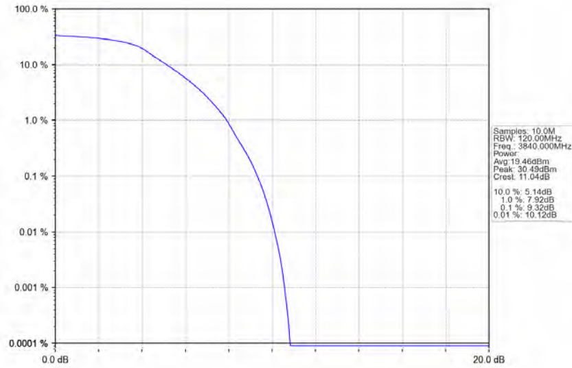
n77a_30kHz_SISO_NTNV_90MHz_DFT-s-OFDM_QPSK_3840MHz_Outer_Full_Ant1
