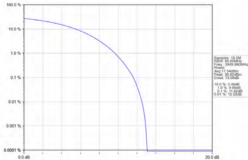
n77a_30kHz_SISO_NTNV_60MHz_CP-OFDM_QPSK_3949.98MHz_Outer_Full_Ant1
