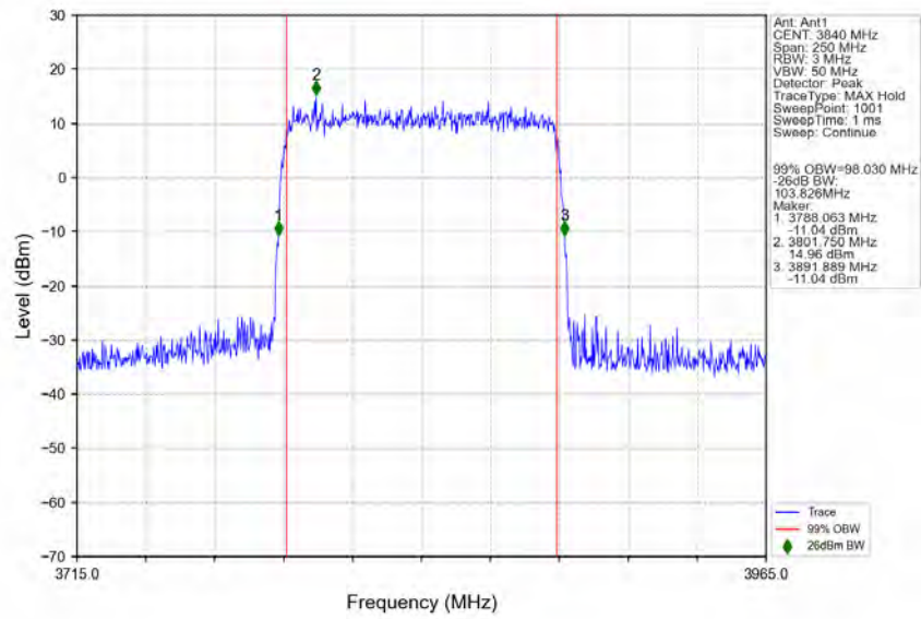
n77a_30kHz_SISO_NTNV_100MHz_CP-OFDM_256_QAM_3840MHz_Outer_Full_Ant1
