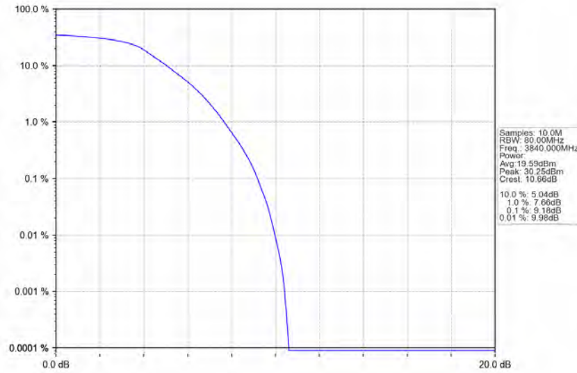
n77a_30kHz_SISO_NTNV_60MHz_DFT-s-OFDM_QPSK_3840MHz_Outer_Full_Ant1
