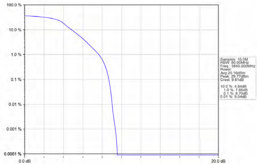
n77a_30kHz_SISO_NTNV_50MHz_DFT-s-OFDM PI/2 BPSK_3840MHz_Outer_Full_Ant1
