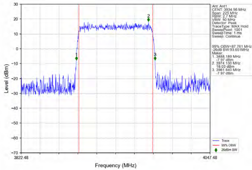
n77a_30kHz_SISO_NTNV_90MHz_CP-OFDM_QPSK_3934.98MHz_Outer_Full_Ant1
