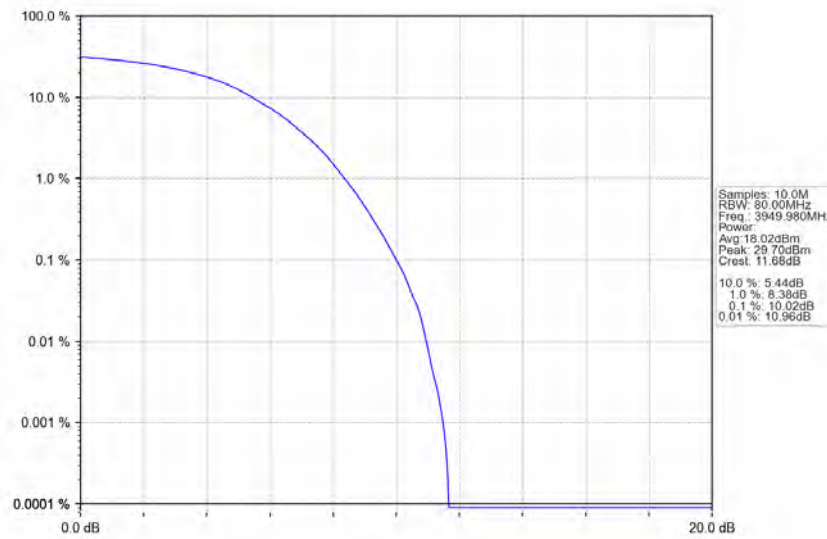
n77a_30kHz_SISO_NTNV_60MHz_DFT-s-OFDM_64_QAM_3949.98MHz_Outer_Full_Ant1
