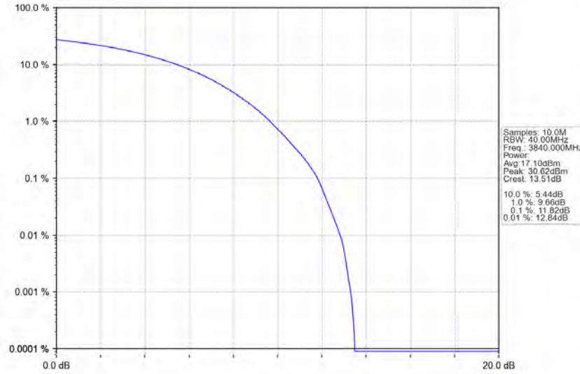
n77a_30kHz_SISO_NTNV_40MHz_CP-OFDM 64 QAM_3840MHz_Outer_Full_Ant1
