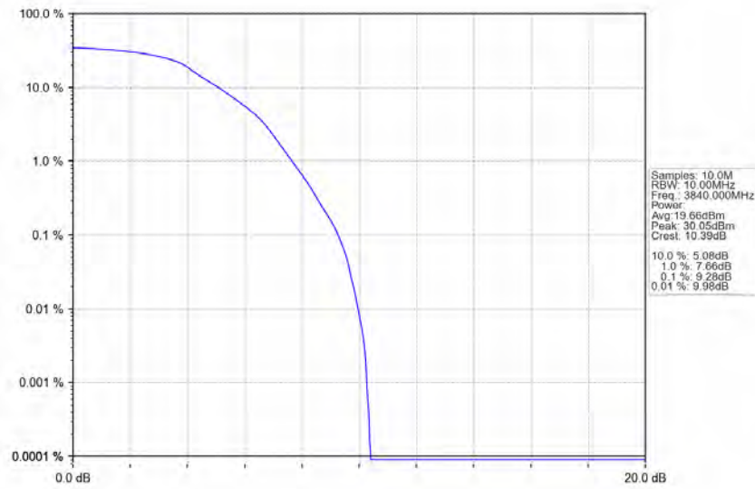
n77a_30kHz_SISO_NTNV_10MHz_DFT-s-OFDM_QPSK_3840MHz_Outer_Full_Ant1
