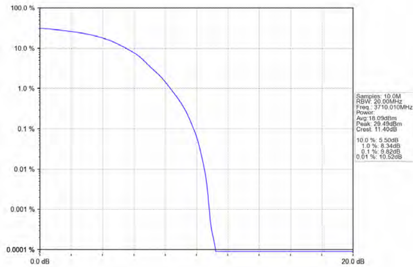
n77a_30kHz_SISO_NTNV_20MHz_DFT-s-OFDM_64_QAM_3710.01MHz_Outer_Full_Ant1
