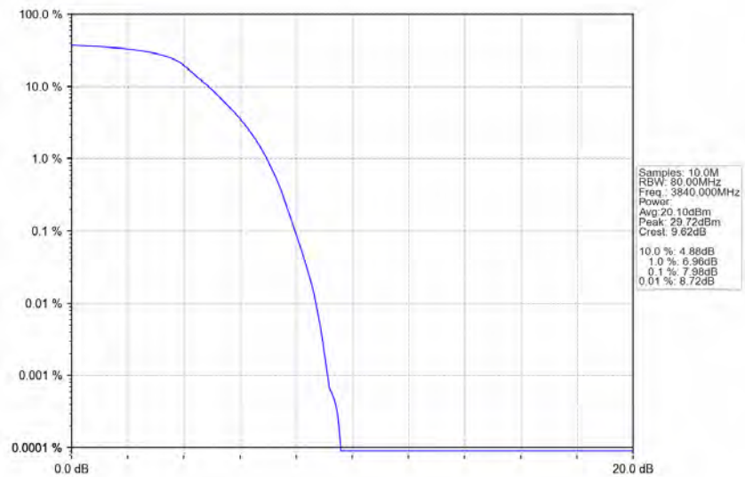
n77a_30kHz_SISO_NTNV_60MHz_DFT-s-OFDM PI/2 BPSK_3840MHz_Outer_Full_Ant1
