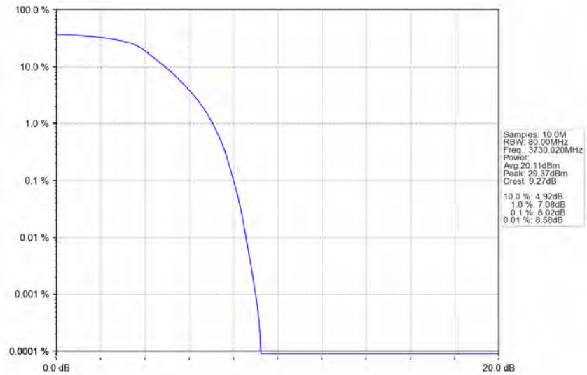
n77a_30kHz_SISO_NTNV_60MHz_DFT-s-OFDM PI/2 BPSK_3730.02MHz_Outer_Full_Ant1
