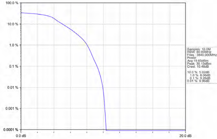
n77a_30kHz_SISO_NTNV_50MHz_DFT-s-OFDM_QPSK_3840MHz_Outer_Full_Ant1
