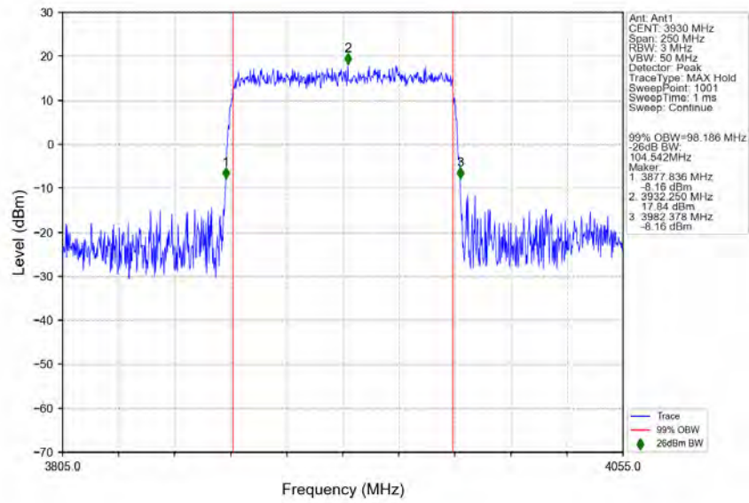
n77a_30kHz_SISO_NTNV_100MHz_CP-OFDM_QPSK_3930MHz_Outer_Full_Ant1
