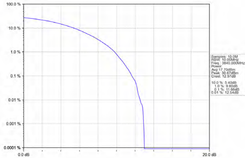
n77a_30kHz_SISO_NTNV_10MHz_CP-OFDM_16_QAM_3840MHz_Outer_Full_Ant1
