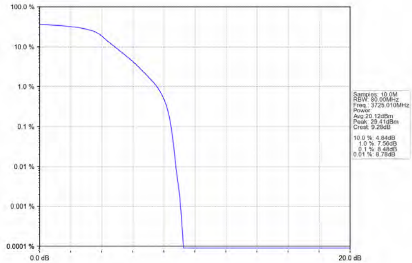
n77a_30kHz_SISO_NTNV_50MHz_DFT-s-OFDM PI/2 BPSK_3725.01MHz_Outer_Full_Ant1
