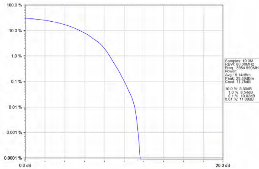
n77a_30kHz_SISO_NTNV_50MHz_DFT-s-OFDM_64_QAM_3954.99MHz_Outer_Full_Ant1
