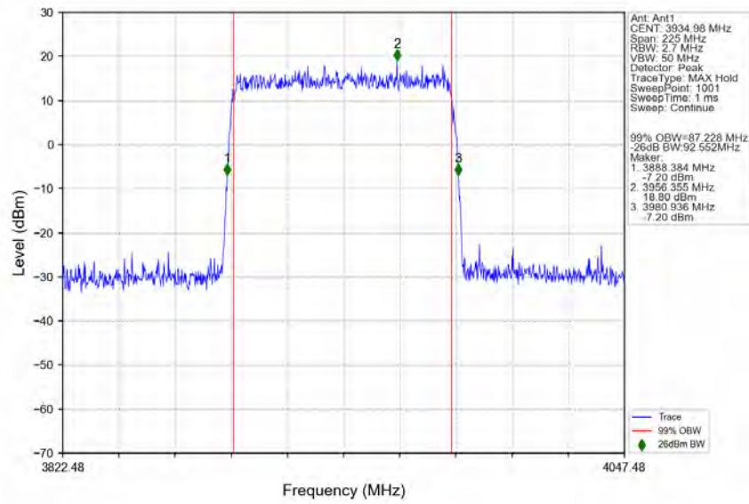
n77a_30kHz_SISO_NTNV_90MHz_DFT-s-OFDM 64 QAM 3934.98MHz_Outer_Full_Ant1
