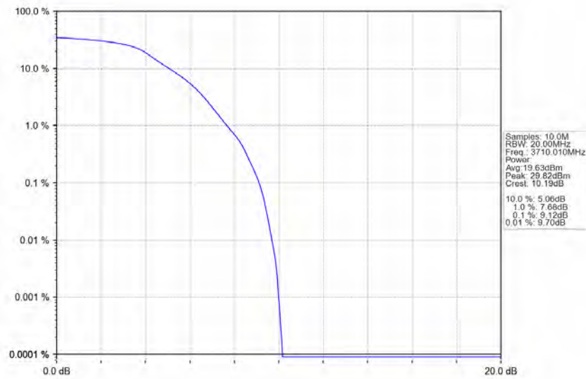
n77a_30kHz_SISO_NTNV_20MHz_DFT-s-OFDM QPSK_3710.01MHz_Outer_Full_Ant1
