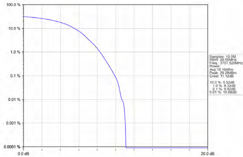
n77a_30kHz_SISO_NTNV_15MHz_DFT-s-OFDM_64_QAM_3707.52MHz_Outer_Full_Ant1
