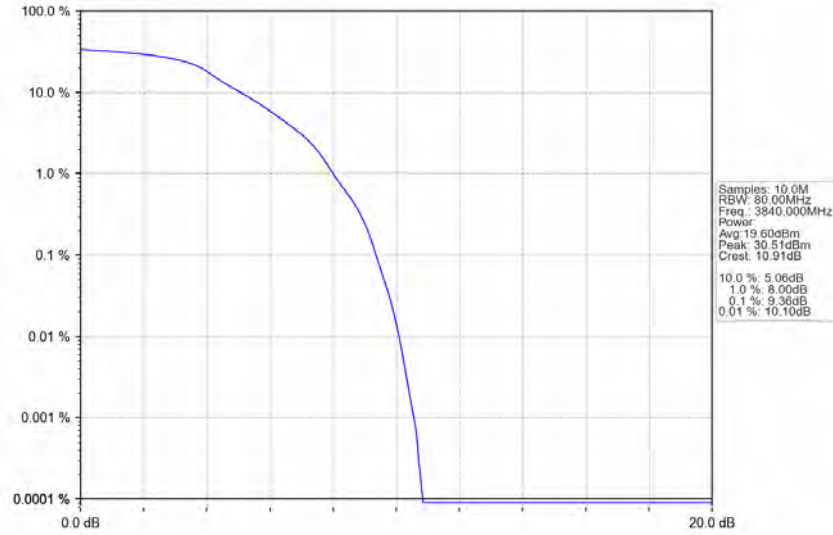
n77a_30kHz_SISO_NTNV_80MHz_DFT-s-OFDM_QPSK_3840MHz_Outer_Full_Ant1
