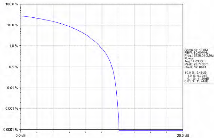
n77a_30kHz_SISO_NTNV_50MHz_CP-OFDM_QPSK_3725.01MHz_Outer_Full_Ant1
