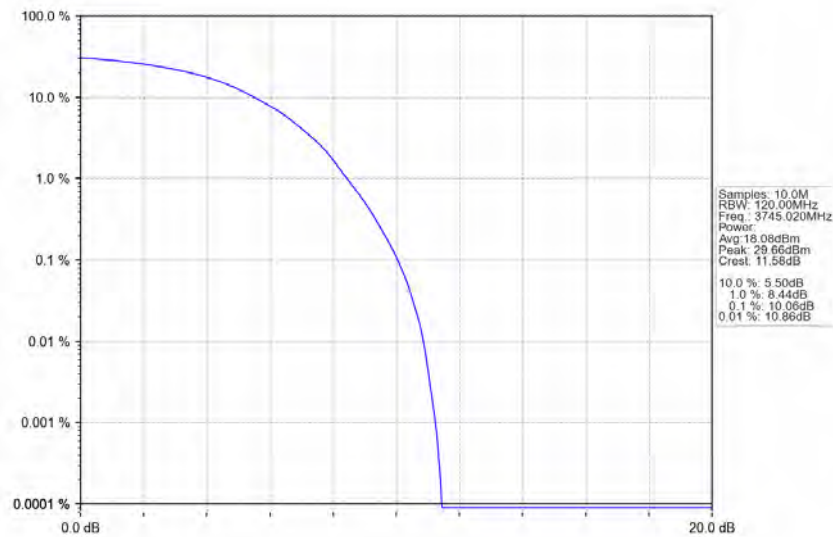
n77a_30kHz_SISO_NTNV_90MHz_DFT-s-OFDM 64 QAM 3745.02MHz_Outer_Full_Ant1
