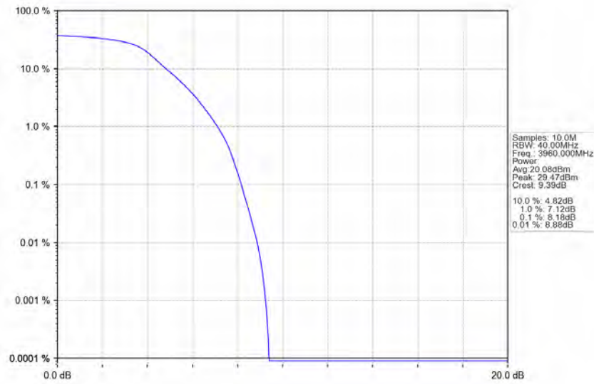
n77a_30kHz_SISO_NTNV_40MHz_DFT-s-OFDM_PI/2_BPSK_3960MHz_Outer_Full_Ant1
