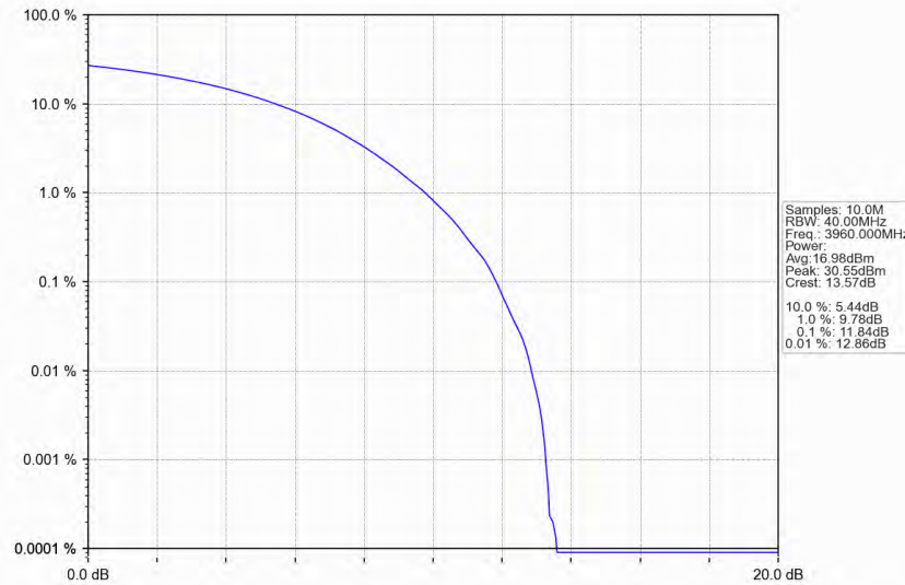
n77a_30kHz_SISO_NTNV_40MHz_CP-OFDM 64 QAM_3960MHz_Outer_Full_Ant1
