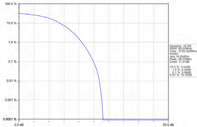
n77a_30kHz_SISO_NTNV_60MHz_DFT-s-OFDM_64_QAM_3730.02MHz_Outer_Full_Ant1
