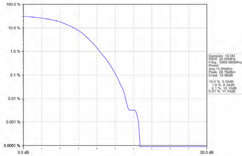
n77a_30kHz_SISO_NTNV_20MHz_DFT-s-OFDM_256_QAM_3969.99MHz_Outer_Full_Ant1
