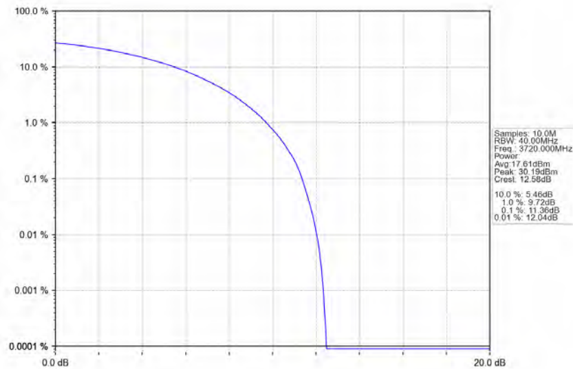
n77a_30kHz_SISO_NTNV_40MHz_CP-OFDM_QPSK_3720MHz_Outer_Full_Ant1
