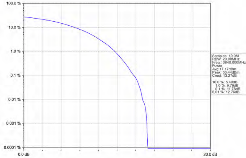
n77a_30kHz_SISO_NTNV_15MHz_CP-OFDM_64_QAM_3840MHz_Outer_Full_Ant1
