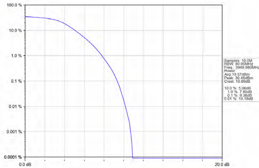
n77a_30kHz_SISO_NTNV_60MHz_DFT-s-OFDM_QPSK_3949.98MHz_Outer_Full_Ant1
