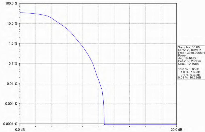
n77a_30kHz_SISO_NTNV_20MHz_DFT-s-OFDM_QPSK_3969.99MHz_Outer_Full_Ant1
