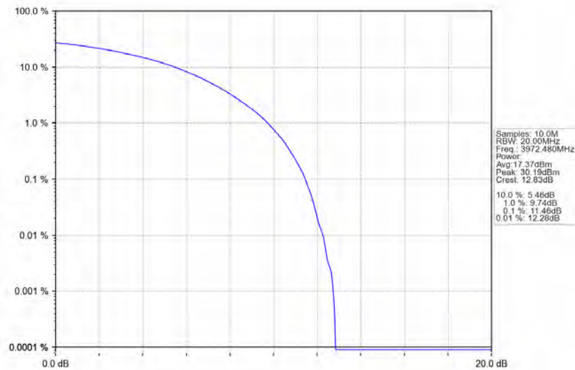
n77a_30kHz_SISO_NTNV_15MHz_CP-OFDM_QPSK_3972.48MHz_Outer_Full_Ant1
