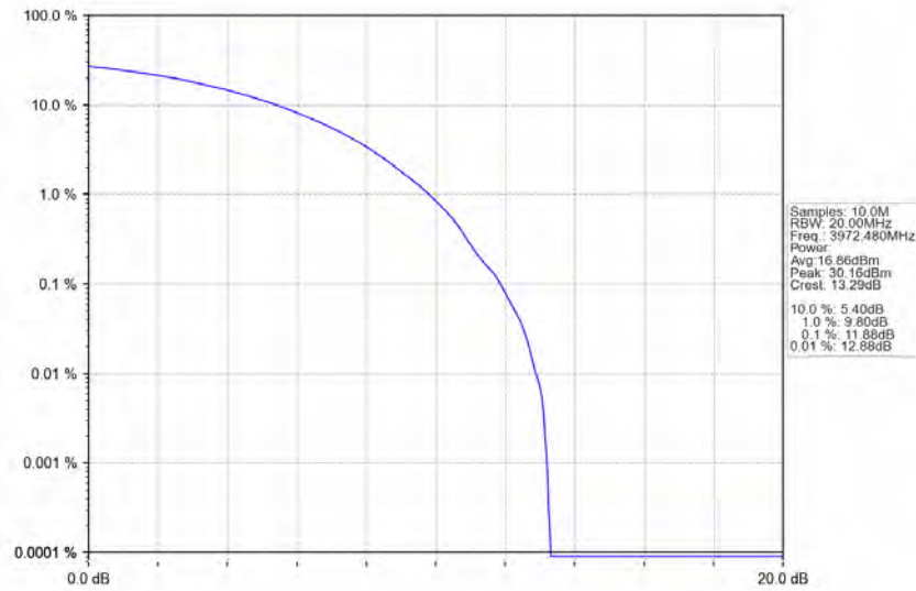
n77a_30kHz_SISO_NTNV_15MHz_CP-OFDM_64_QAM_3972.48MHz_Outer_Full_Ant1
