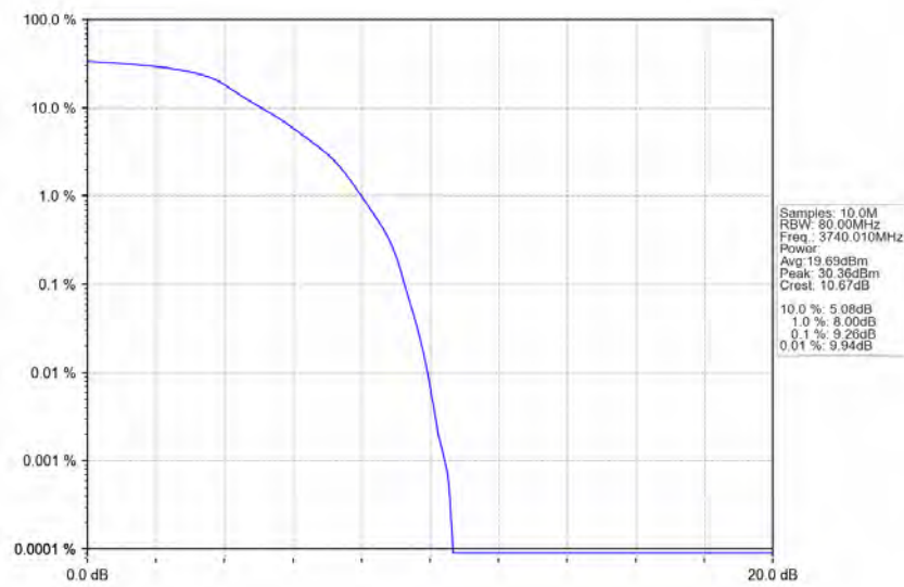
n77a_30kHz_SISO_NTNV_80MHz_DFT-s-OFDM QPSK_3740.01MHz_Outer_Full_Ant1
