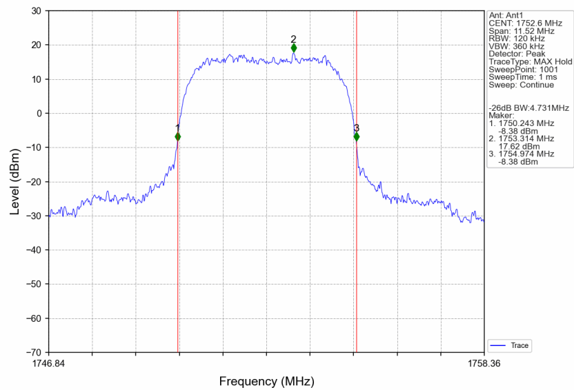
Band4_HSDPA_HCH_1752.6MHz_Subtest 1_NTNV
