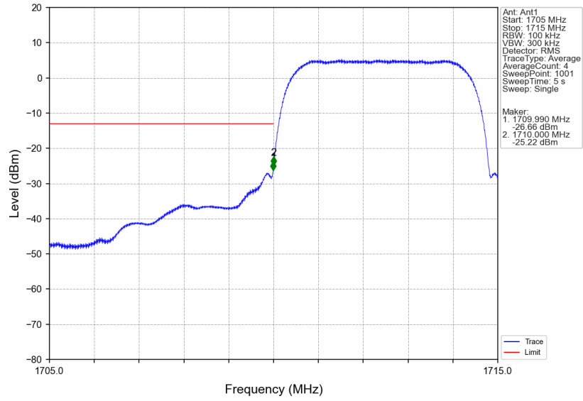
Band4_HSDPA_LCH_1712.4MHz_Subtest 1_NTNV
