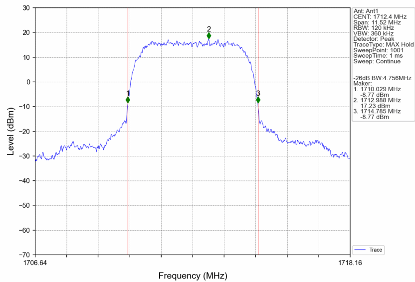
Band4_HSDPA_LCH_1712.4MHz_Subtest 1_NTNV
