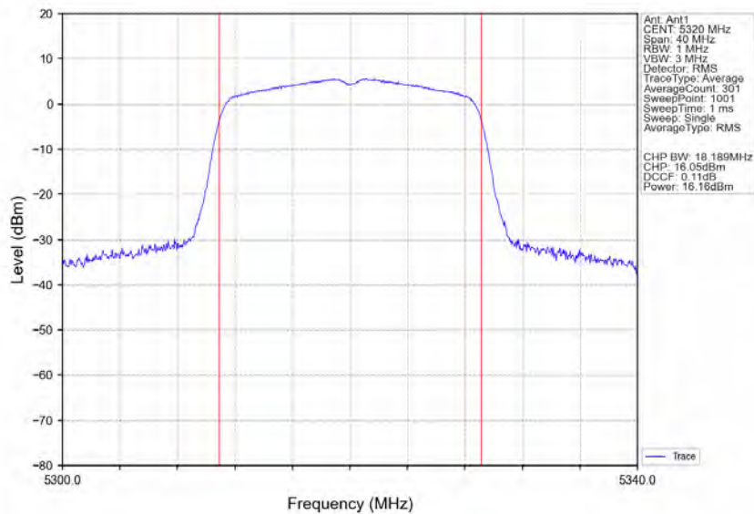
802.11ac(VHT20)_HCH_5320MHz_Ant1_NTNV
