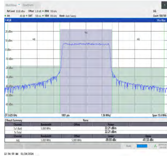
Band48-5MHz-QPSK-55990-25RB#0-PASS
