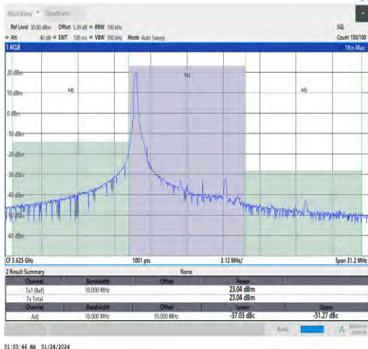
Band48-10MHz-QPSK-55990-1RB#0-PASS
