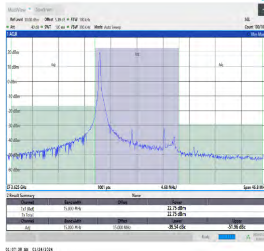
Band48-15MHz-QPSK-55990-1RB#0-PASS
