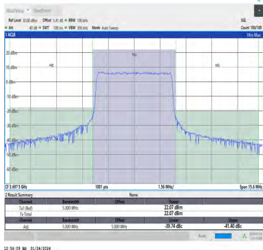
Band48-5MHz-QPSK-56715-25RB#0-PASS
