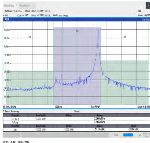
Band48-15MHz-QPSK-56665-1RB#74-PASS
