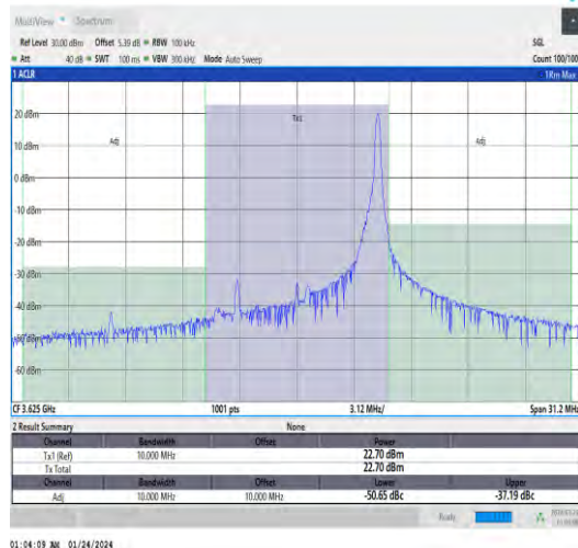
Band48-10MHz-QPSK-55990-1RB#49-PASS
