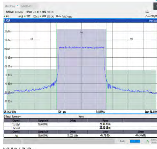
Band48-15MHz-QPSK-55990-75RB#0-PASS
