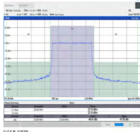
Band48-20MHz-QPSK-56640-100RB#0-PASS
