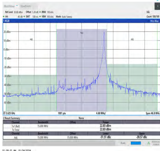
Band48-15MHz-QPSK-55990-1RB#74-PASS
