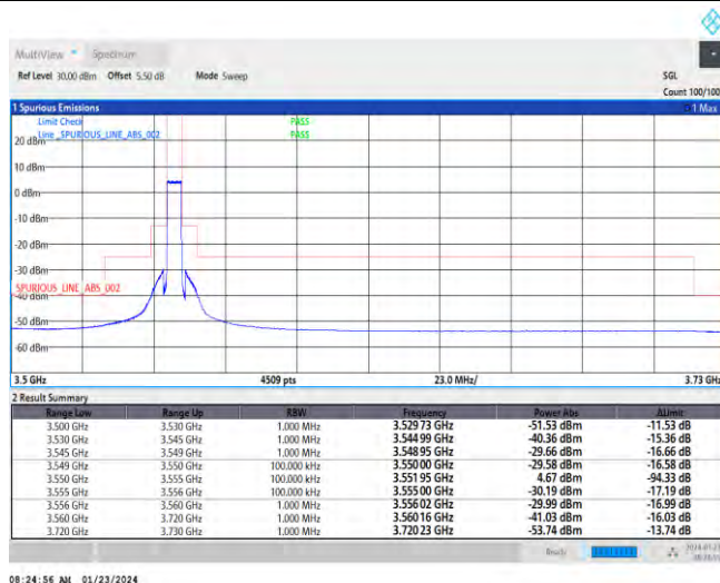
Band48-5MHz-QPSK-55265-25RB#0
