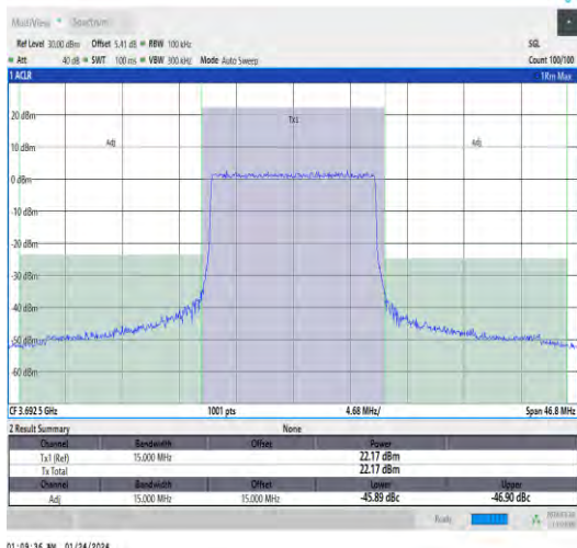
Band48-15MHz-QPSK-56665-75RB#0-PASS
