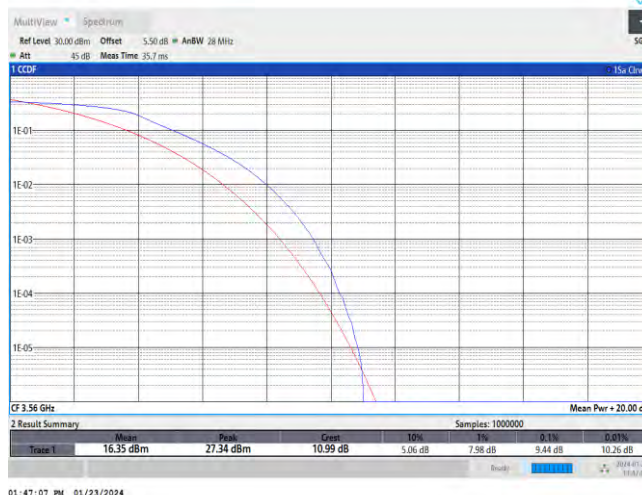
Band48-20MHz-QPSK-55990-100RB#0
