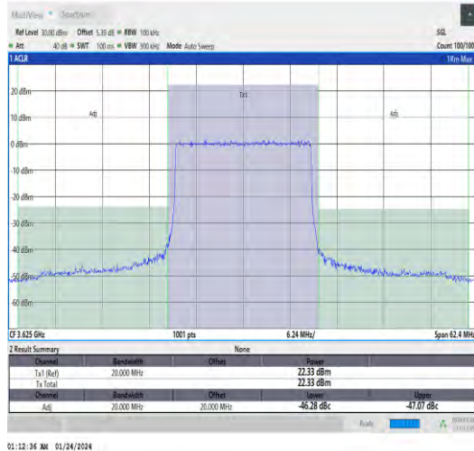
Band48-20MHz-QPSK-55990-100RB#0-PASS
