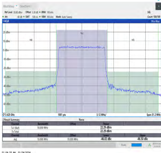
Band48-10MHz-QPSK-55990-50RB#0-PASS
