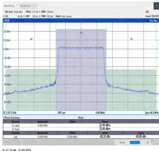
Band48-15MHz-QPSK-55315-75RB#0-PASS
