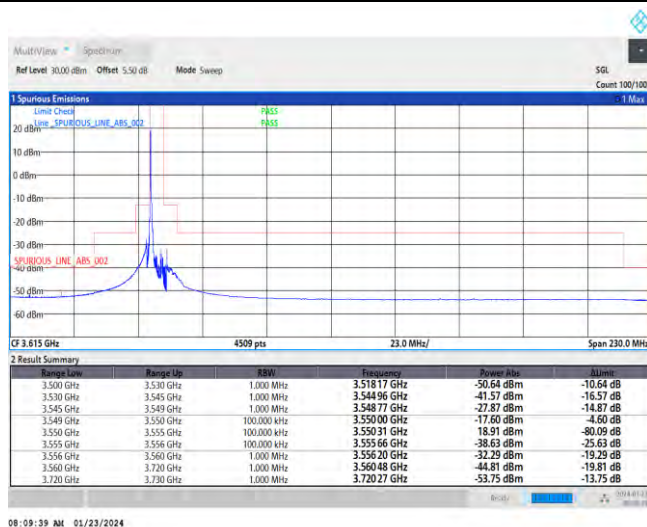
Band48-5MHz-QPSK-55265-25RB#0
