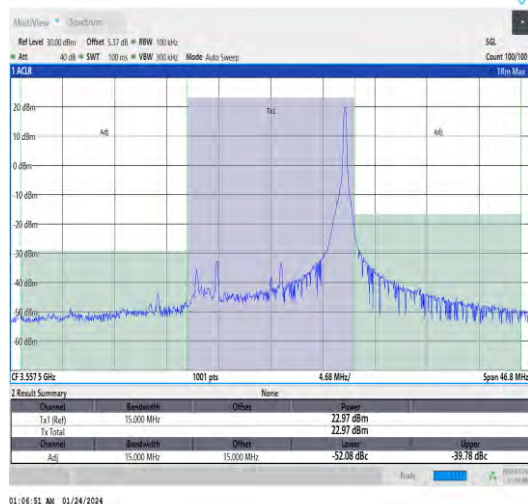
Band48-15MHz-QPSK-55315-1RB#74-PASS
