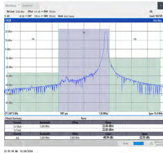
Band48-5MHz-QPSK-56715-1RB#24-PASS
