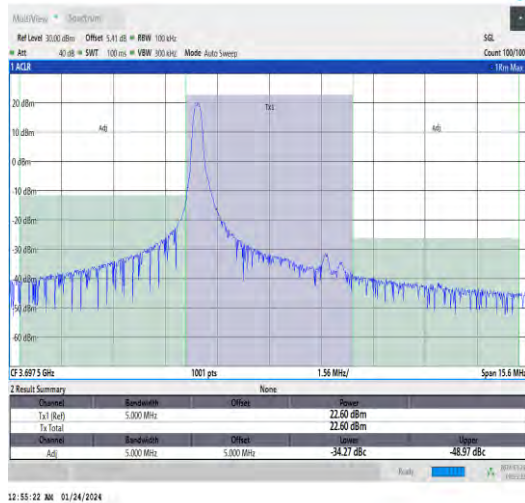
Band48-5MHz-QPSK-56715-1RB#0-PASS
