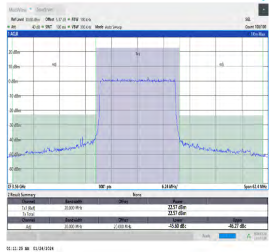
Band48-20MHz-QPSK-55340-100RB#0-PASS
