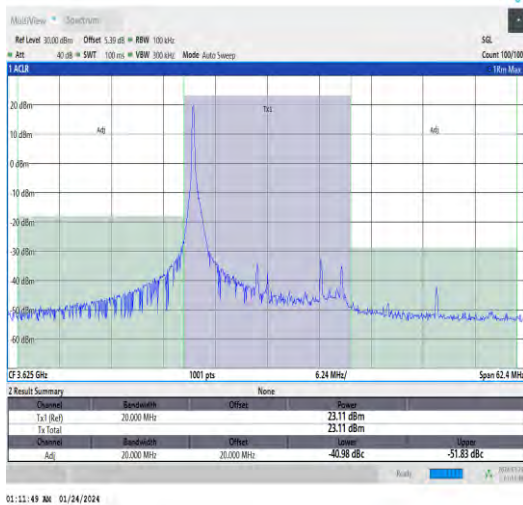
Band48-20MHz-QPSK-55990-1RB#0-PASS
