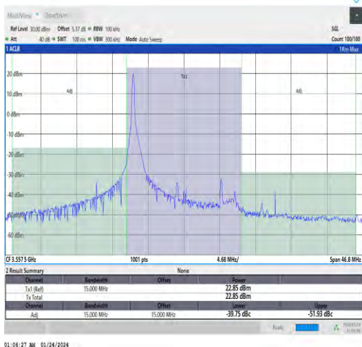
Band48-15MHz-QPSK-55315-1RB#0-PASS
