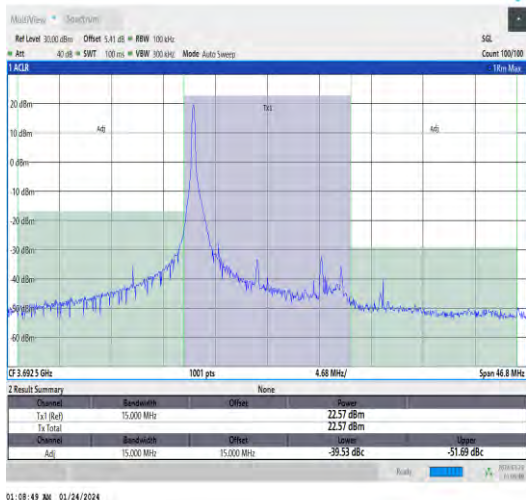
Band48-15MHz-QPSK-56665-1RB#0-PASS
