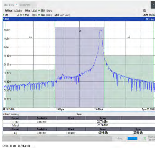
Band48-5MHz-QPSK-55990-1RB#24-PASS
