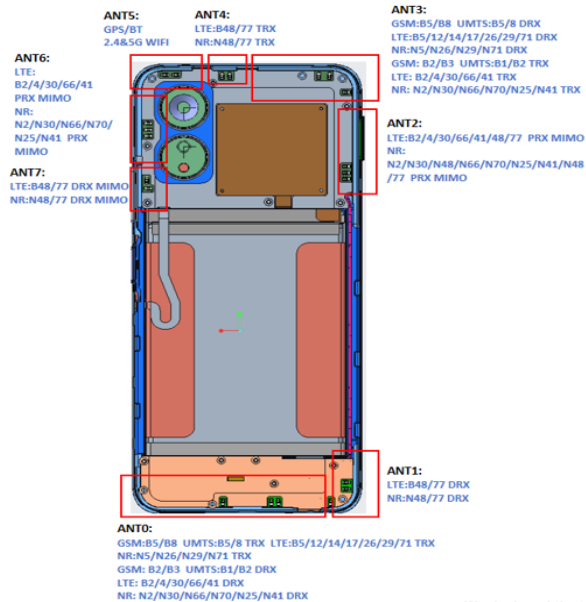
Photograph 15. Antenna position of EUT
