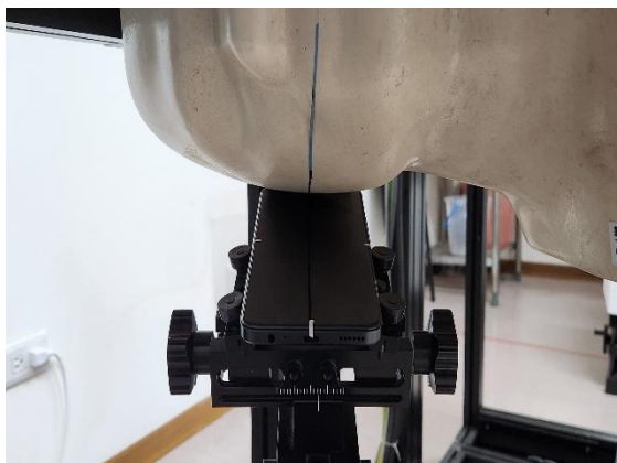
Photograph 9. Head, Right Tilt, 0mm
