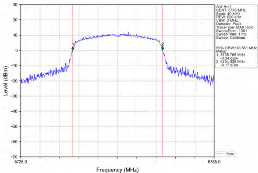
802.11ac(VHT20)_LCH_5745MHz_Ant1_NTNV
