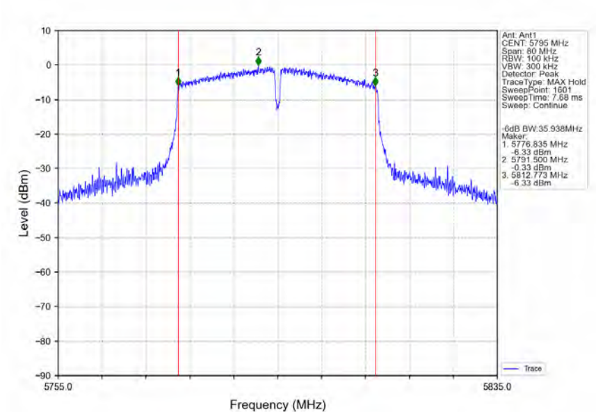
802.11ac(VHT40)_HCH_5795MHz_Ant1_NTNV
