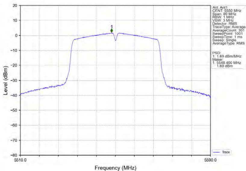
802.11ac(VHT40)_MCH_5550MHz_Ant1_NTNV
