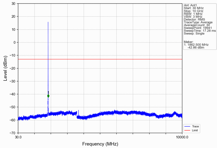
Band2_HSUPA_LCH_1852.4MHz_Subtest 1_NTNV
