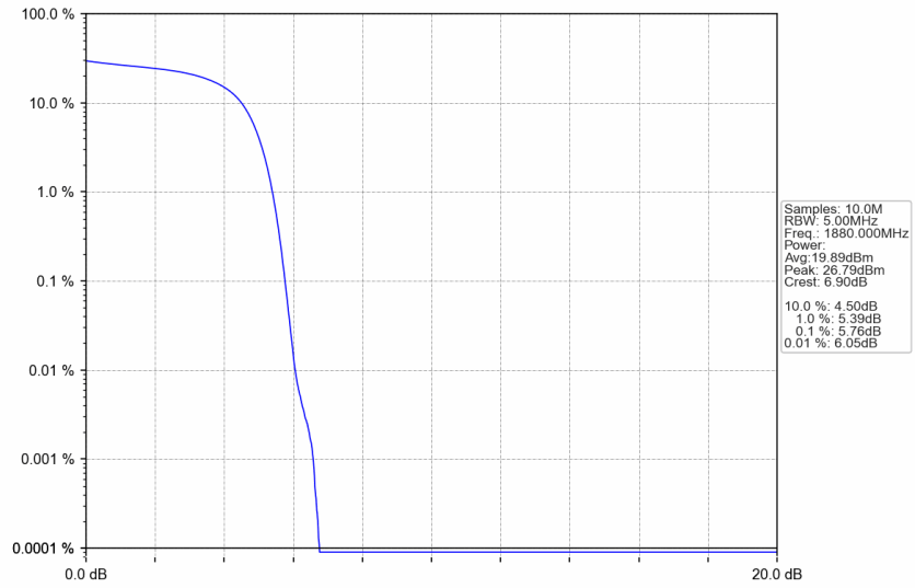
Band2_HSDPA_MCH_1880MHz_Subtest 1_NTNV
