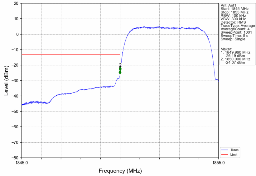
Band2_HSUPA_LCH_1852.4MHz_Subtest 1_NTNV
