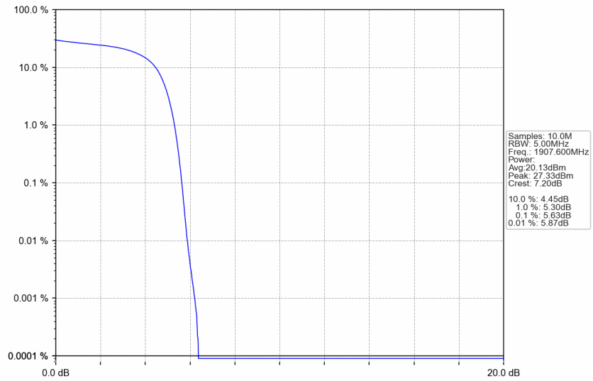
Band2_HSDPA_HCH_1907.6MHz_Subtest 1_NTNV
