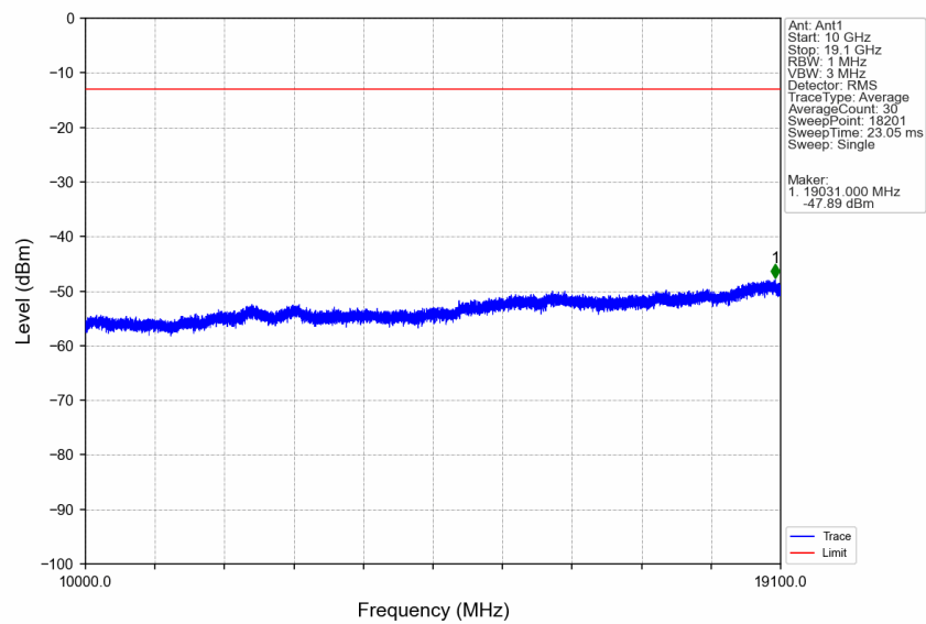
Band2_HSUPA_HCH_1907.6MHz_Subtest 1_NTNV
