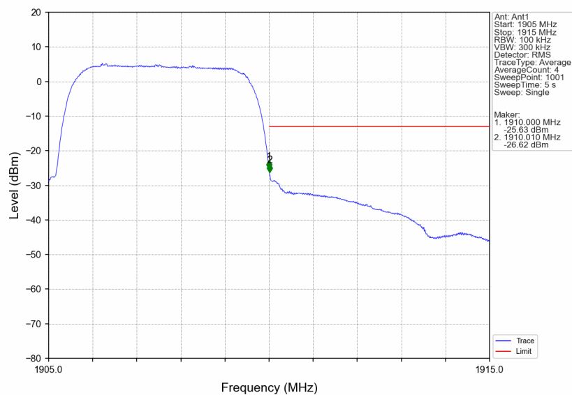
Band2_HSUPA_HCH_1907.6MHz_Subtest 1_NTNV
