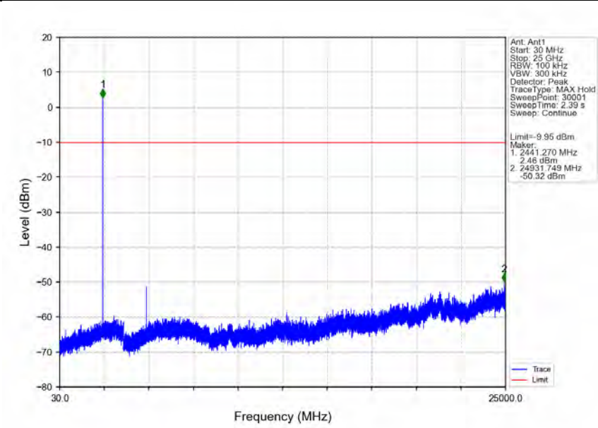
Pi/4DQPSK_2DH5_MCH_2441MHz_Ant1_NTNV
