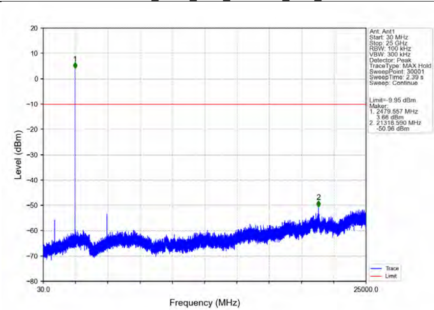
Pi/4DQPSK_2DH5_HCH_2480MHz_Ant1_NTNV
