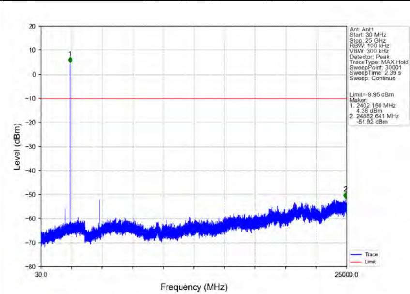
Pi/4DQPSK_2DH5_LCH_2402MHz_Ant1_NTNV
