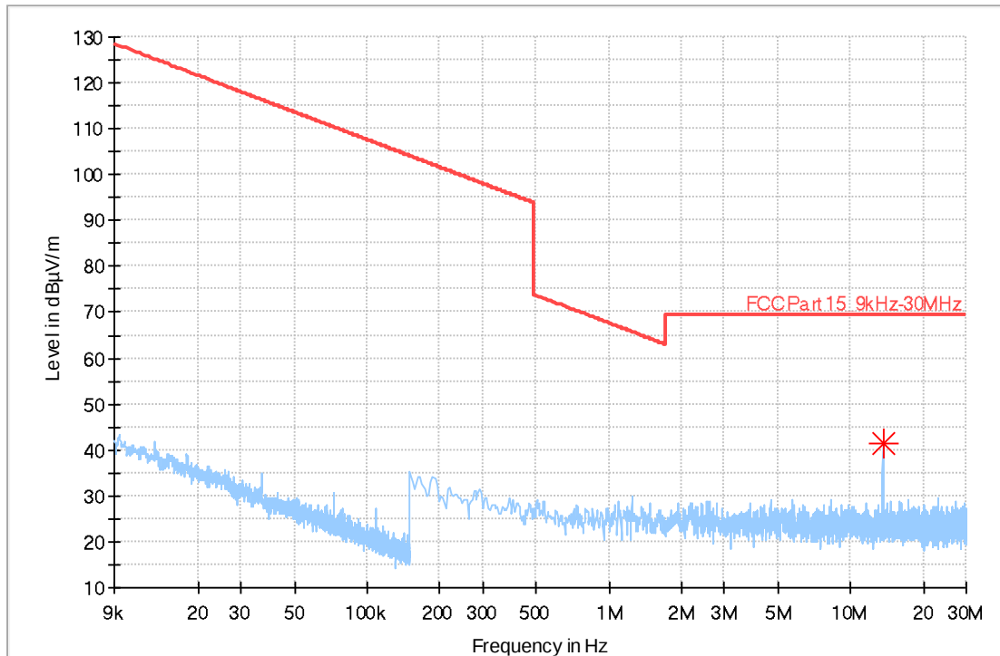
Figure B-4: Measurement results for Electric Field Radiated Emissions (&lt; 30MHz)
