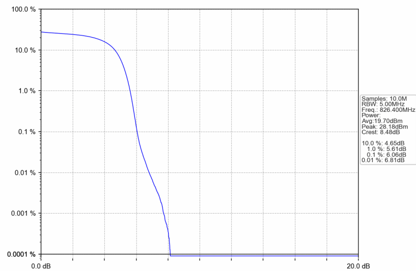
Band5_HSDPA_LCH_826.4MHz_Subtest 1_NTNV
