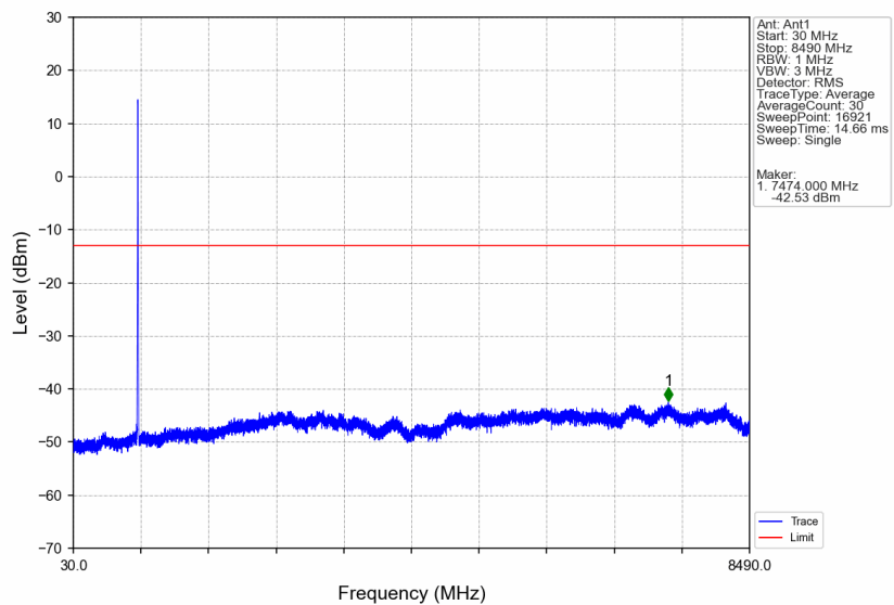
Band5_HSDPA_MCH_836.6MHz_Subtest 1_NTNV
