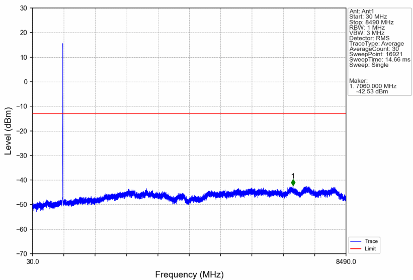
Band5_HSDPA_HCH_846.6MHz_Subtest 1_NTNV
