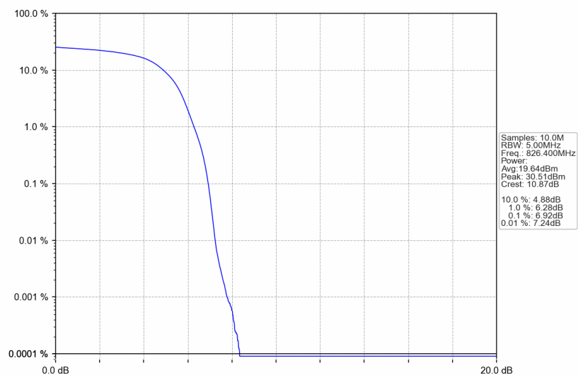
Band5_HSUPA_LCH_826.4MHz_Subtest 1_NTNV
