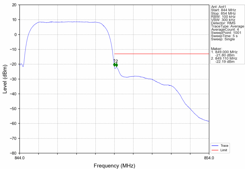
Band5_RMC_HCH_846.6MHz_12.2kbps RMC_NTNV
