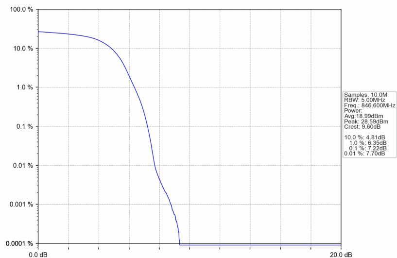
Band5_HSUPA_HCH_846.6MHz_Subtest 1_NTNV
