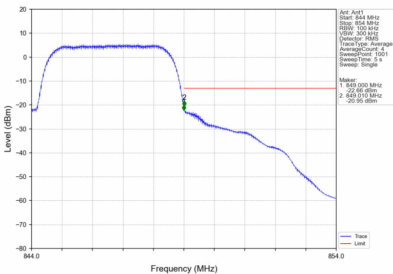
Band5_HSDPA_HCH_846.6MHz_Subtest 1_NTNV
