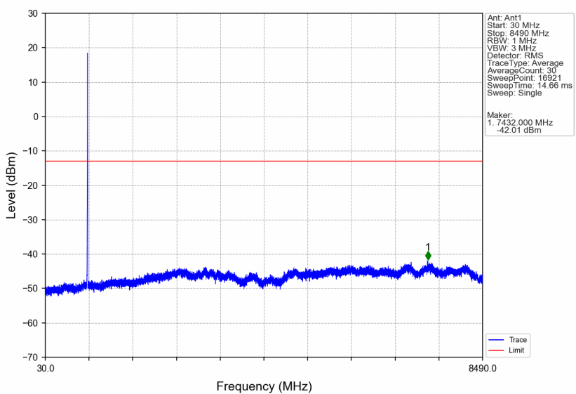
Band5_HSDPA_LCH_826.4MHz_Subtest 1_NTNV
