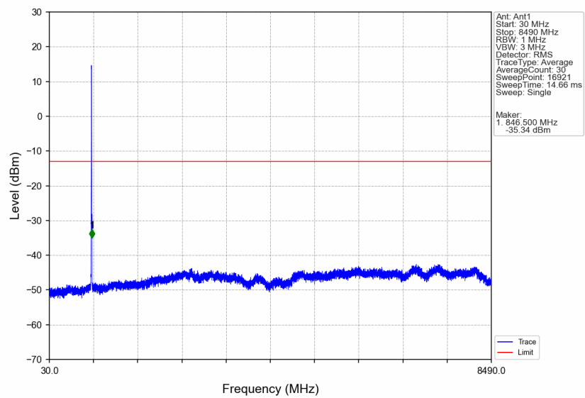
Band5_HSUPA_HCH_846.6MHz_Subtest 1_NTNV
