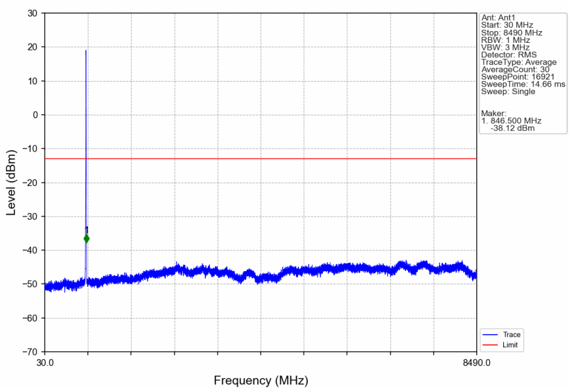
Band5_RMC_HCH_846.6MHz_12.2kbps RMC_NTNV
