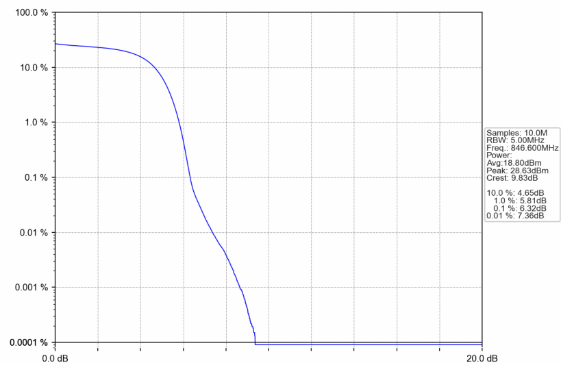
Band5_HSDPA_HCH_846.6MHz_Subtest 1_NTNV
