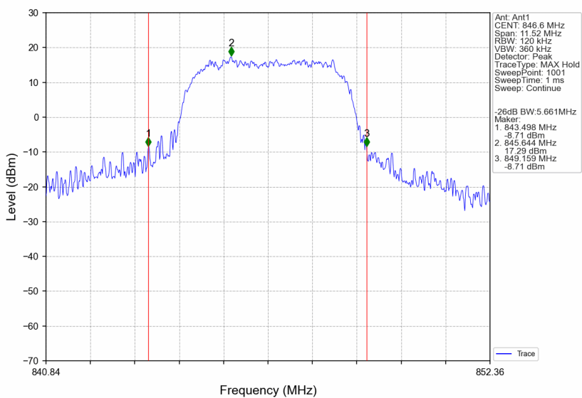
Band5_HSDPA_HCH_846.6MHz_Subtest 1_NTNV
