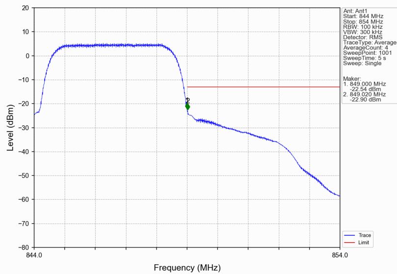
Band5_HSUPA_HCH_846.6MHz_Subtest 1_NTNV
