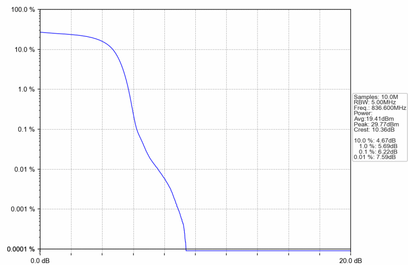
Band5_HSDPA_MCH_836.6MHz_Subtest 1_NTNV
