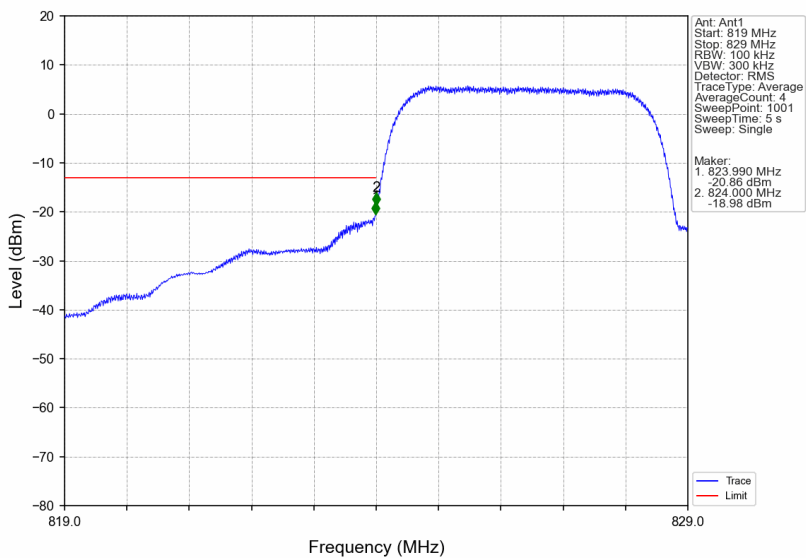
Band5_HSDPA_LCH_826.4MHz_Subtest 1_NTNV
