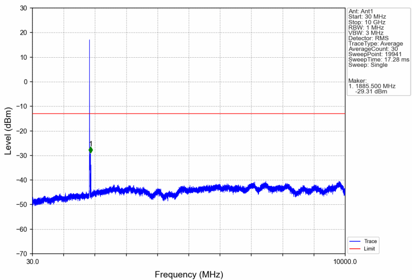
Band2_HSUPA_LCH_1852.4MHz_Subtest 1_NTNV
