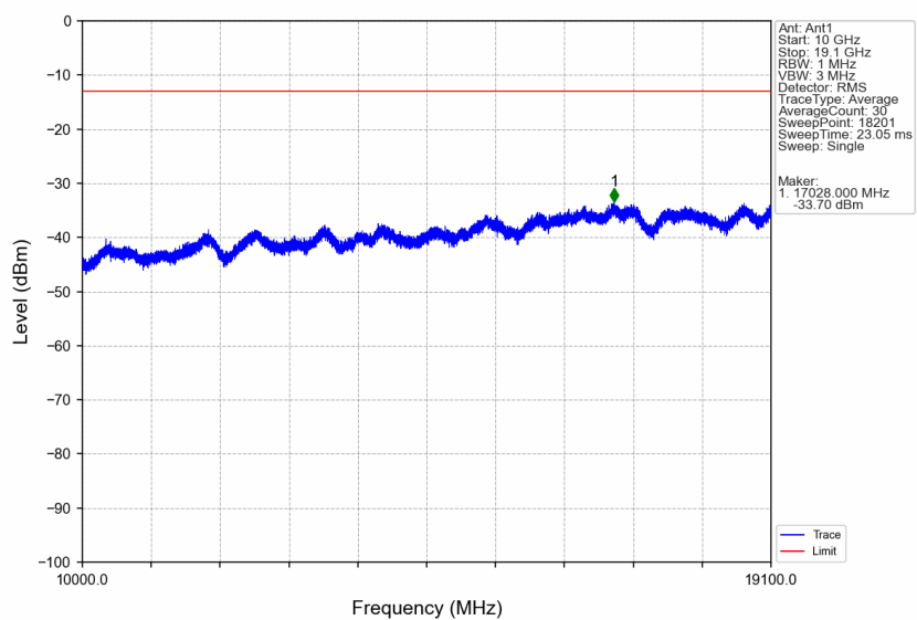
Band2_RMC_MCH_1880MHz_12.2kbps RMC_NTNV
