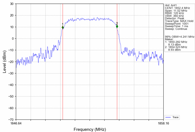
Band2_HSDPA_LCH_1852.4MHz_Subtest 1_NTNV
