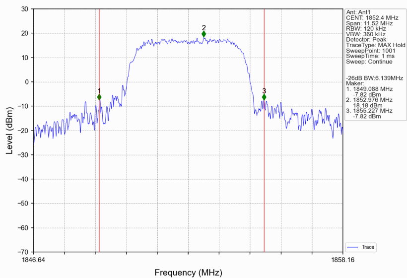
Band2_HSDPA_LCH_1852.4MHz_Subtest 1_NTNV
