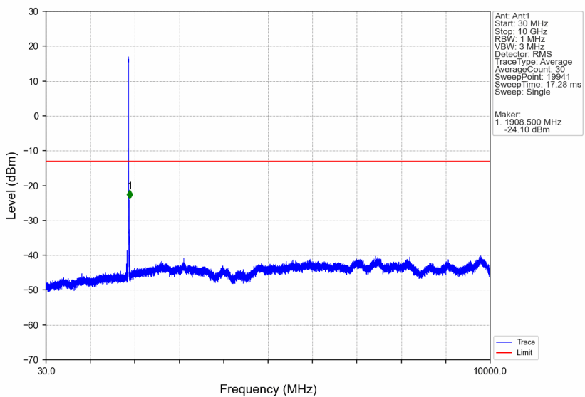
Band2_HSDPA_MCH_1880MHz_Subtest 1_NTNV
