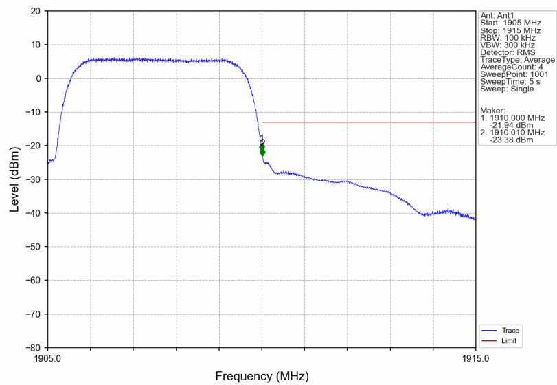
Band2_HSUPA_HCH_1907.6MHz_Subtest 1_NTNV
