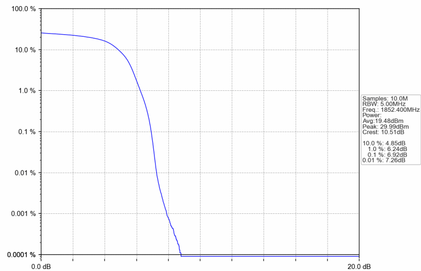
Band2_HSUPA_LCH_1852.4MHz_Subtest 1_NTNV
