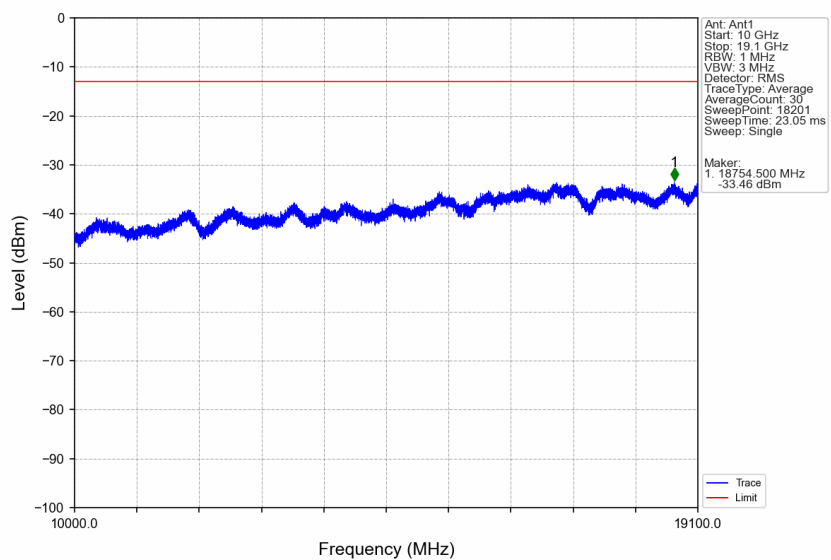
Band2_HSUPA_HCH_1907.6MHz_Subtest 1_NTNV
