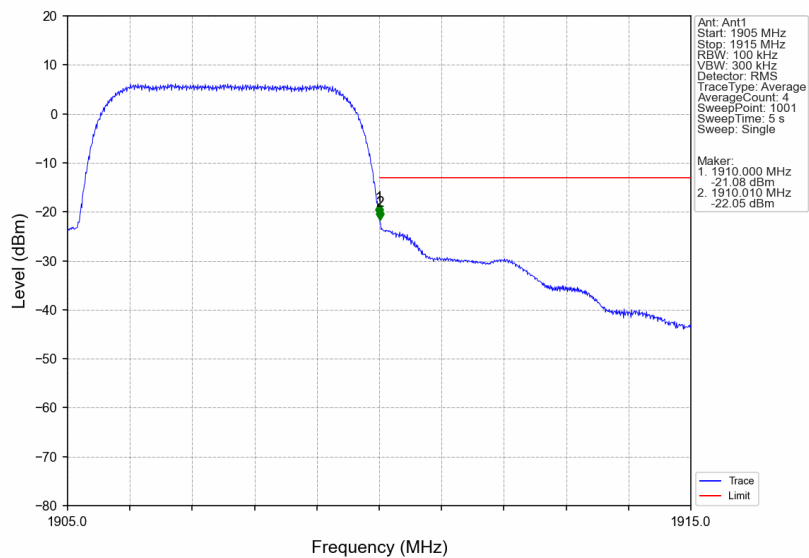
Band2_HSDPA_HCH_1907.6MHz_Subtest 1_NTNV
