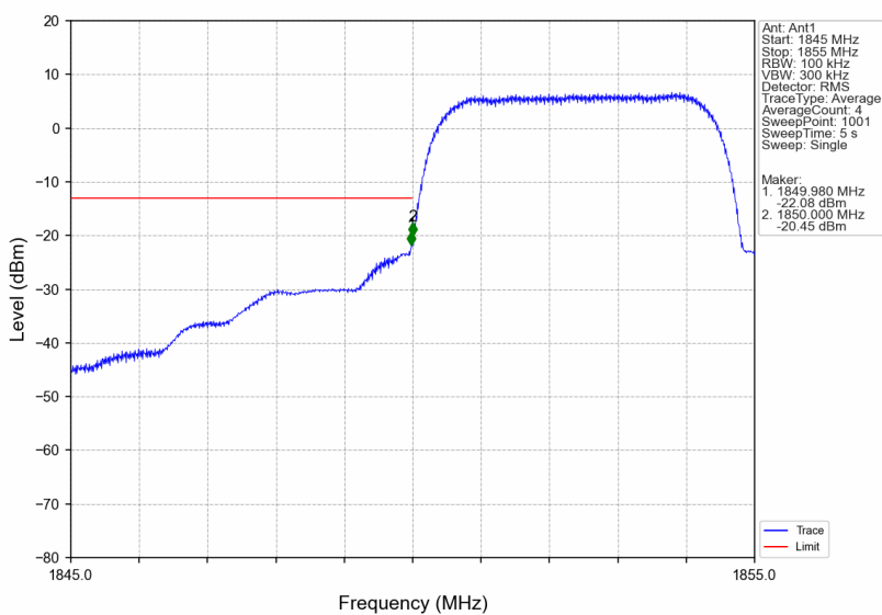
Band2_HSDPA_LCH_1852.4MHz_Subtest 1_NTNV
