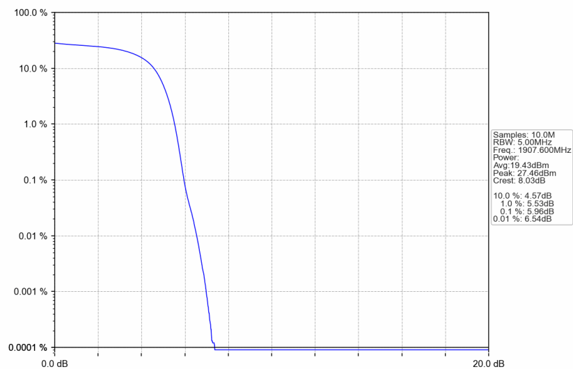
Band2_HSDPA_HCH_1907.6MHz_Subtest 1_NTNV
