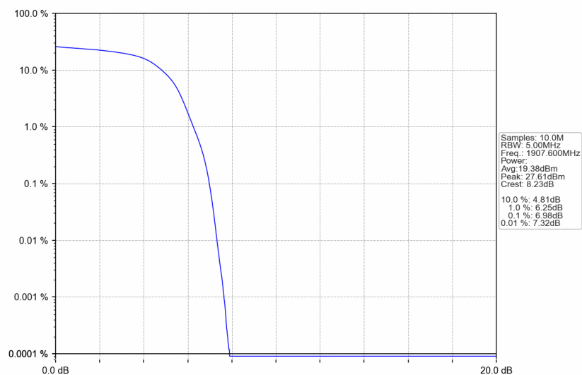
Band2_HSUPA_HCH_1907.6MHz_Subtest 1_NTNV
