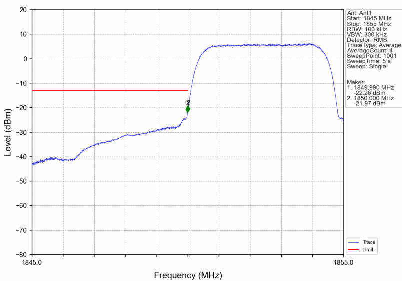
Band2_HSUPA_LCH_1852.4MHz_Subtest 1_NTNV
