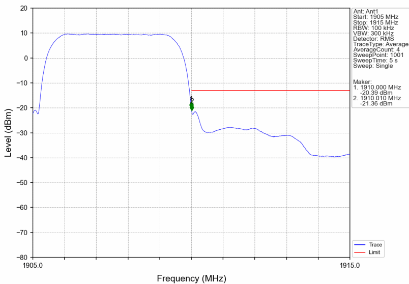
Band2_RMC_HCH_1907.6MHz_12.2kbps RMC_NTNV
