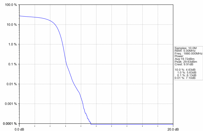
Band2_HSDPA_MCH_1880MHz_Subtest 1_NTNV
