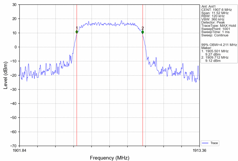
Band2_HSDPA_HCH_1907.6MHz_Subtest 1_NTNV
