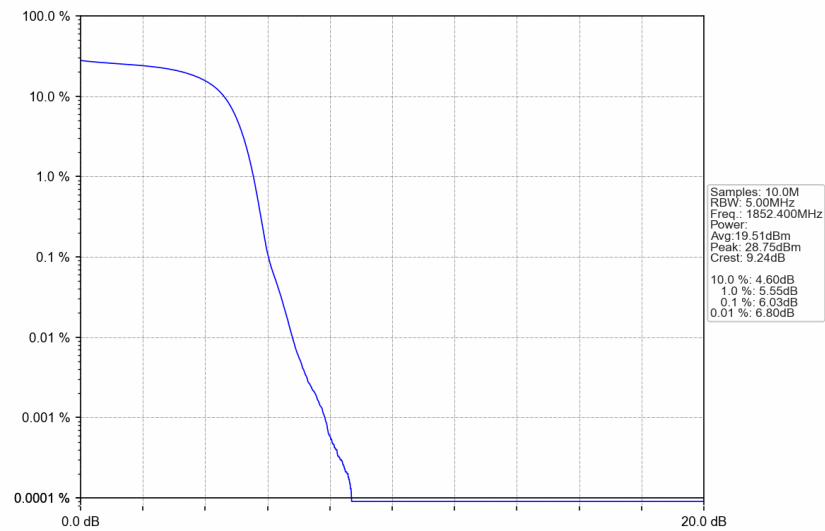
Band2_HSDPA_LCH_1852.4MHz_Subtest 1_NTNV
