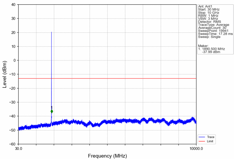
Band2_RMC_MCH_1880MHz_12.2kbps RMC_NTNV
