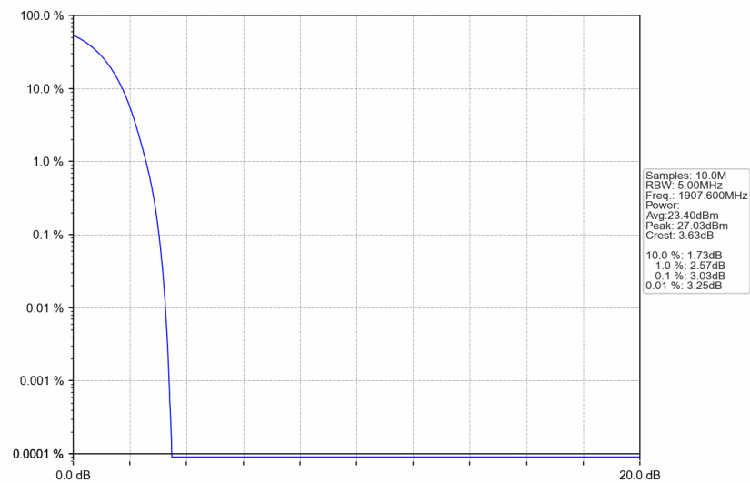
Band2_RMC_HCH_1907.6MHz_12.2kbps RMC_NTNV
