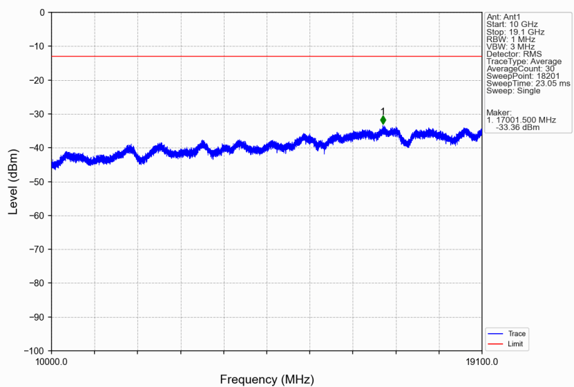
Band2_HSDPA_HCH_1907.6MHz_Subtest 1_NTNV
