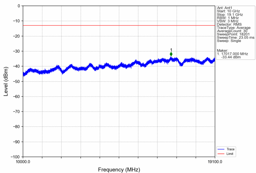
Band2_HSDPA_MCH_1880MHz_Subtest 1_NTNV
