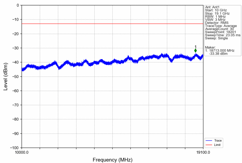
Band2_RMC_HCH_1907.6MHz_12.2kbps RMC_NTNV
