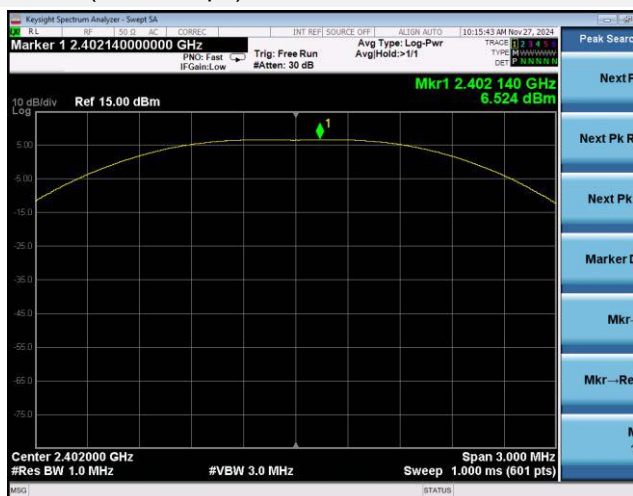
GFSK (BLE 1Mbps) LOW CHANNEL
