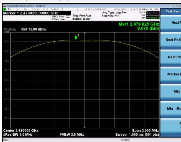
GFSK (BLE 1Mbps) HIGH CHANNEL
