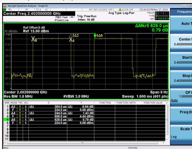
GFSK (BLE 1Mbps)
