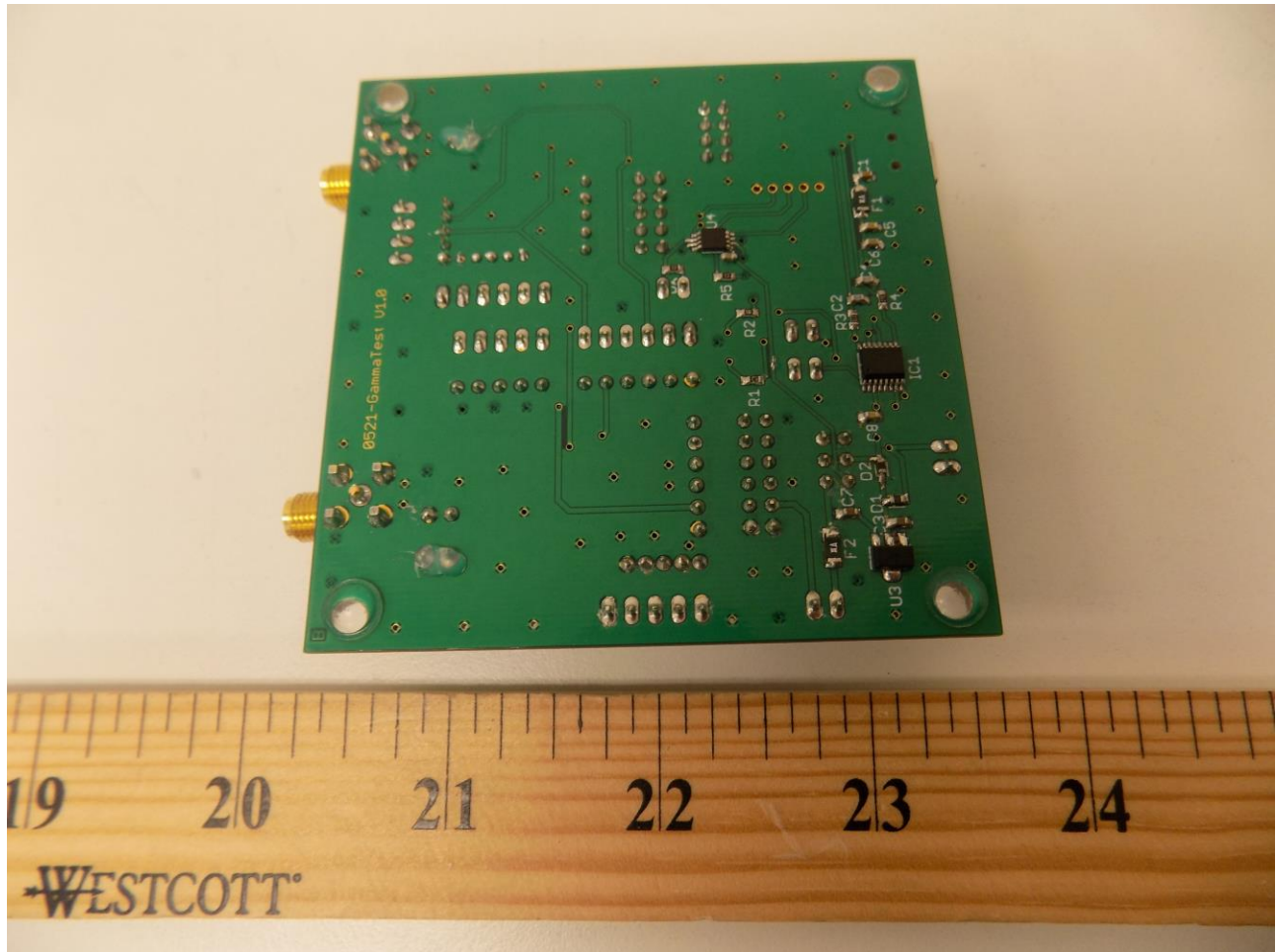
Figure 4 - External Photo of EUT development board - Rear View
