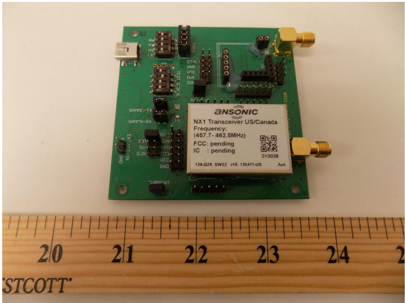
Figure 3 - External Photo of EUT development board- Front View
