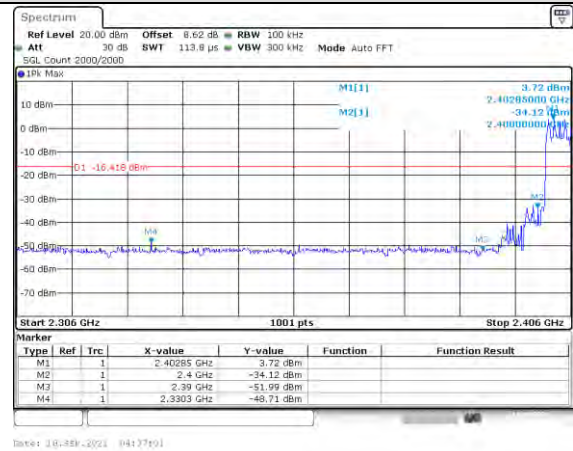
Hopping mode
