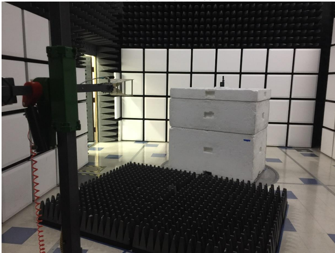
Front view – 1GHz – 18GHz
