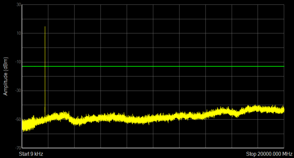
Band66 16QAM BW=3MHz Channel=132657 RB Size=1 Position=#0
