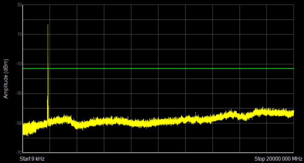
Band25 16QAM BW=20MHz Channel=26365 RB Size=1 Position=#0
