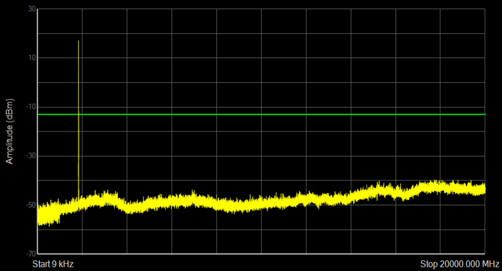
Band25 16QAM BW=5MHz Channel=26065 RB Size=1 Position=#0
