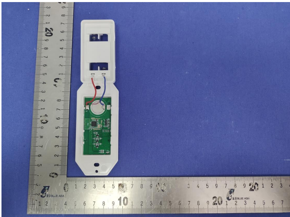
Series model:WP1025A.A0
