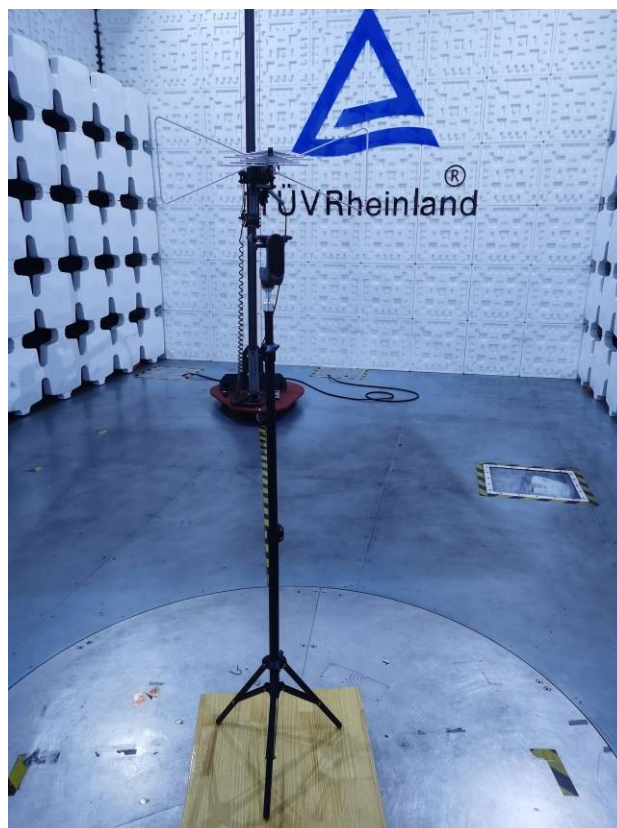
Photograph 1: Set-up photo for Radiated Emissions Below 1GHz
