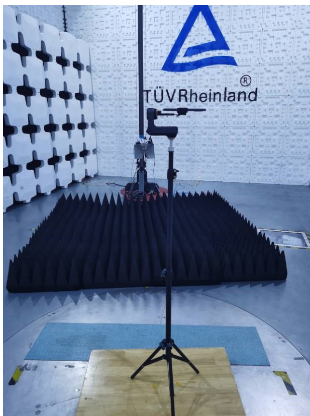
Photograph 2: Set-up photo for Radiated Emissions Above 1GHz
