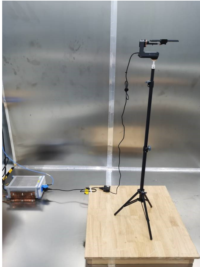
Photograph 3: Set-up photo for Conducted Emission on AC Mains
