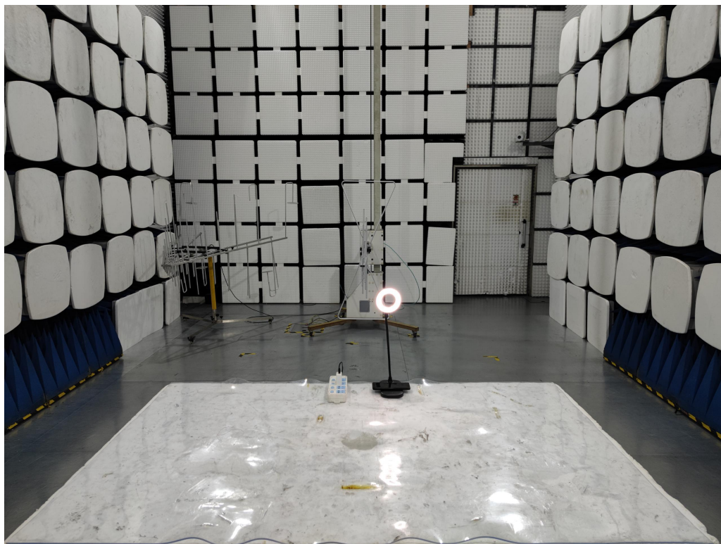
Radiated Emission 30MHz-1GHz-DC adapter charge mode
