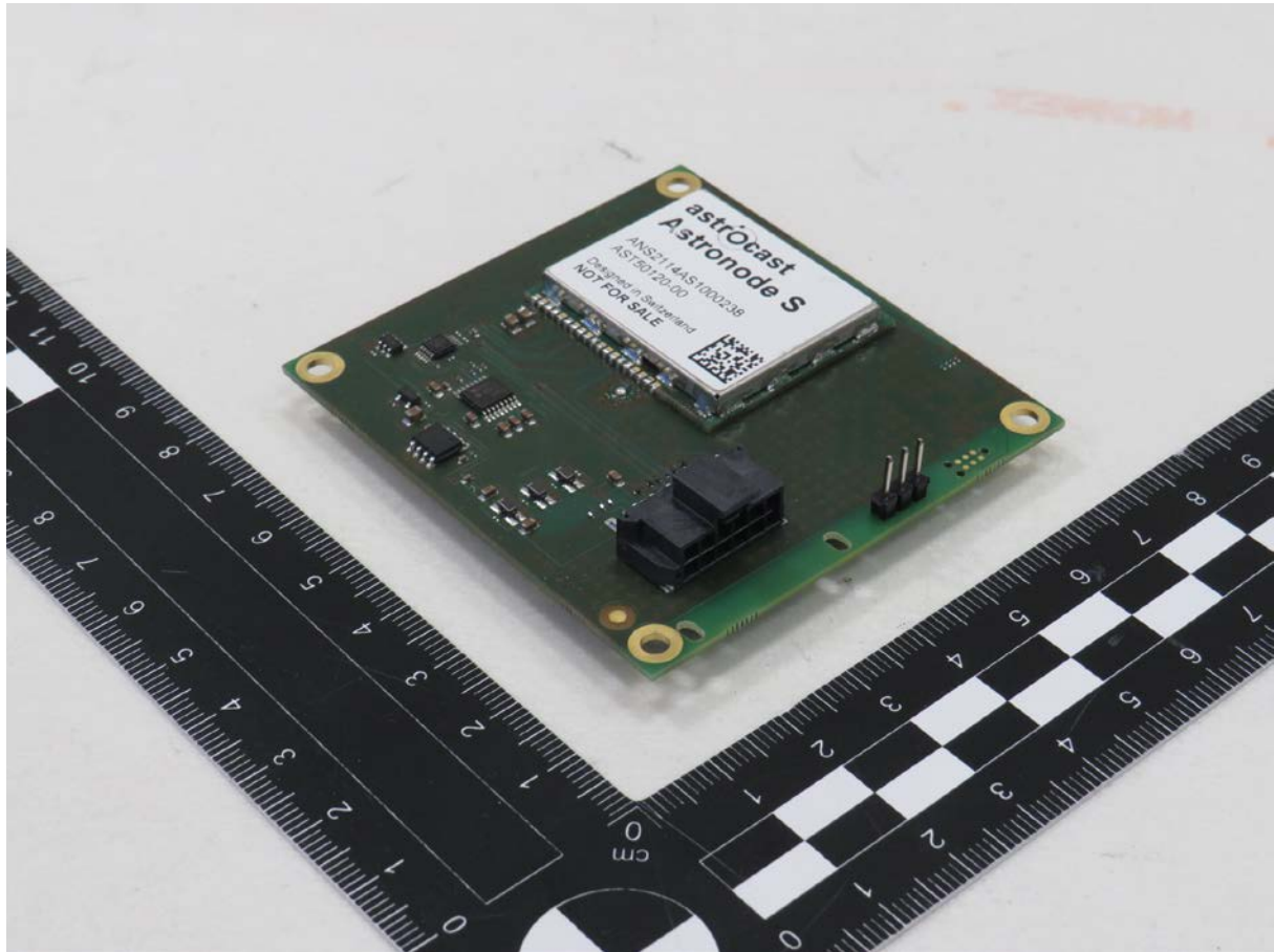
Astronoe S – Top on Evaluation Board
