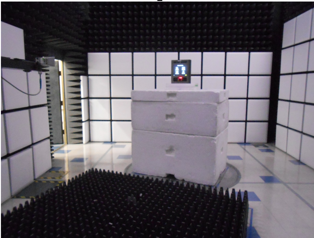
Radiated RF_18 - 25 GHz
