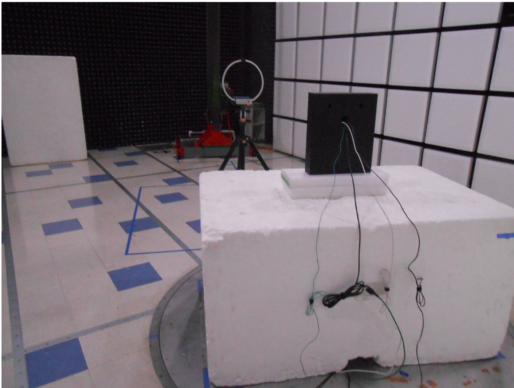
Radiated RF – 100 kHz – 30 MHz
