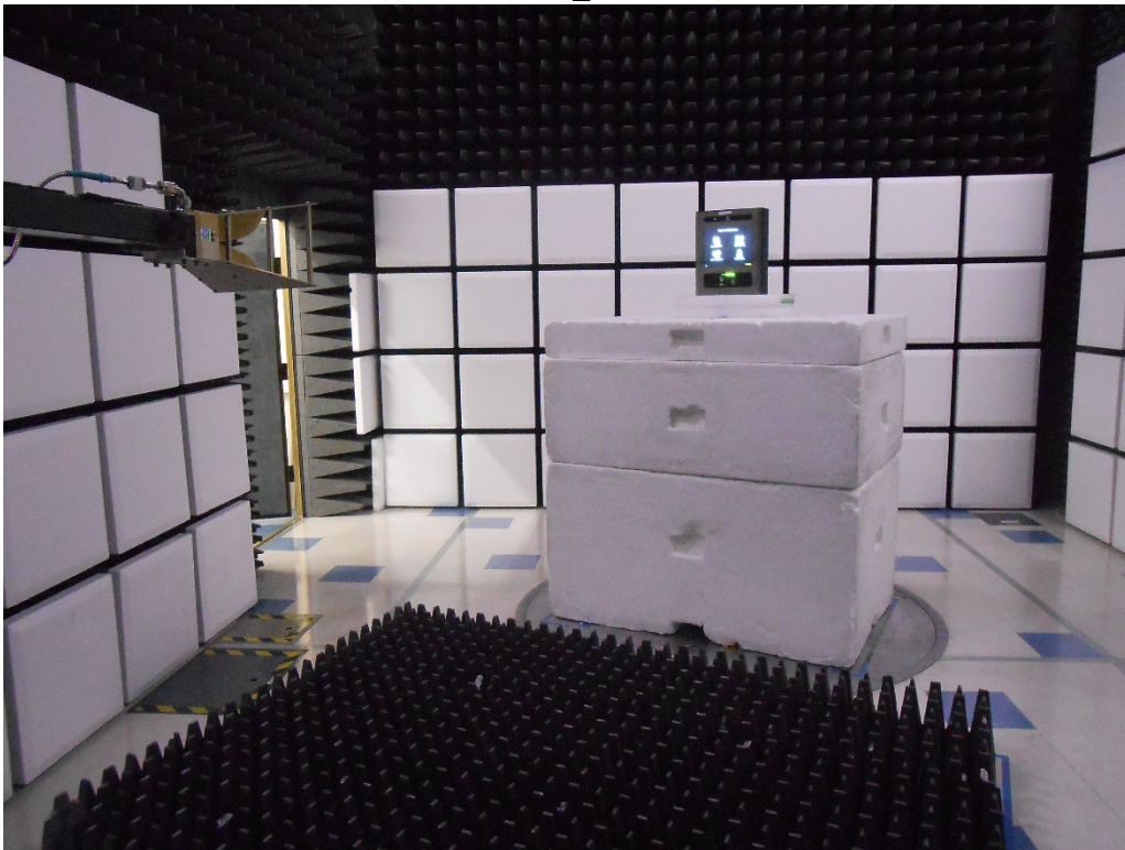
Radiated RF_1 - 18 GHz
