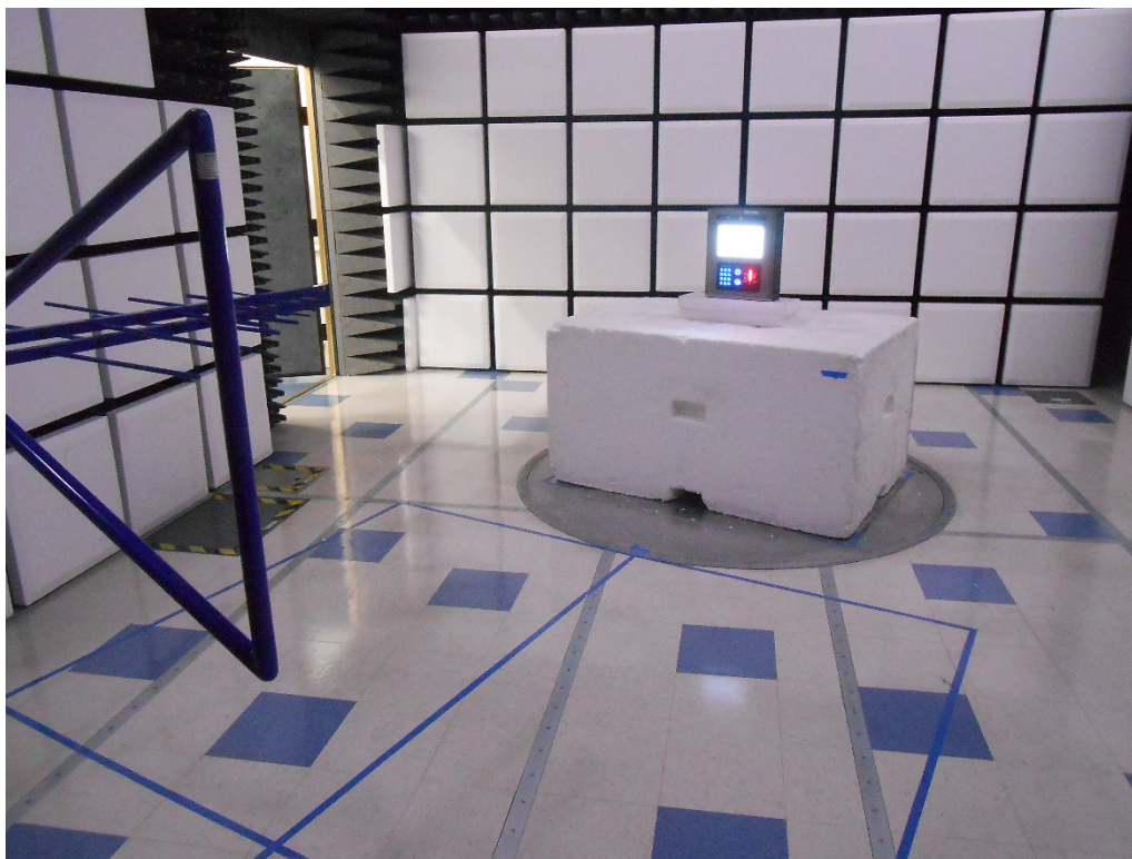
Radiated RF – 30 – 1000 MHz
