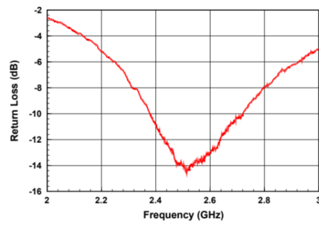
Return Loss: Antenna 1
