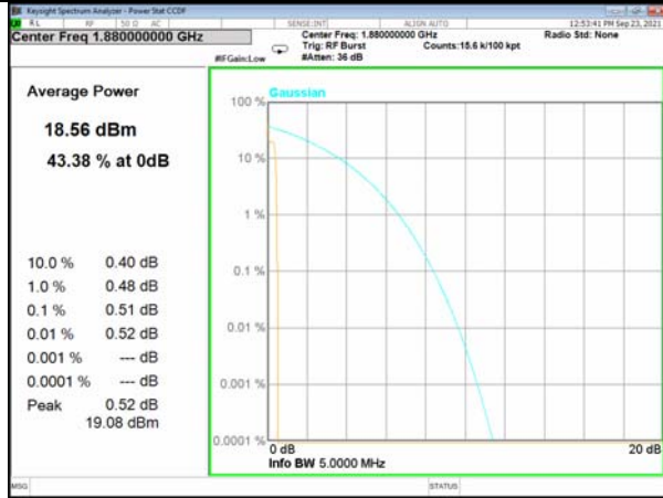
Band 2-3.75KHz-1#47-BPSK-Mid
