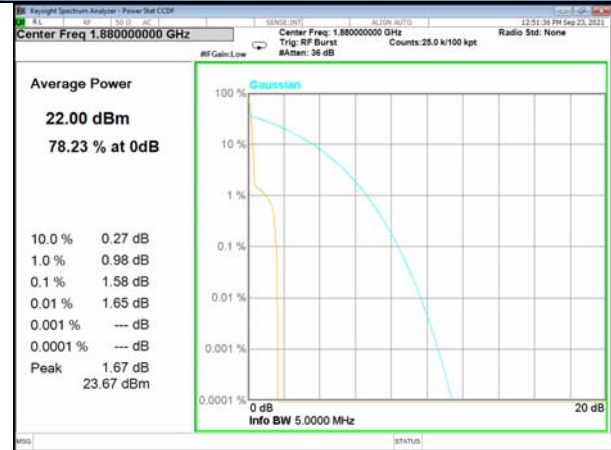
Band 2-15KHz-1#0-QPSK-Mid
