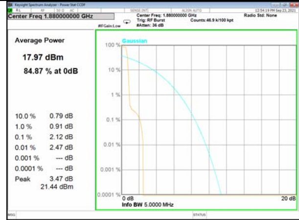
Band 2-3.75KHz-1#47-QPSK-Mid
