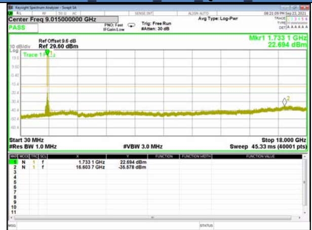
Band 4_3.75KHz_1#47_QPSK_High
