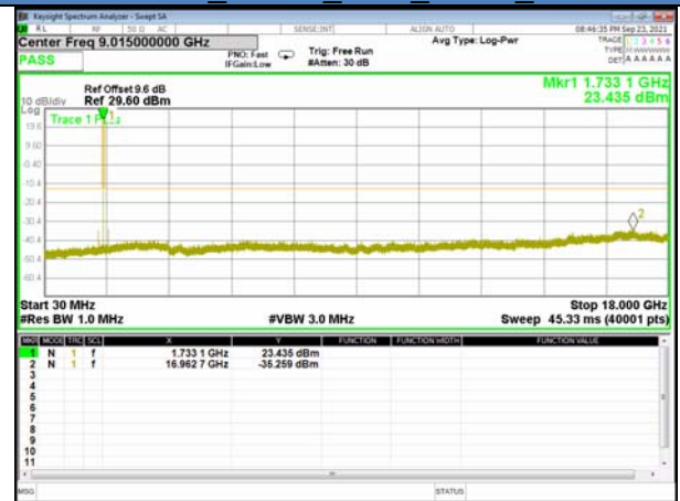
Band 4_15KHz_1#11_BPSK_High
