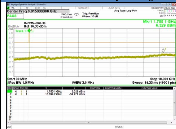
Band 4_3.75KHz_1#0_QPSK_High
