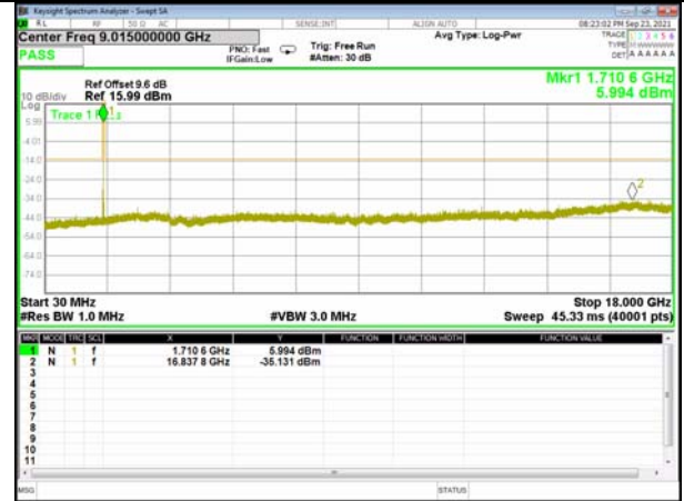
Band 4_3.75KHz_1#47_QPSK_Mid
