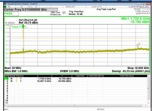
Band 4_3.75KHz_1#47_QPSK_High
