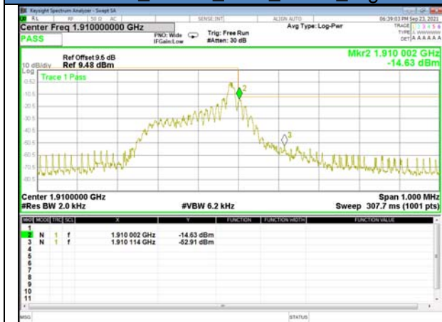
Band 2_15KHz_12#0_QPSK_High
