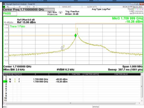
Band 66_3.75KHz_1#47_QPSK_High
