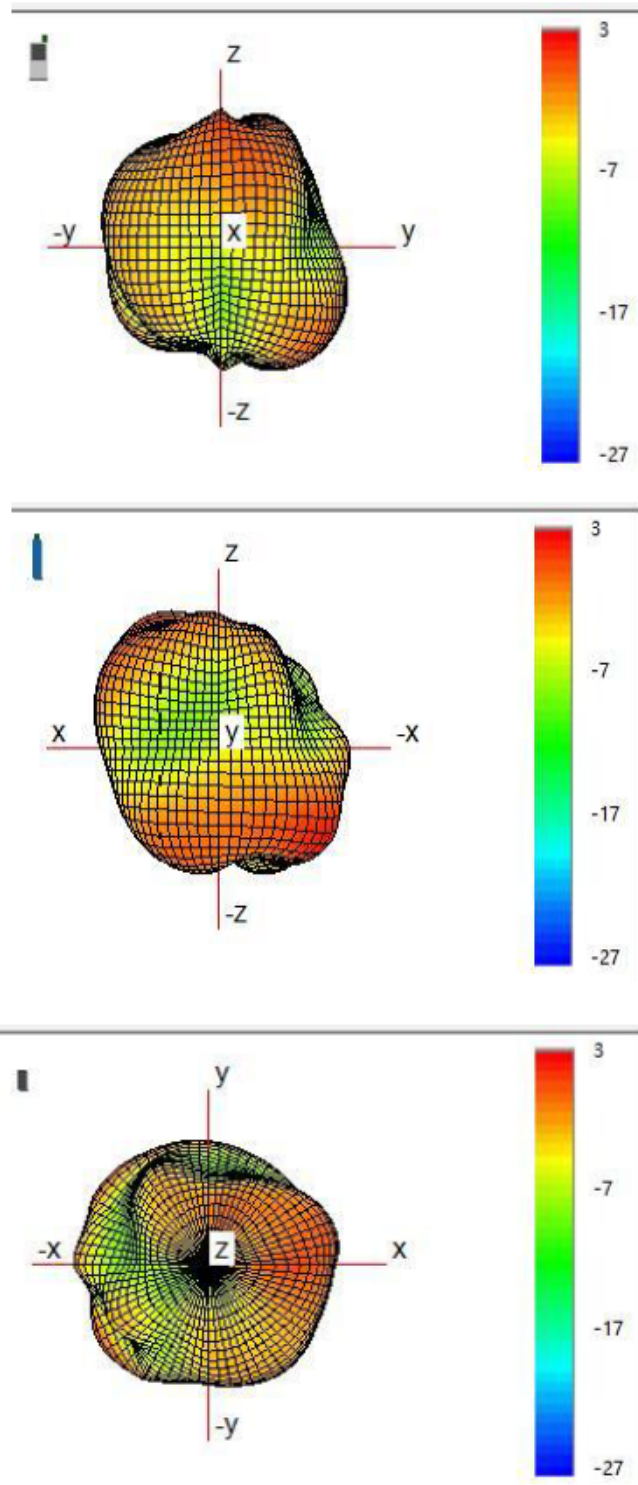
3D Gain Pattern @ 2450 MHz Unit: dBi
