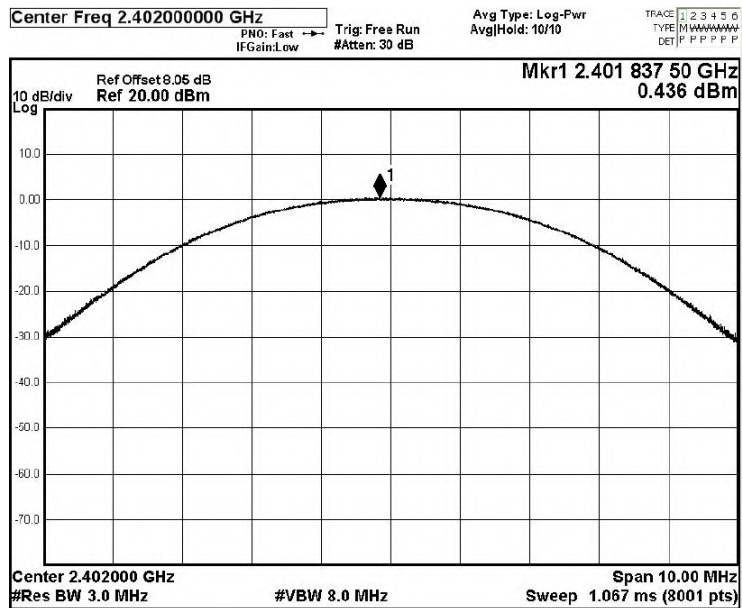
Test Mode: 8DPSK---Low
