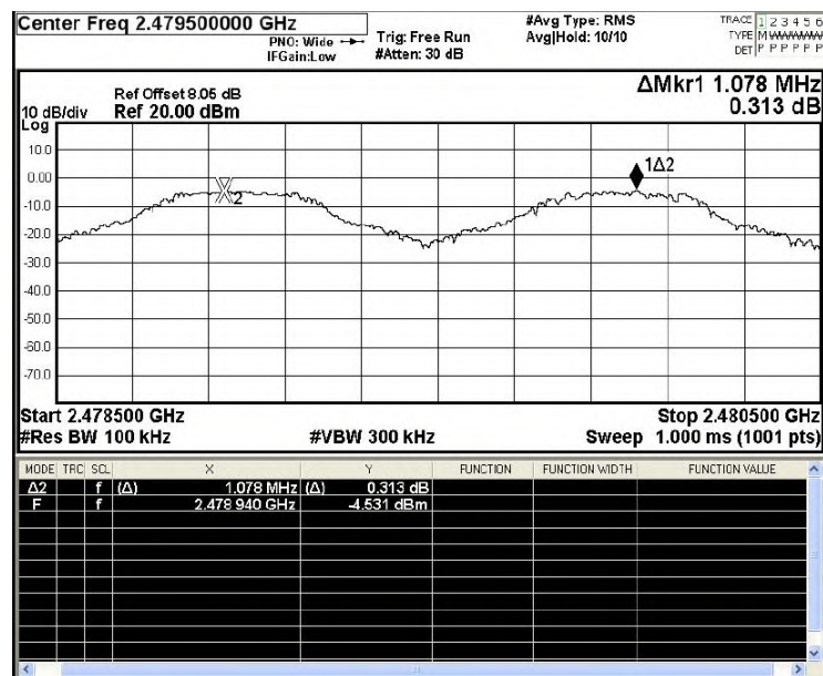
Test Mode: GFSK ---High
