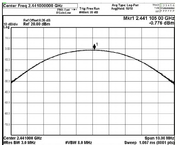
Test Mode: 8DPSK ---Middle
