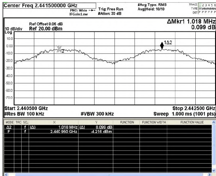
Test Mode: GFSK ---Middle
