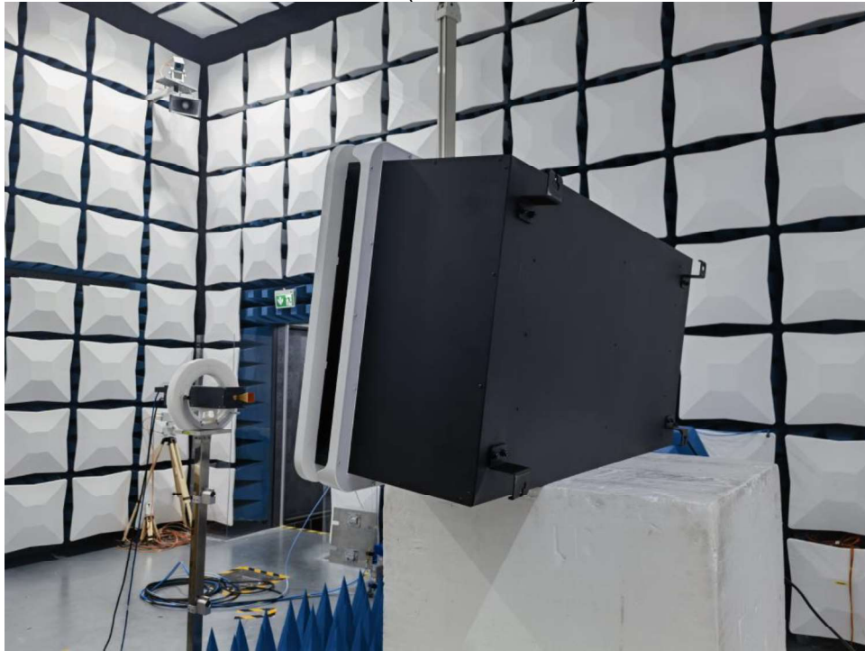
Radiated Emission (Above 40 GHz) – EUT B
