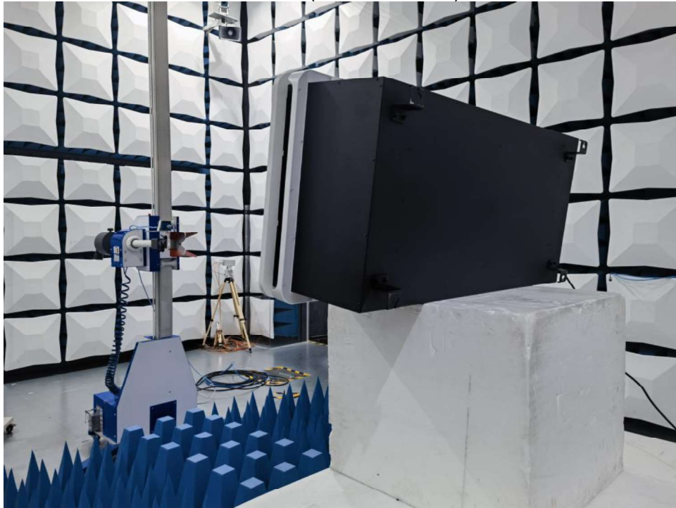
Radiated Emission (1 GHz – 40 GHz) – EUT B
