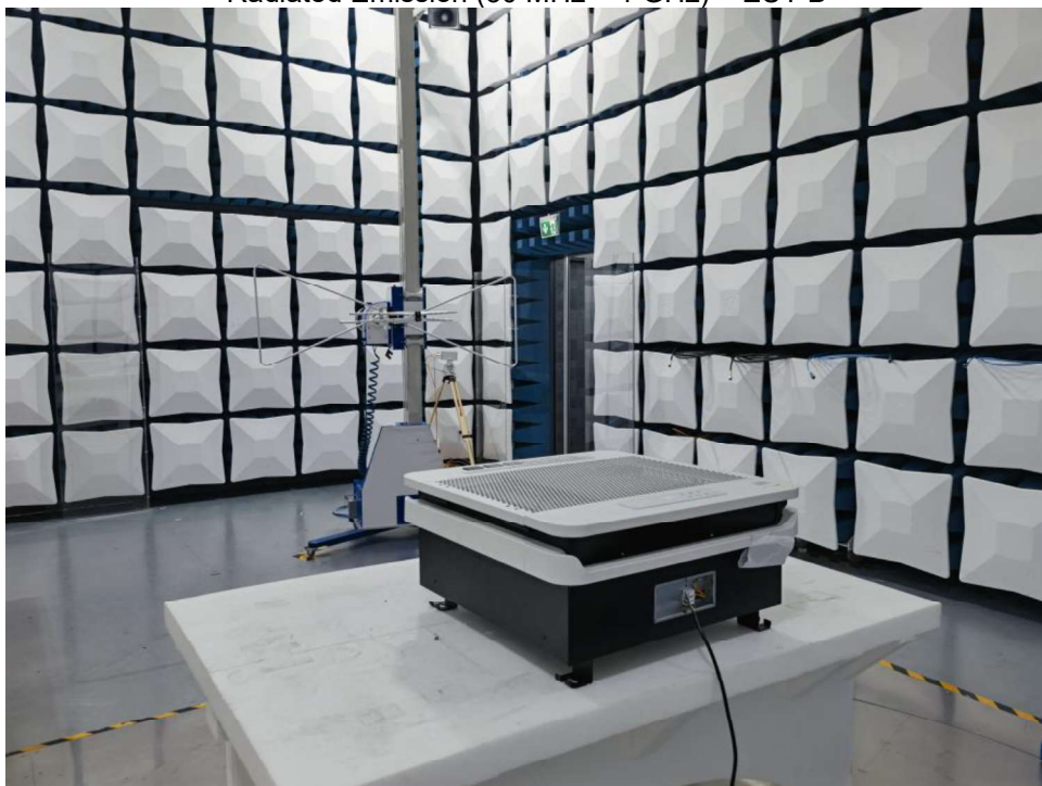
Radiated Emission (30 MHz – 1 GHz) – EUT B
