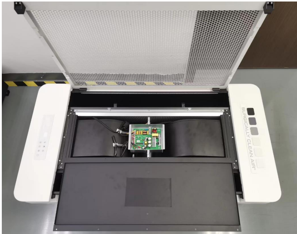
Figure 27: Internal view of SCA14000-2x4
