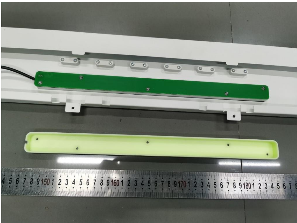
Figure 10: Internal view of SCA14000-2x2
