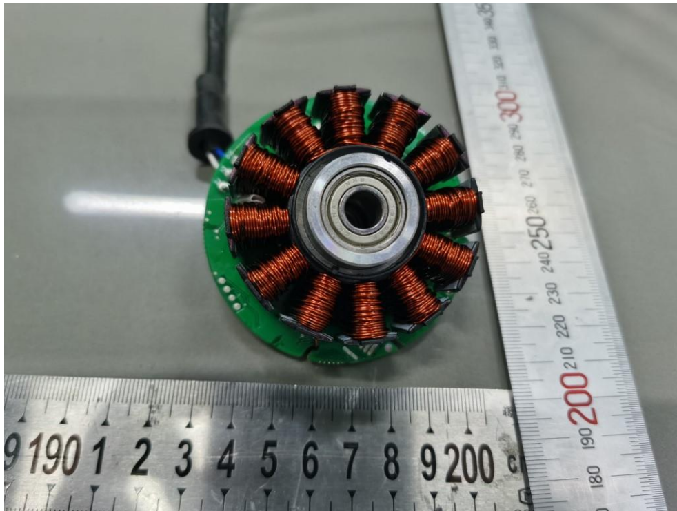
Figure 23: Motor of SCA14000-2x2
