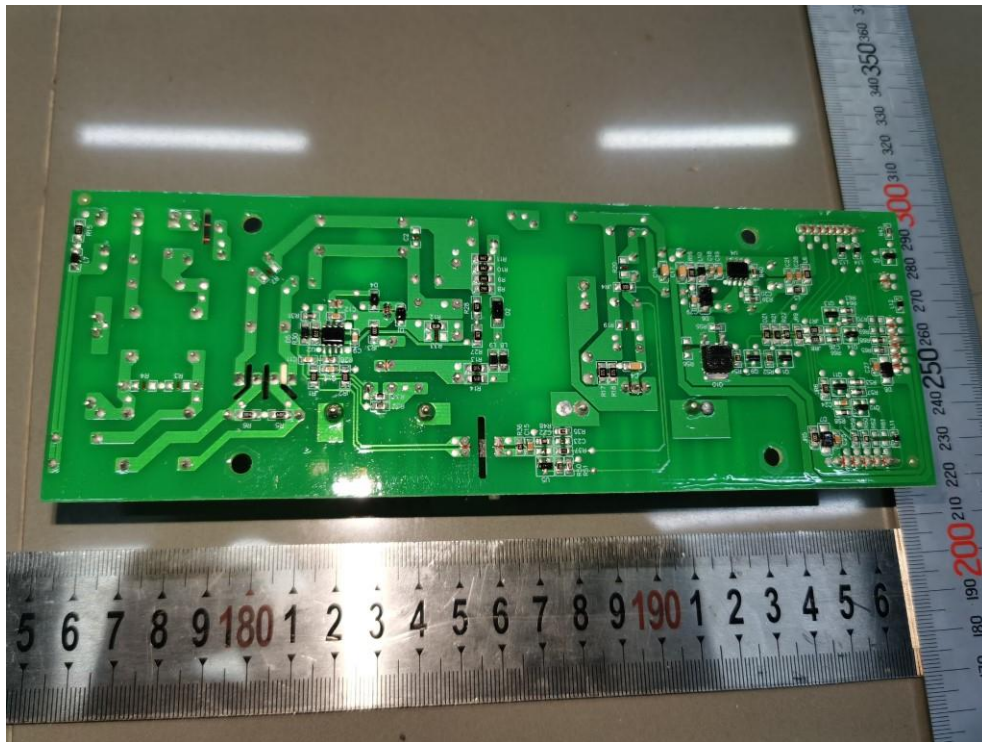
Figure 17: Power PCB of SCA14000-2x2
