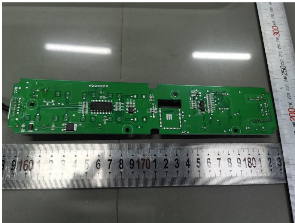
Figure 34: Main PCB of SCA14000-2x2 & SCA14000-2x4
