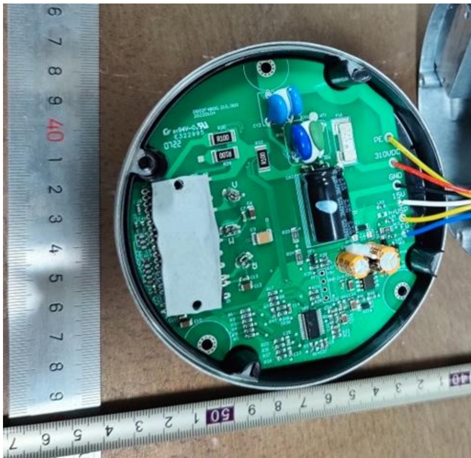
Figure 44: Motor of SCA14000-2x4
