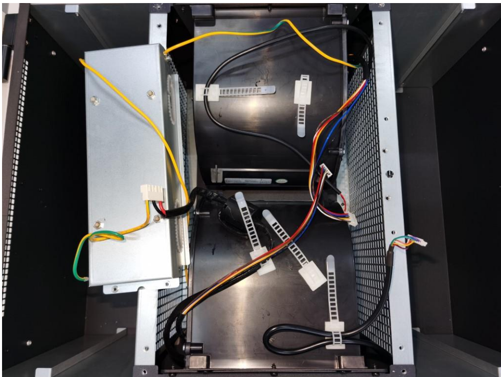
Figure 14: Internal view of SCA14000-2x2
