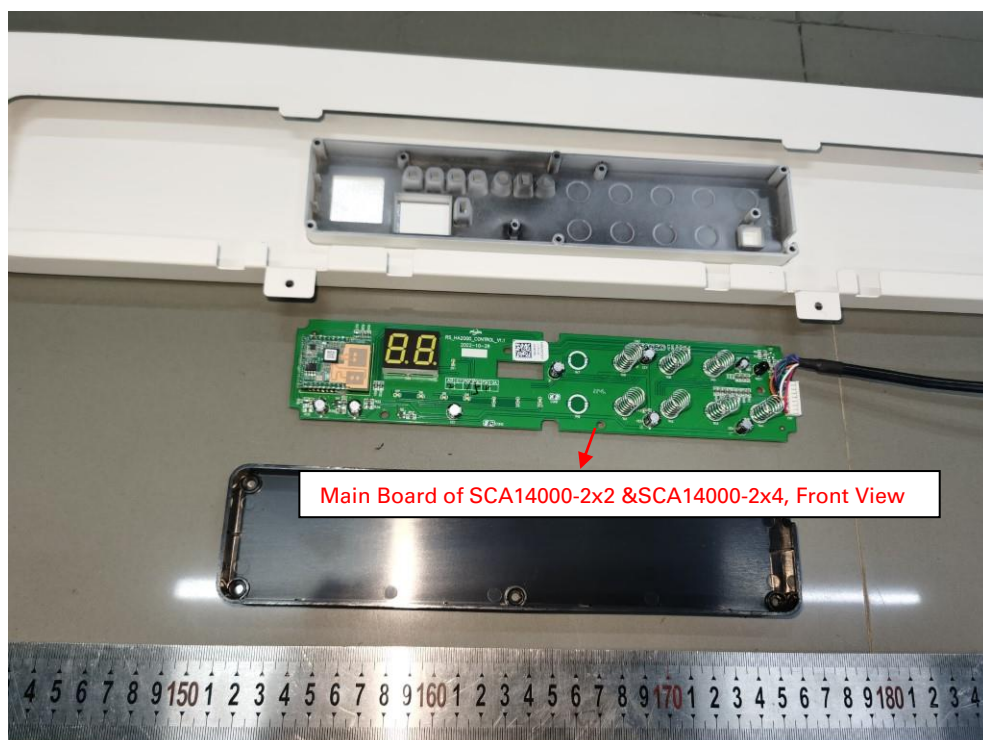
Figure 6: Internal view of SCA14000-2x2
