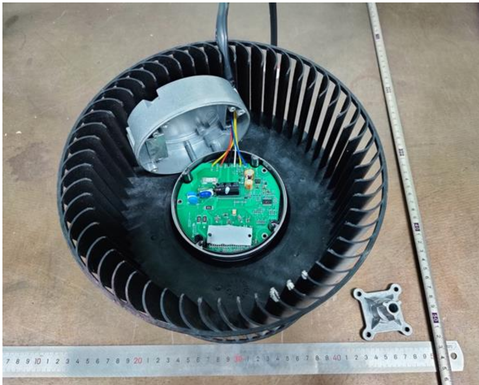
Figure 41: Motor of SCA14000-2x4
