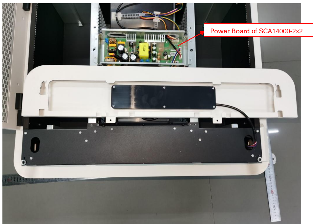
Figure 4: Internal view of SCA14000-2x2
