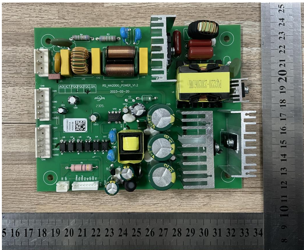
Figure 30: Power PCB of SCA14000-2x4
