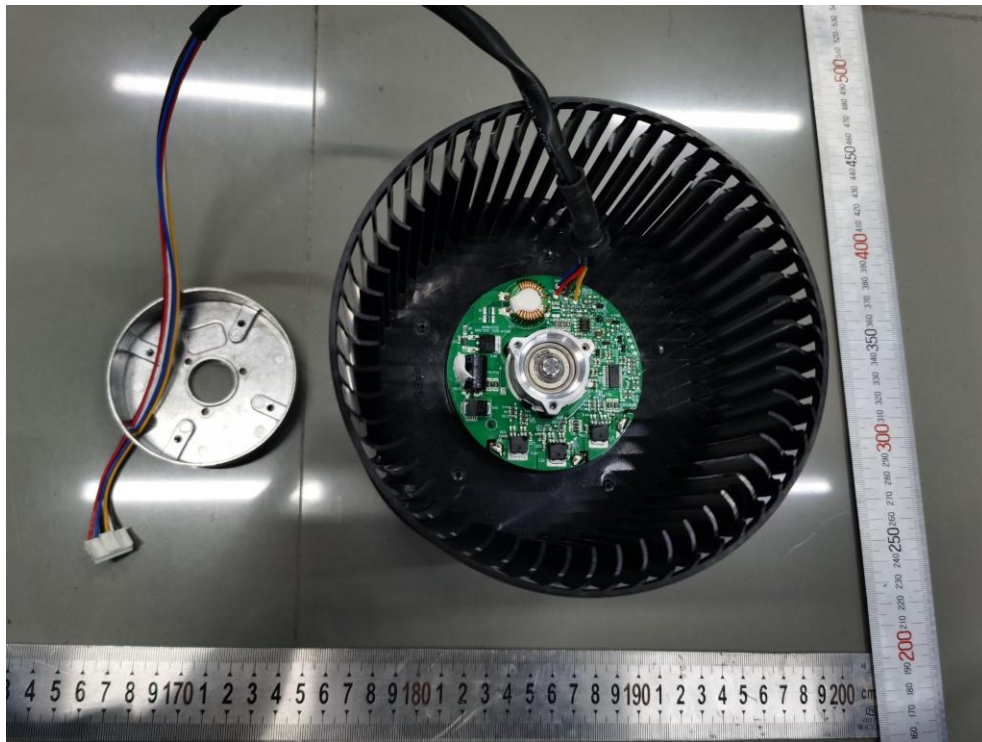
Figure 21: Motor of SCA14000-2x2
