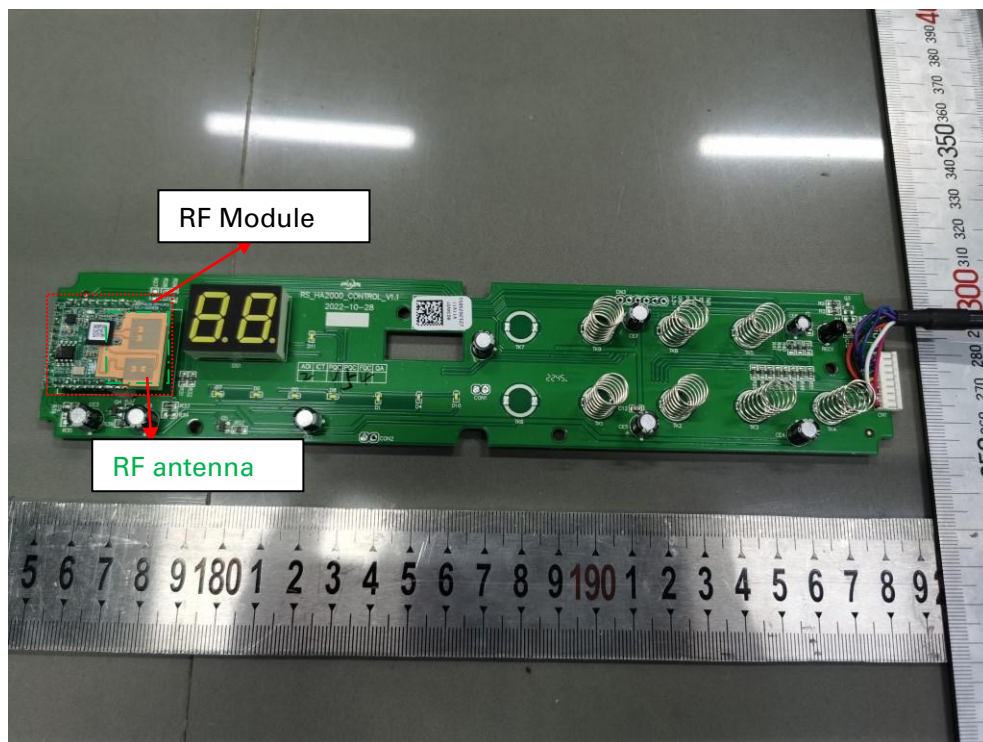
Figure 7: Main PCB of SCA14000-2x2 & SCA14000-2x4
