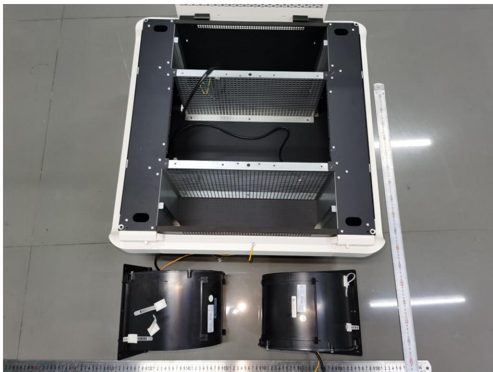
Figure 18: Internal view of SCA14000-2x2
