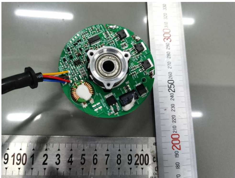
Figure 24: Motor of SCA14000-2x2
