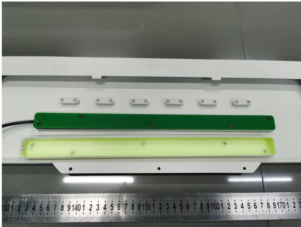
Figure 35: Internal view of SCA14000-2x4
