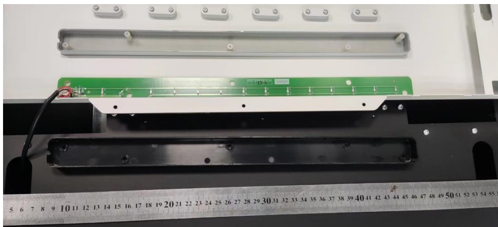
Figure 36: Internal view of SCA14000-2x4
