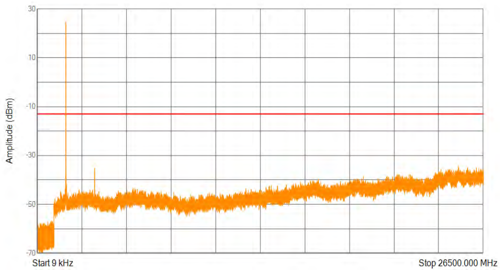
Band4 QPSK BW=15MHz Channel=20025 RB Size=1 Position=#0 NB Index=0
