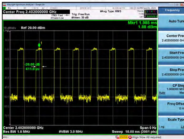
8-DPSK 3DH1 2402MHZ
