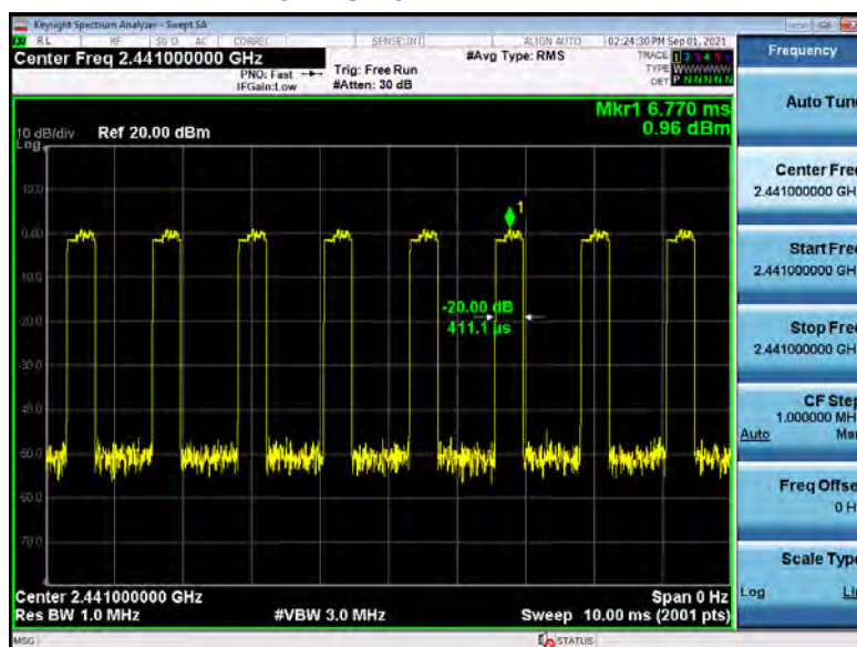
8-DPSK 3DH1 2441MHZ
