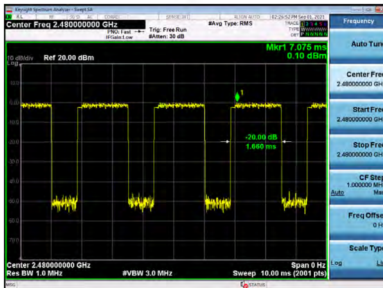
8-DPSK 3DH3 2480MHZ
