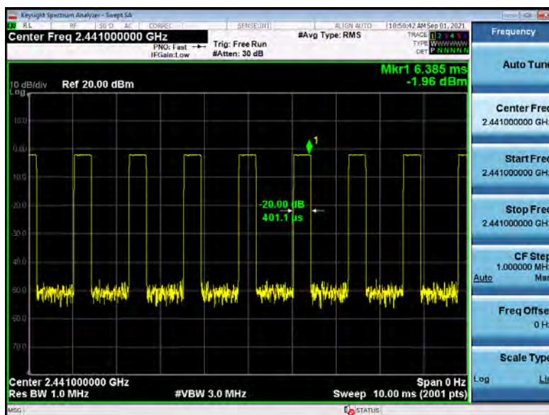
GFSK DH1 2441MHZ
