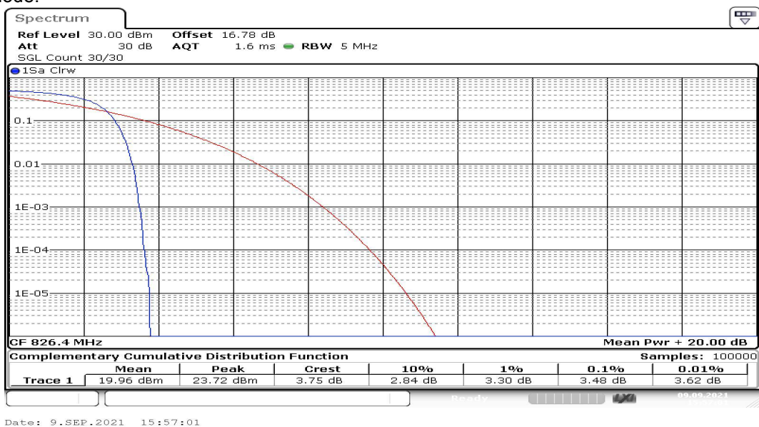
Channel 4132
