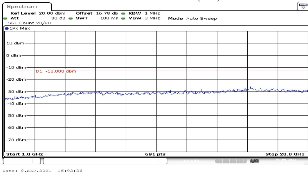
Channel 4183 1GHz~20GHz(dBm)
