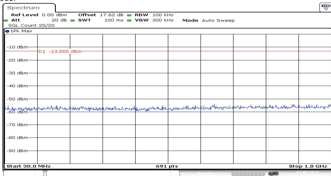
Channel 9400 30MHz~1GHz(dBm)
