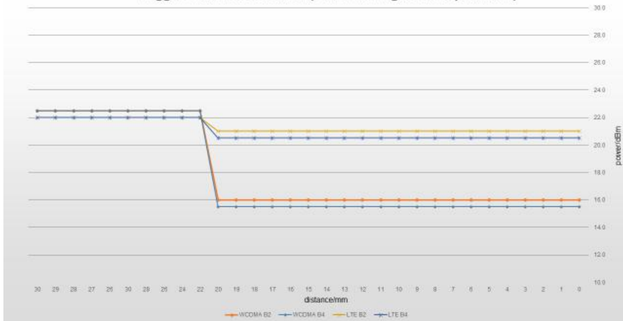
Trigger distance evaluation (Front moving towards phantom )
