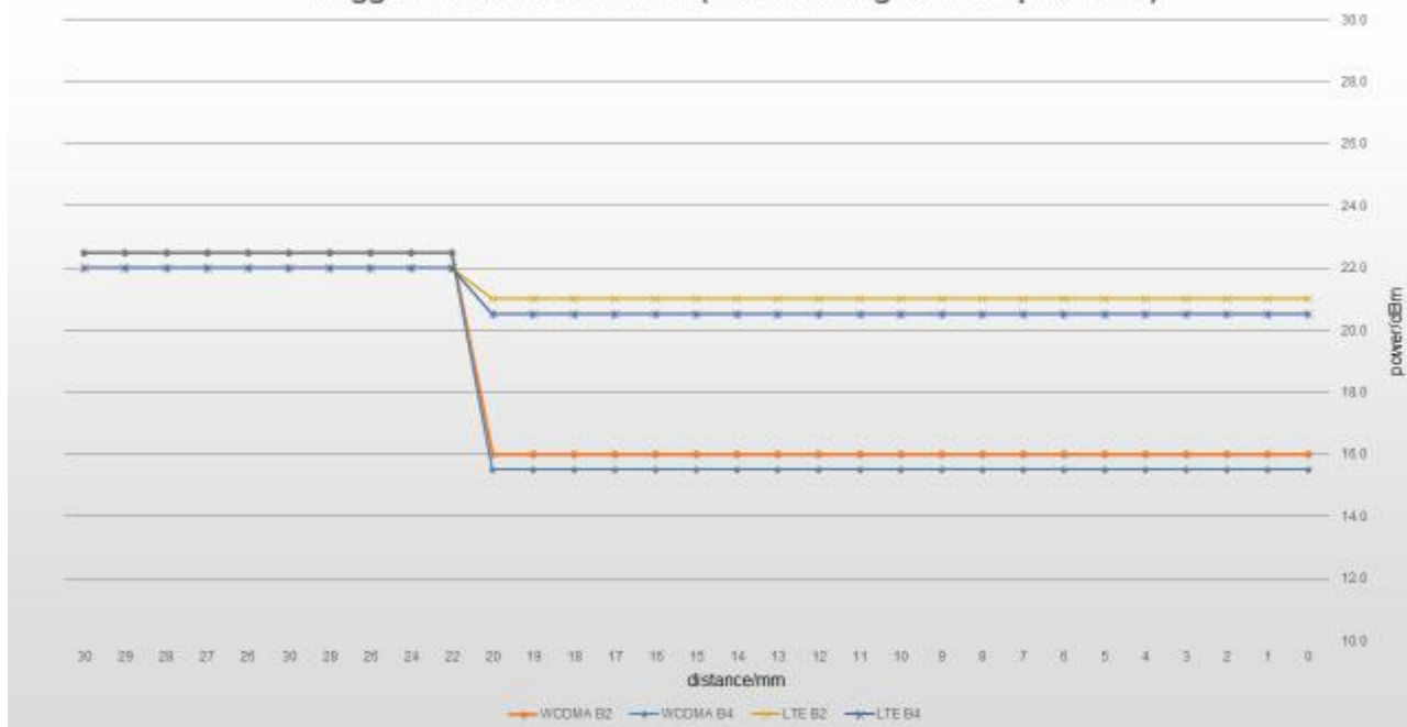
Trigger distance evaluation (back moving towards phantom )
