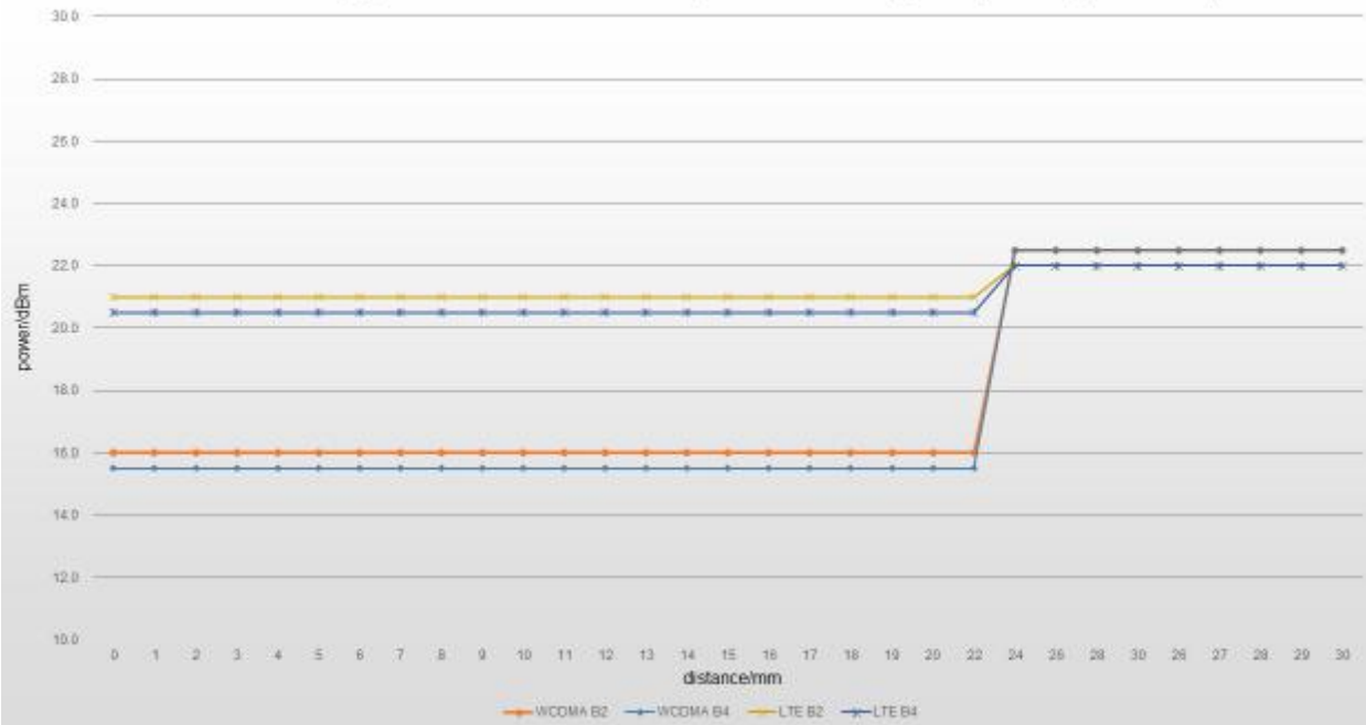
Trigger distance evaluation (bottom moving away from phantom)
