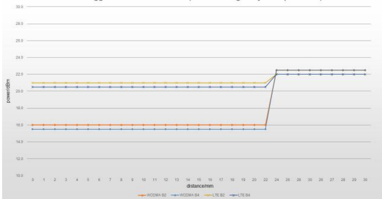
Trigger distance evaluation (back moving away from phantom )
