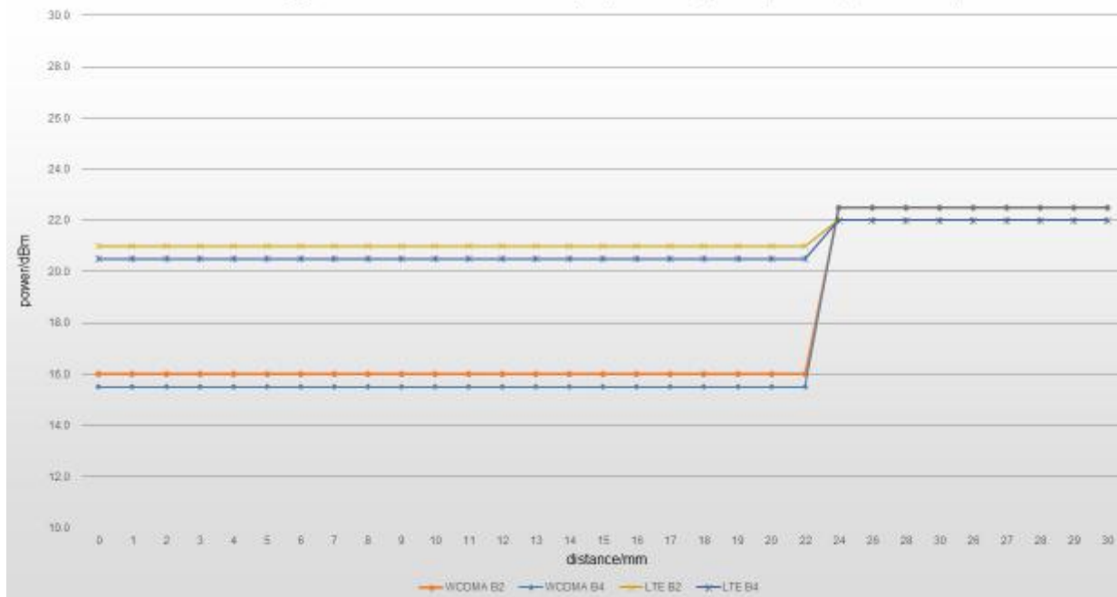
Trigger distance evaluation (top moving away from phantom )
