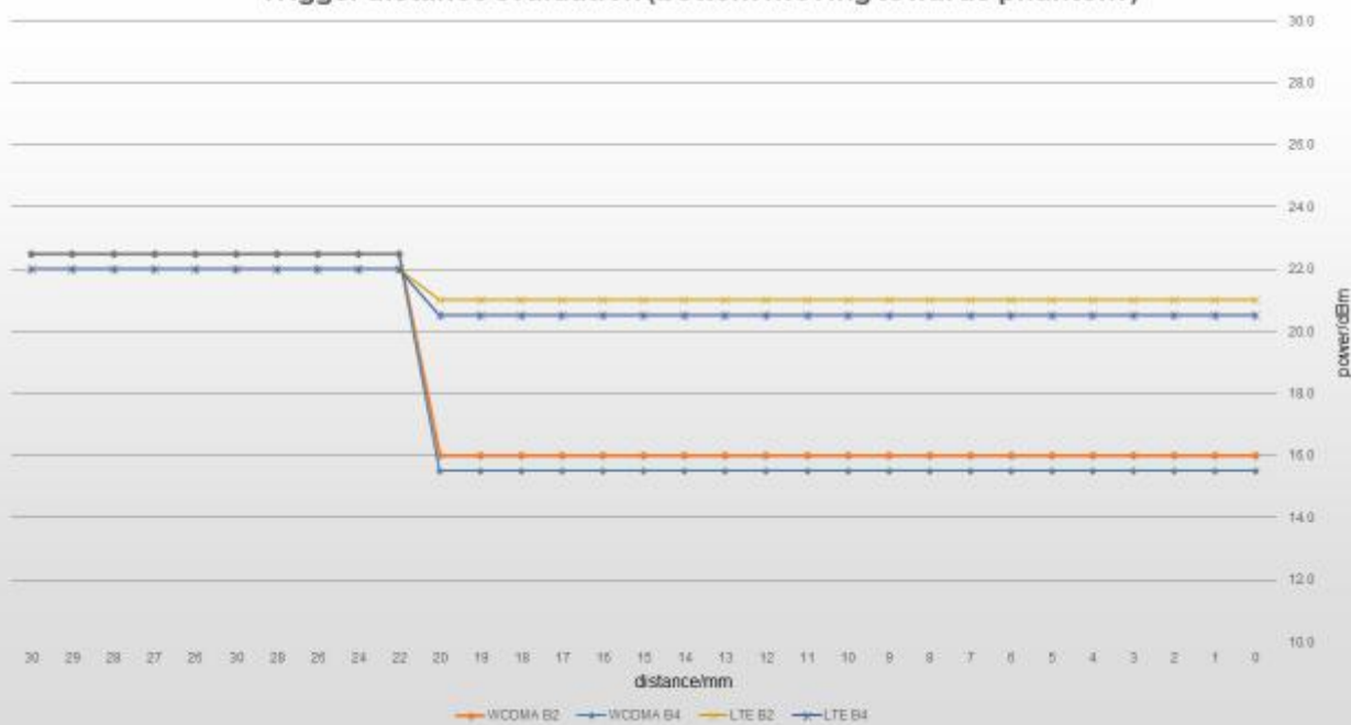
Trigger distance evaluation (bottom moving towards phantom )
