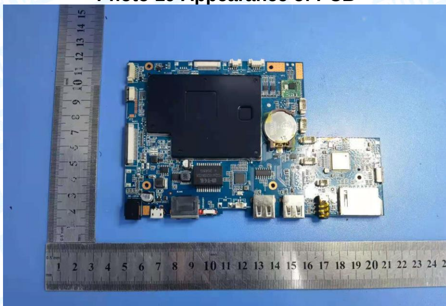
Photo 20 Appearance of PCB
