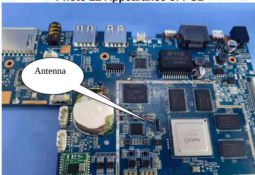
Photo 22 Appearance of PCB
