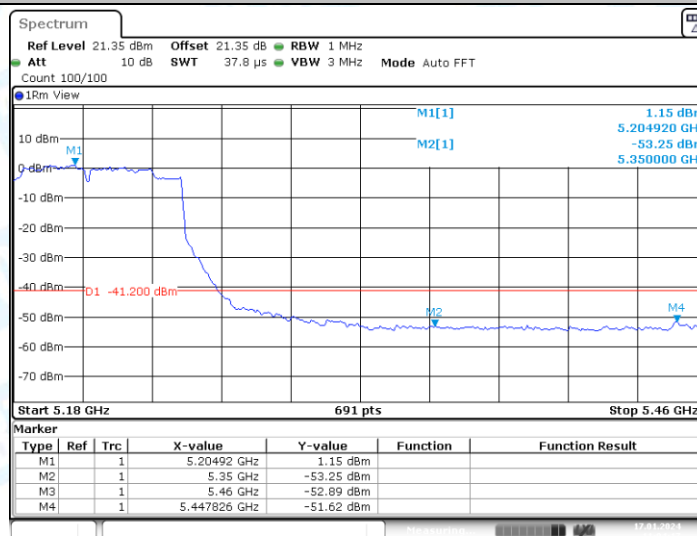
11AC80MIMO_Ant1_High_5210_AV
