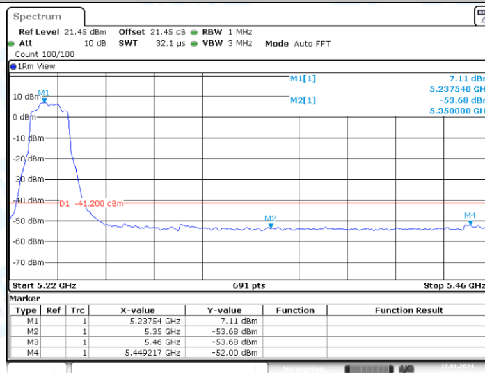
11AX20MIMO_Ant1_High_5240_AV
