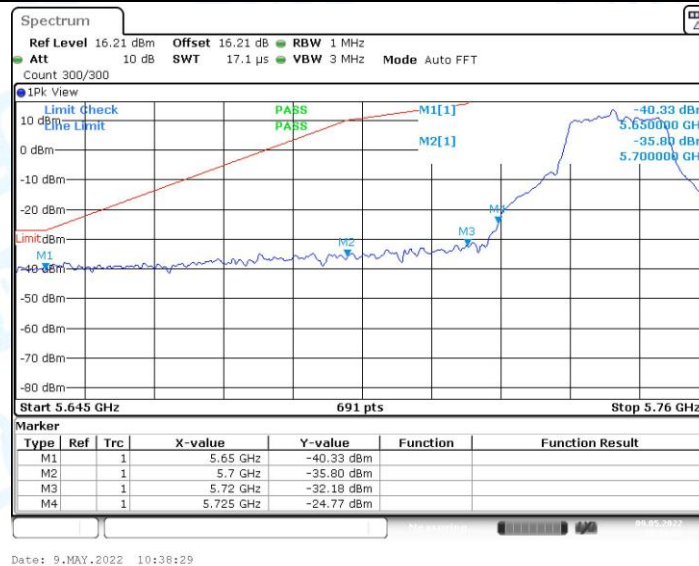
11AMIMO_Ant1_Low_5745_Peak
