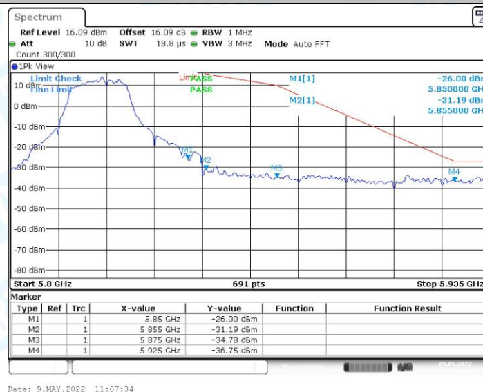
11AMIMO_Ant1_High_5825_Peak
