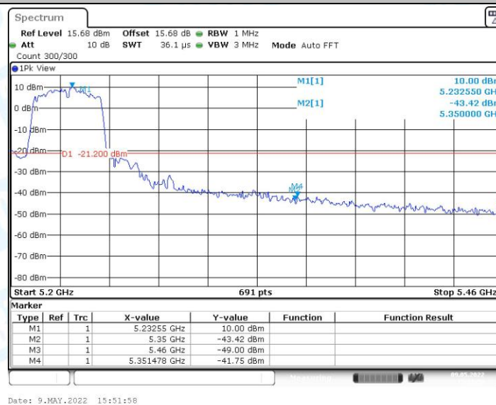
11N40MIMO_Ant0_High_5230_Peak
