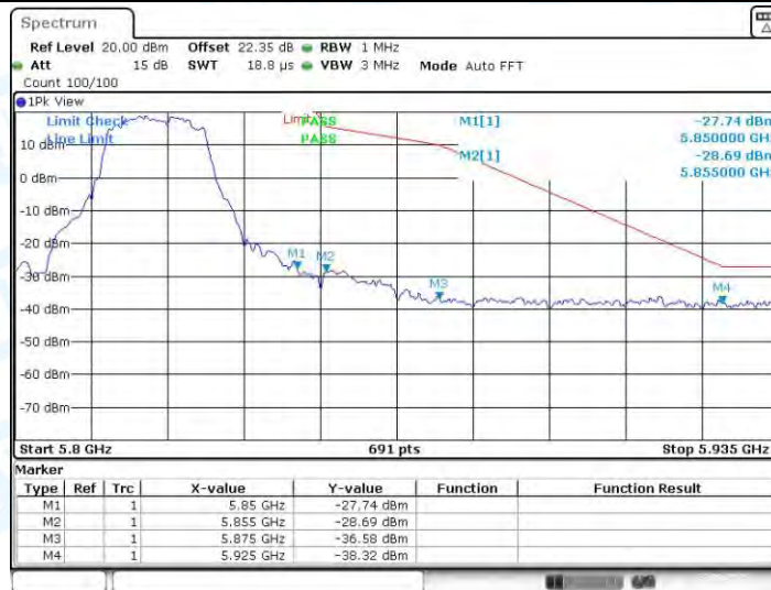
11N20MIMO_Ant2_High_5825_Peak
