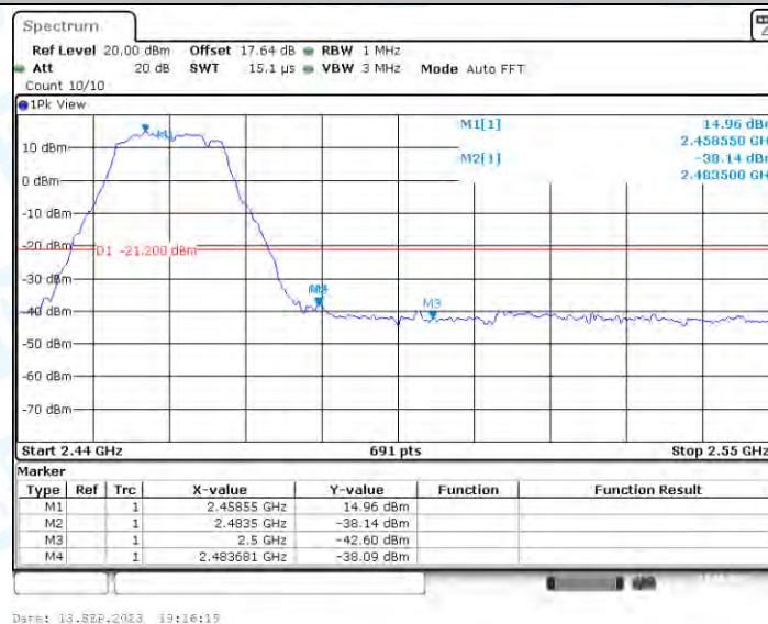
11G-CDD_Ant2_High_2462_AV
