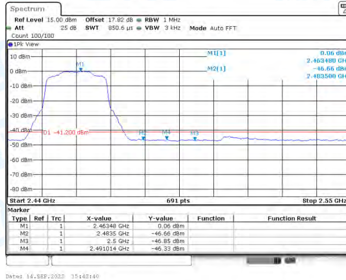
11AX20MIMO_Ant2_High_2462_Peak
