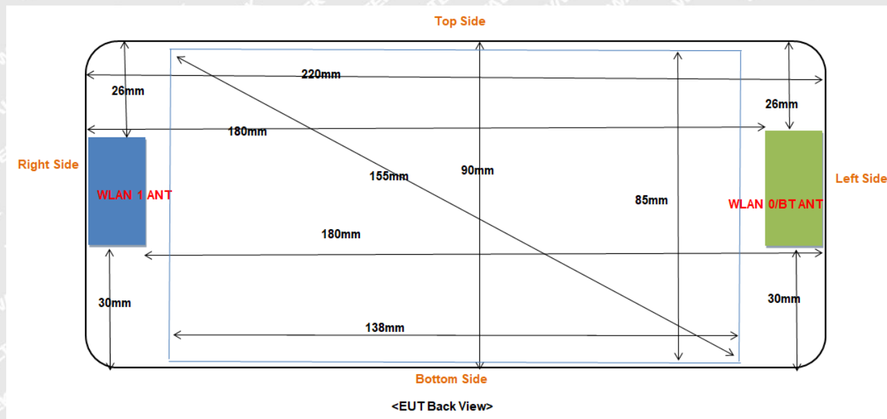
Fig 7.1 Block Diagram for EUT Antenna Position
