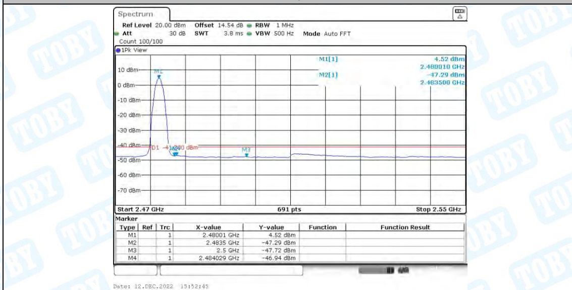
3DH5_Ant1_High_2480_Peak
